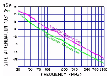
Figure 2-4. Normalized Site Attenuation Curves (H&V)
