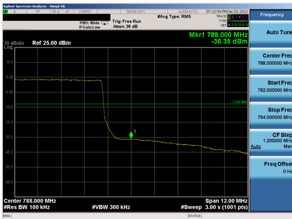
Plot 7-7. Upper Band Edge Plot (10.0MHz QPSK – RB Size 50)
