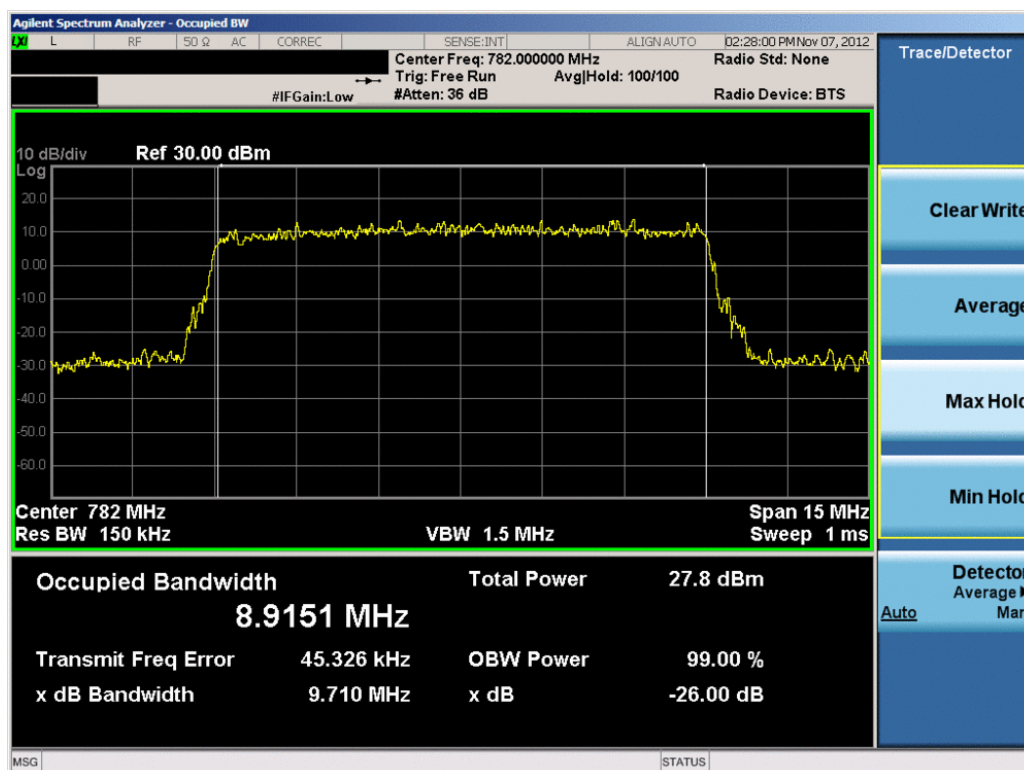
Plot 7-4. Occupied Bandwidth Plot (10.0MHz 16-QAM – RB Size 50)
