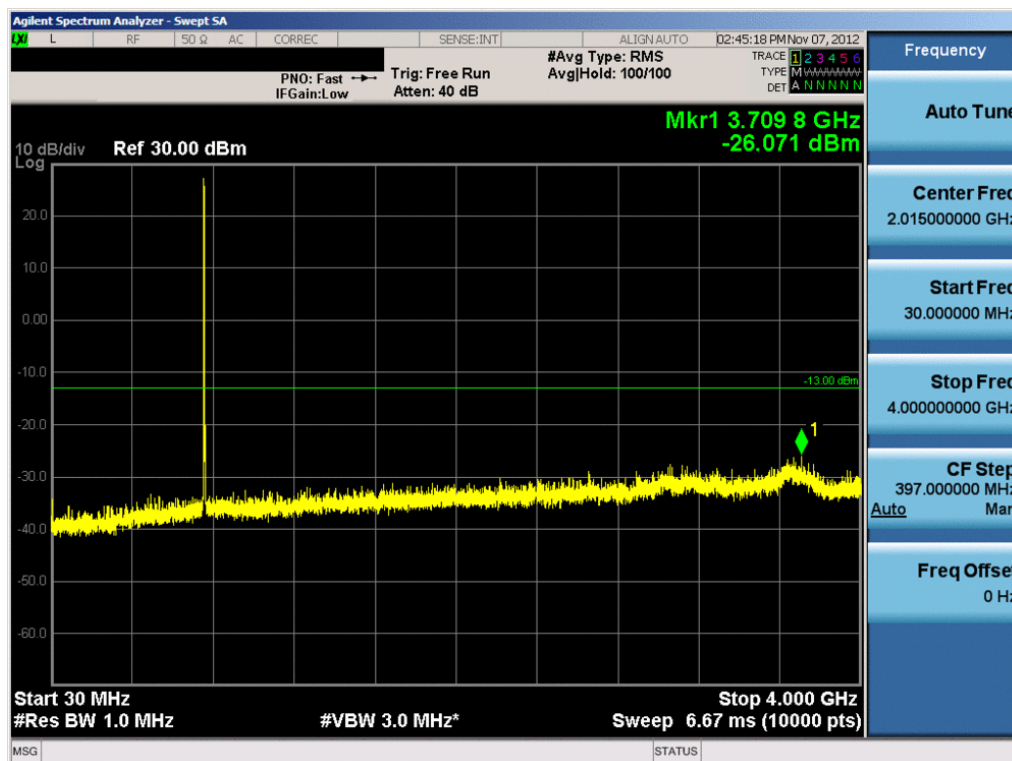
Plot 7-5. Conducted Spurious Plot (10.0MHz QPSK – RB Size 1, RB Offset 0)
