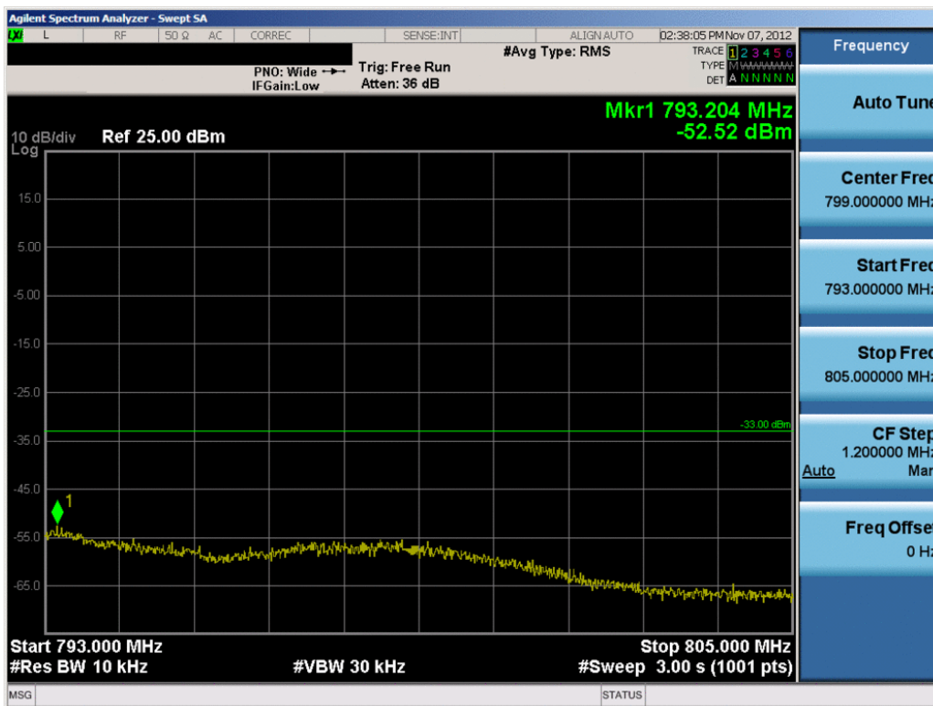
Plot 7-8. Upper Extended Band Edge Plot (10.0MHz QPSK – RB Size 50)
