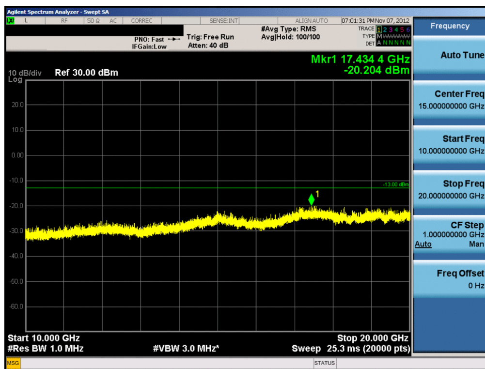
Plot 8-36. Conducted Spurious Plot (15.0MHz QPSK – RB Size 1, RB Offset 0 – Mid Channel)
