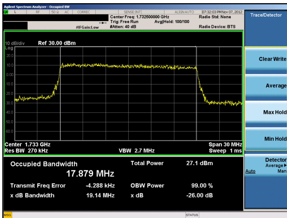
Plot 8-46. Occupied Bandwidth Plot (20.0MHz 16-QAM – RB Size 100)
