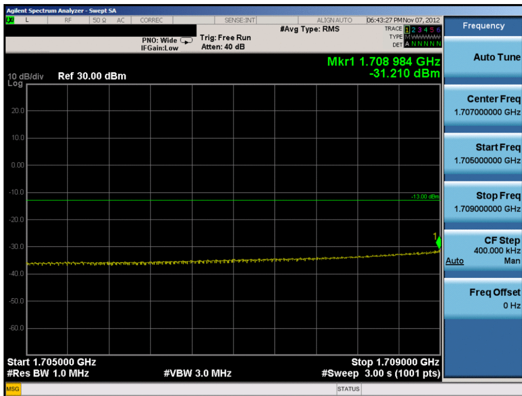
Plot 8-30. Lower Extended Band Edge Plot (15.0MHz QPSK – RB Size 75)
