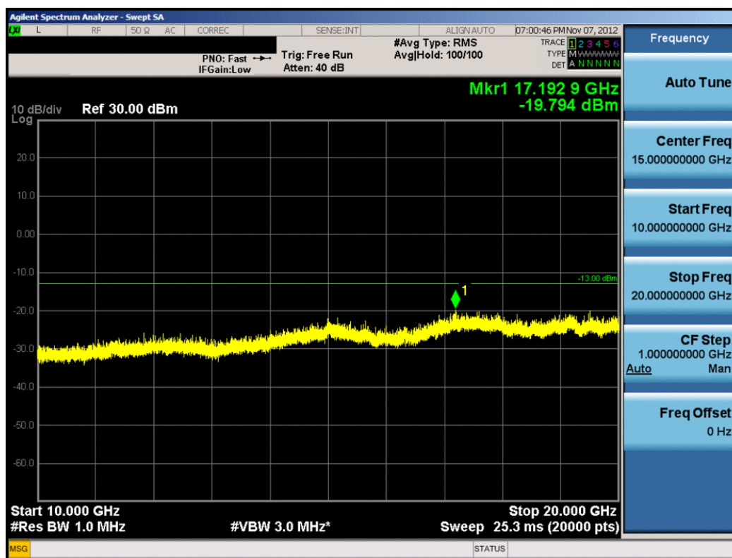
Plot 8-38. Conducted Spurious Plot (15.0MHz QPSK – RB Size 1, RB Offset 0 – High Channel)
