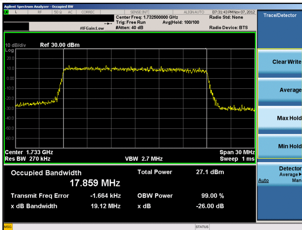
Plot 8-45. Occupied Bandwidth Plot (20.0MHz QPSK – RB Size 100)
