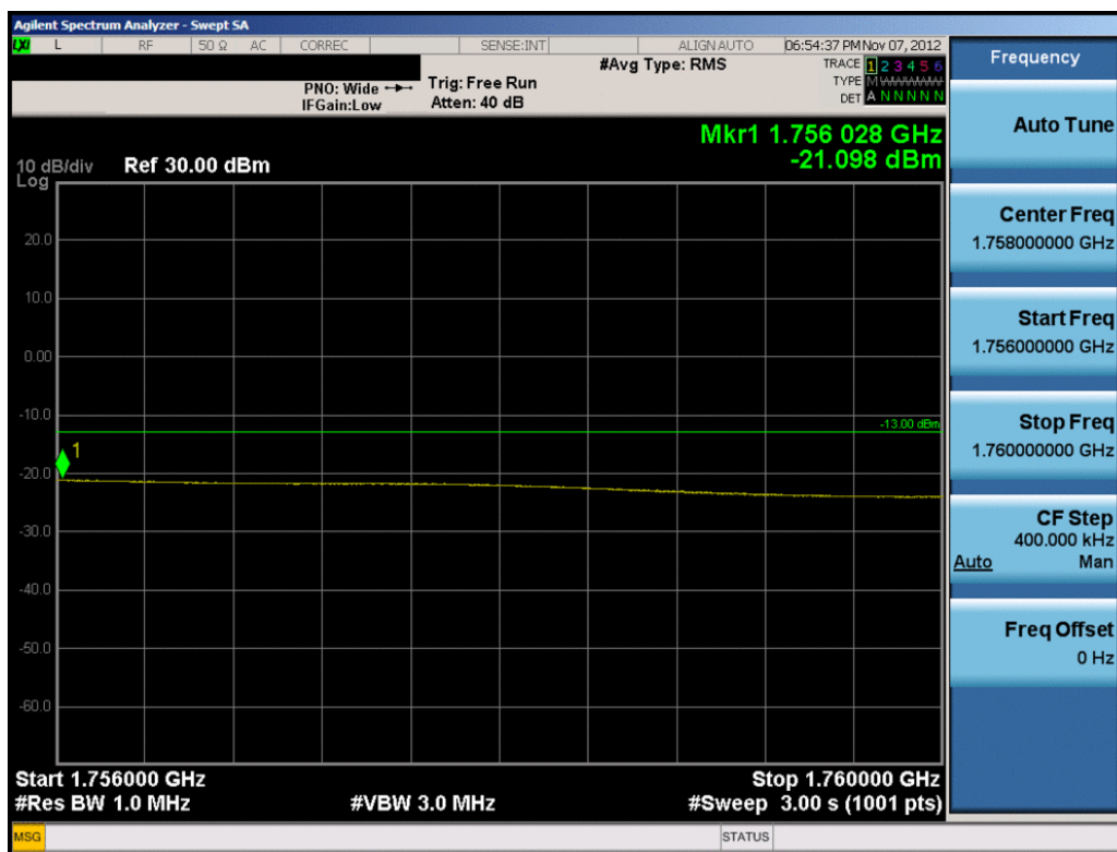
Plot 8-40. Upper Extended Band Edge Plot (15.0MHz QPSK – RB Size 75)
