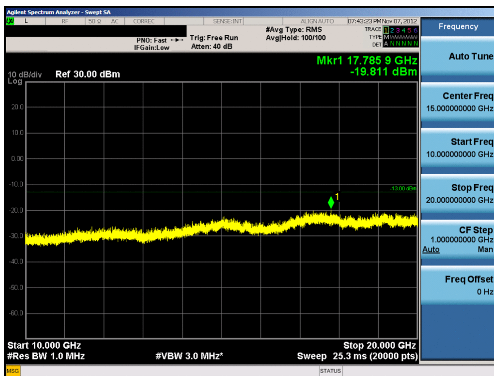
Plot 8-52. Conducted Spurious Plot (20.0MHz QPSK – RB Size 1, RB Offset 0 – High Channel)
