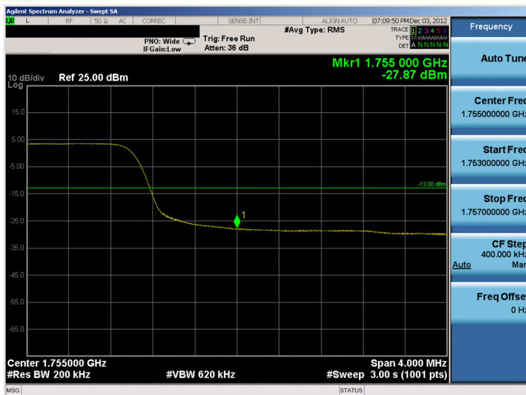
Plot 8-53. Upper Band Edge Plot (20.0MHz QPSK – RB Size 100)
