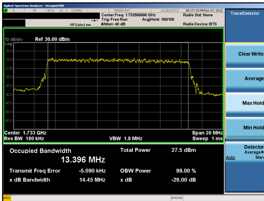
Plot 8-31. Occupied Bandwidth Plot (15.0MHz QPSK – RB Size 75)
