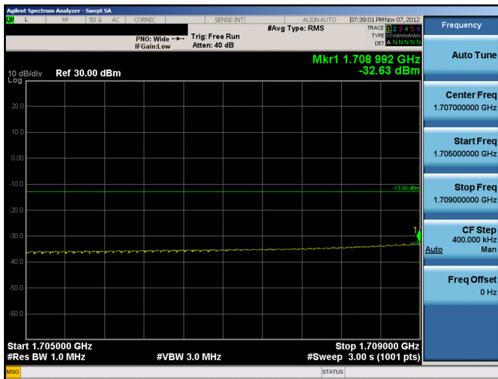
Plot 8-44. Lower Extended Band Edge Plot (20.0MHz QPSK – RB Size 100)
