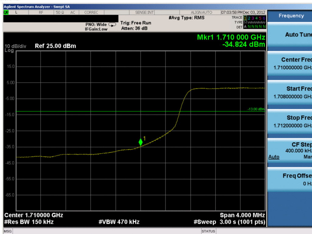
Plot 8-29. Lower Band Edge Plot (15.0MHz QPSK – RB Size 75)
