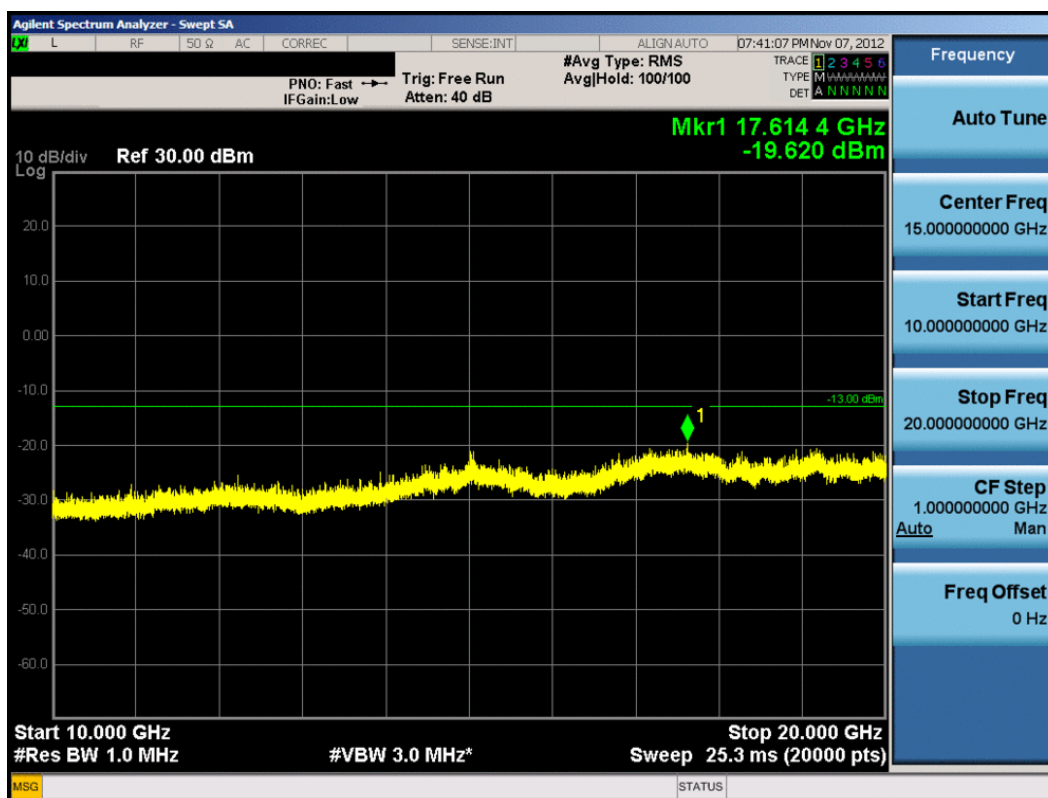
Plot 8-50. Conducted Spurious Plot (20.0MHz QPSK – RB Size 1, RB Offset 0 – Mid Channel)
