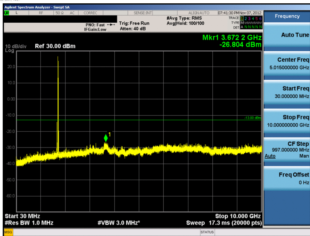
Plot 8-49. Conducted Spurious Plot (20.0MHz QPSK – RB Size 1, RB Offset 0 – Mid Channel)
