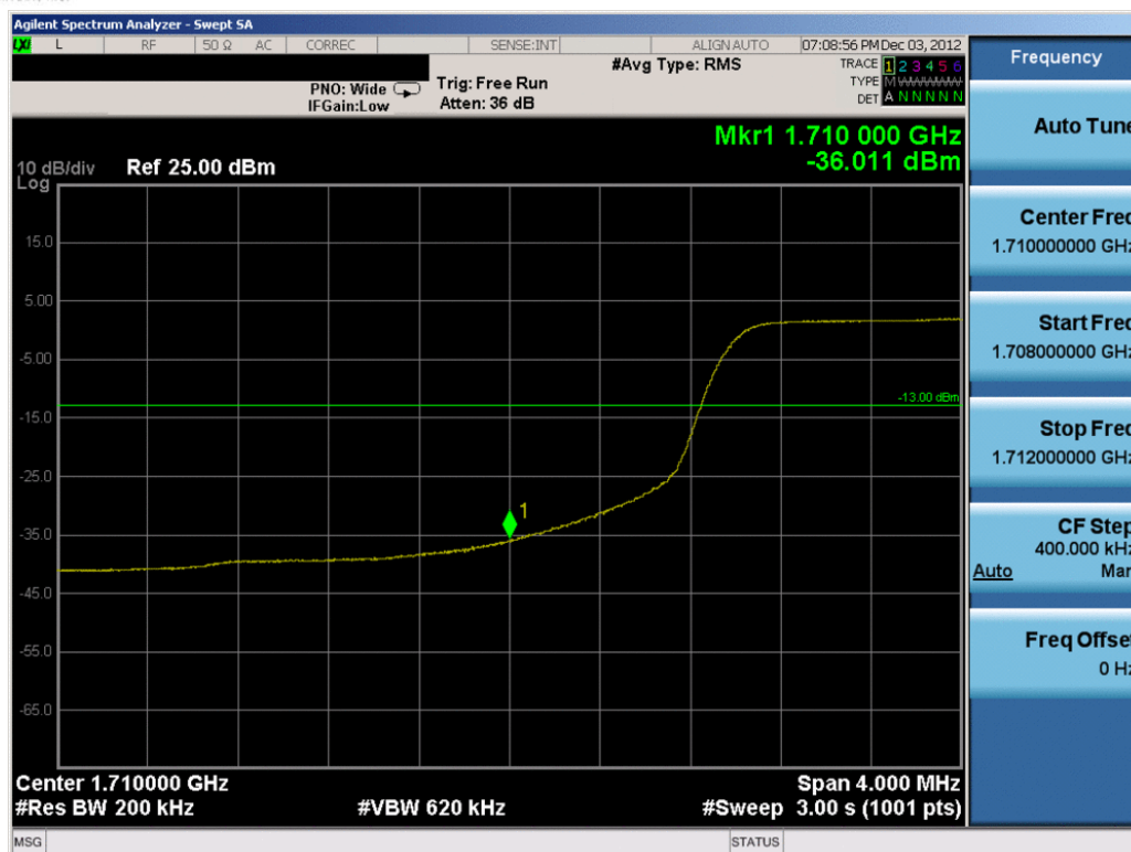
Plot 8-43. Lower Band Edge Plot (20.0MHz QPSK – RB Size 100)
