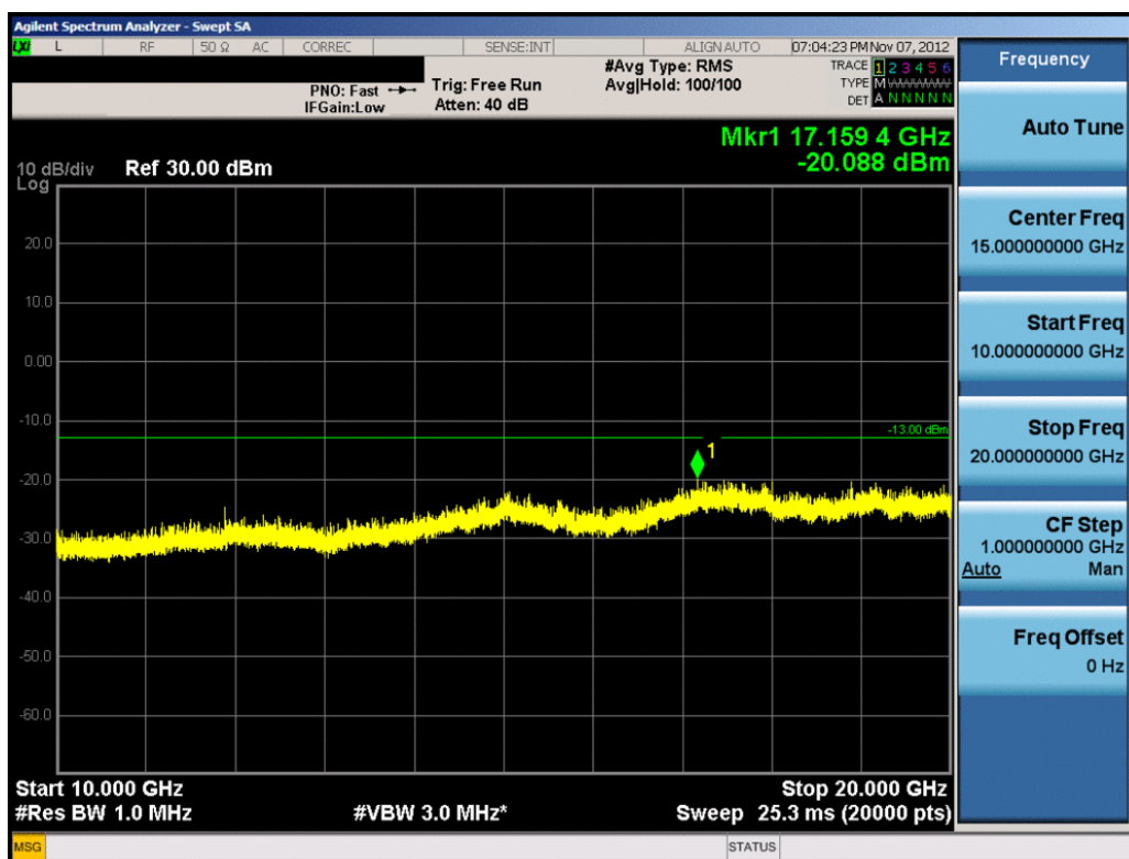
Plot 8-34. Conducted Spurious Plot (15.0MHz QPSK – RB Size 1, RB Offset 0 – Low Channel)
