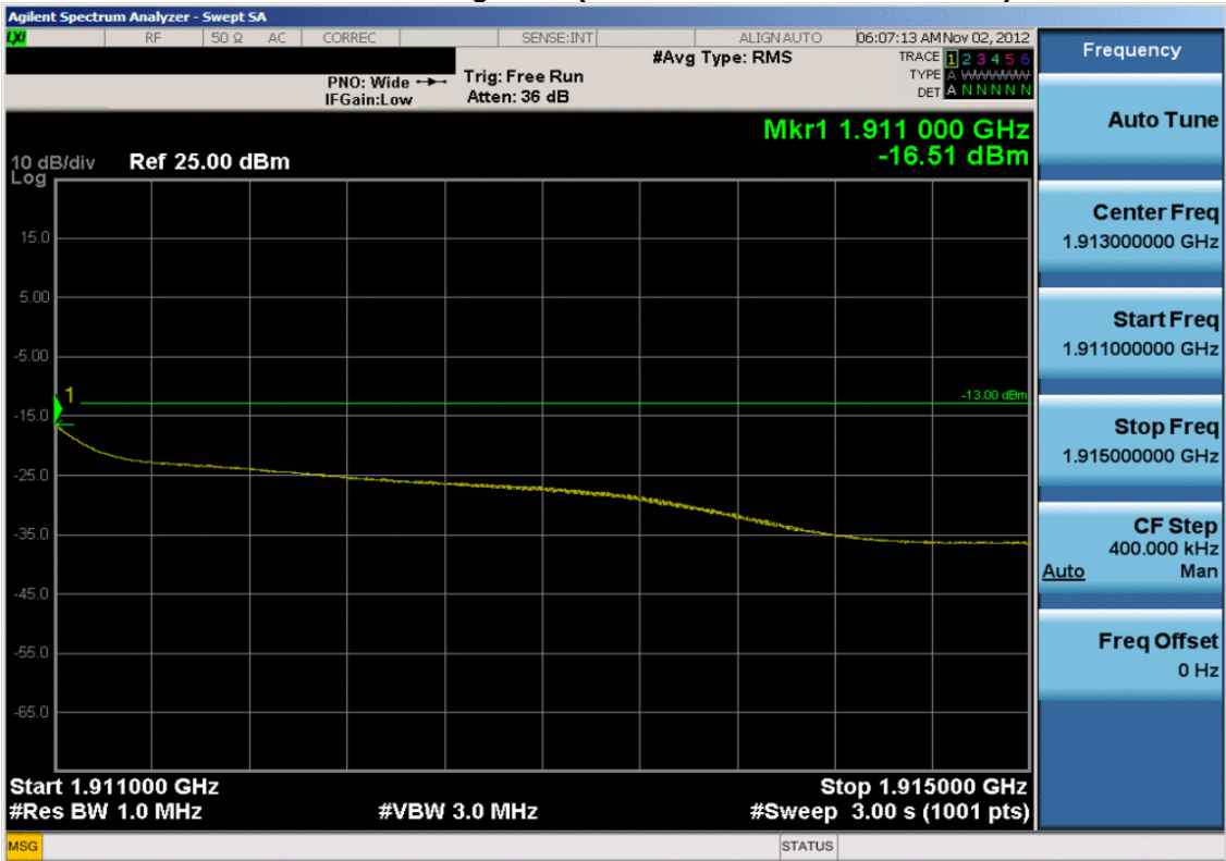
Plot 7-68. 4MHz Span Plot (PCS WCDMA Mode – Ch. 9538)
