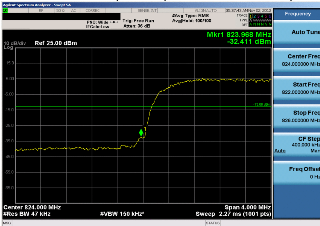
Plot 7-48. Band Edge Plot (Cellular WCDMA Mode – Ch. 4132)
