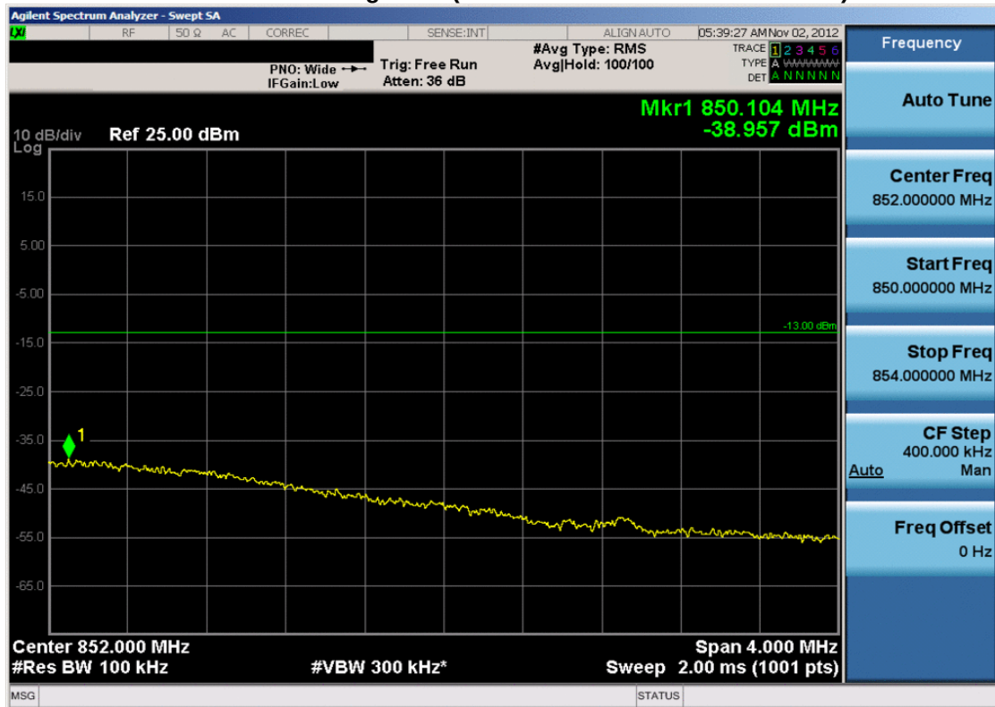
Plot 7-56. 4MHz Span Plot (Cellular WCDMA Mode – Ch. 4233)
