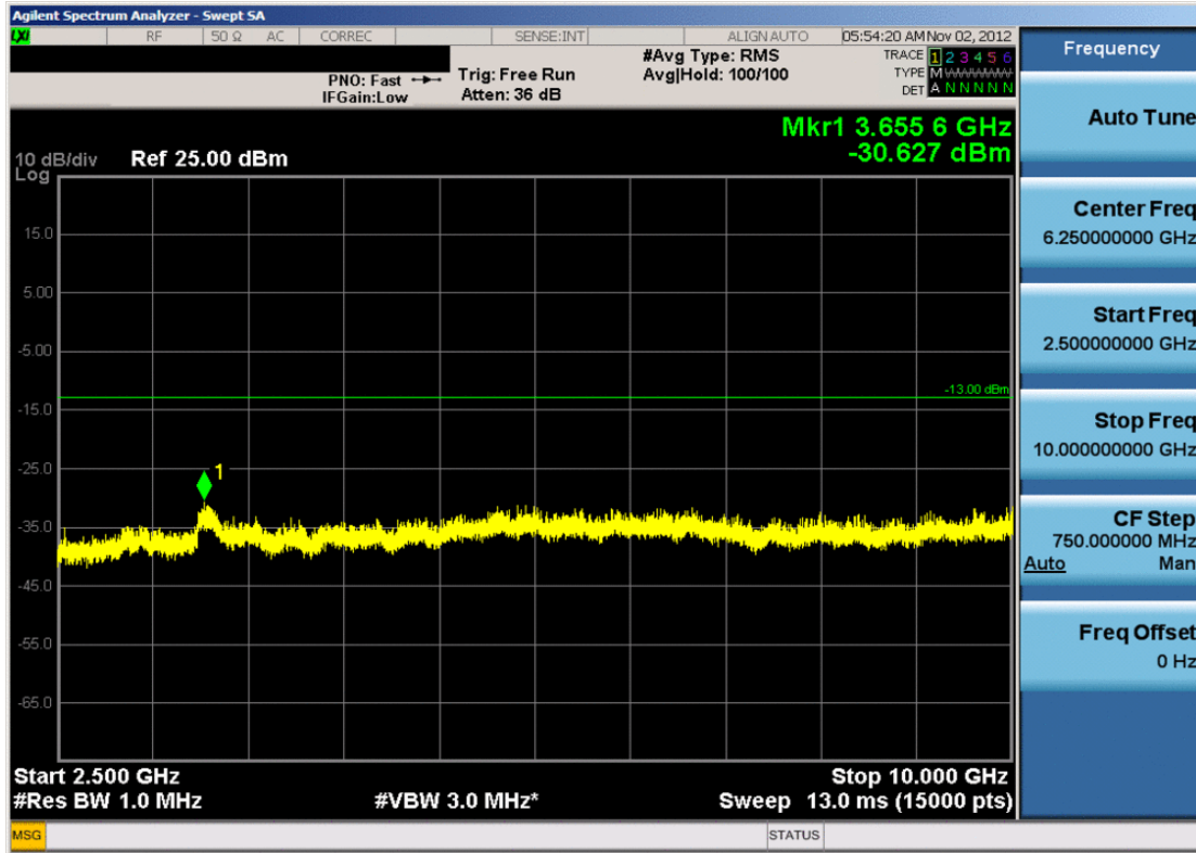
Plot 7-47. Conducted Spurious Plot (Cellular WCDMA Mode – Ch. 4132)
