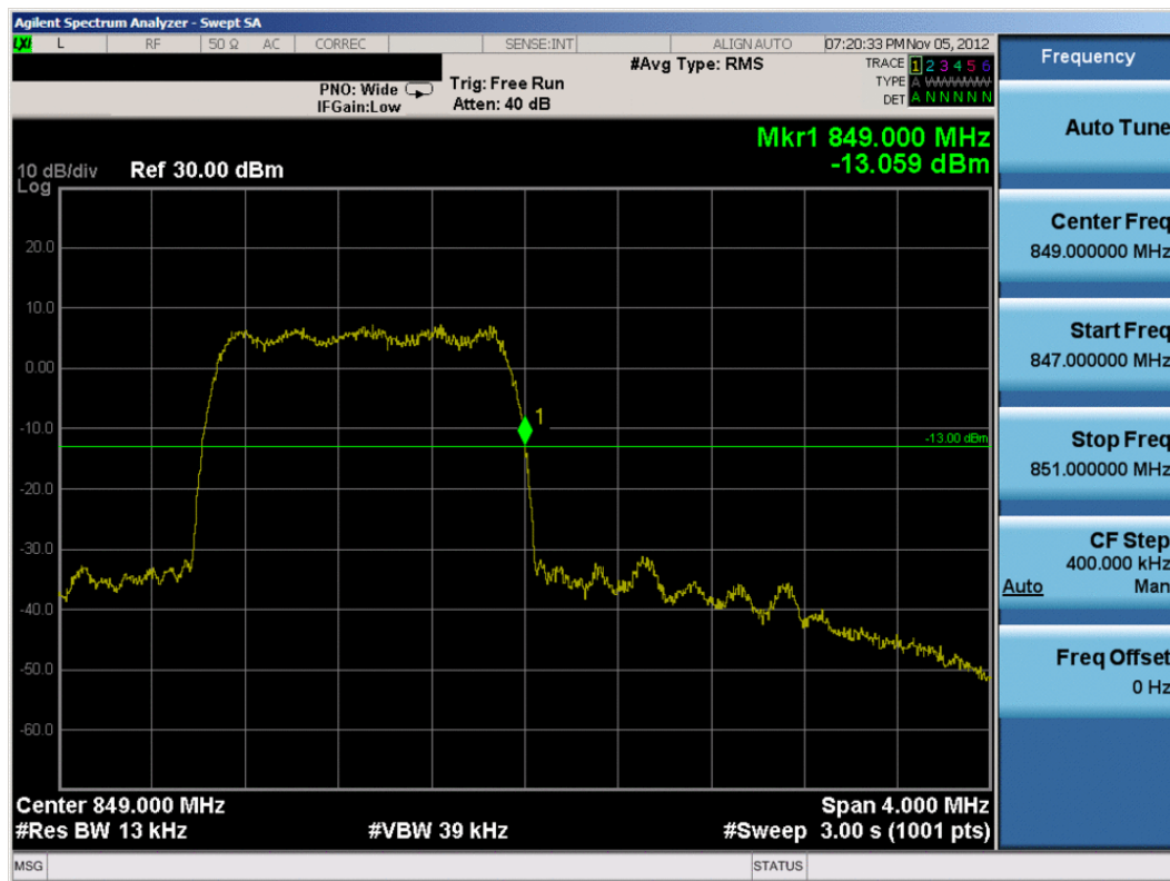
Plot 7-32. Band Edge Plot (Cellular CDMA Mode – Ch. 777)
