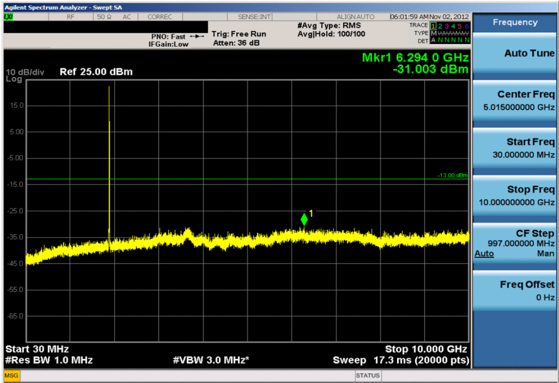
Plot 7-65. Conducted Spurious Plot (PCS WCDMA Mode – Ch. 9538)
