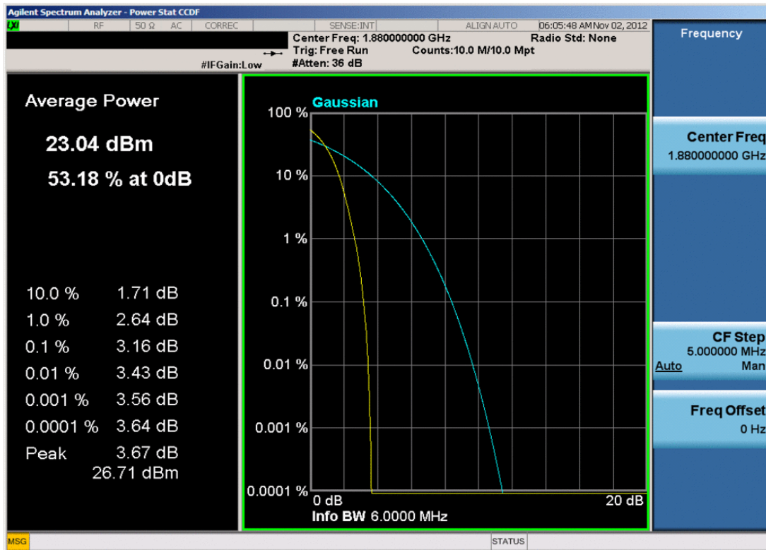
Plot 7-64. Peak-Average Ratio Plot (PCS WCDMA Mode – Ch. 9400)
