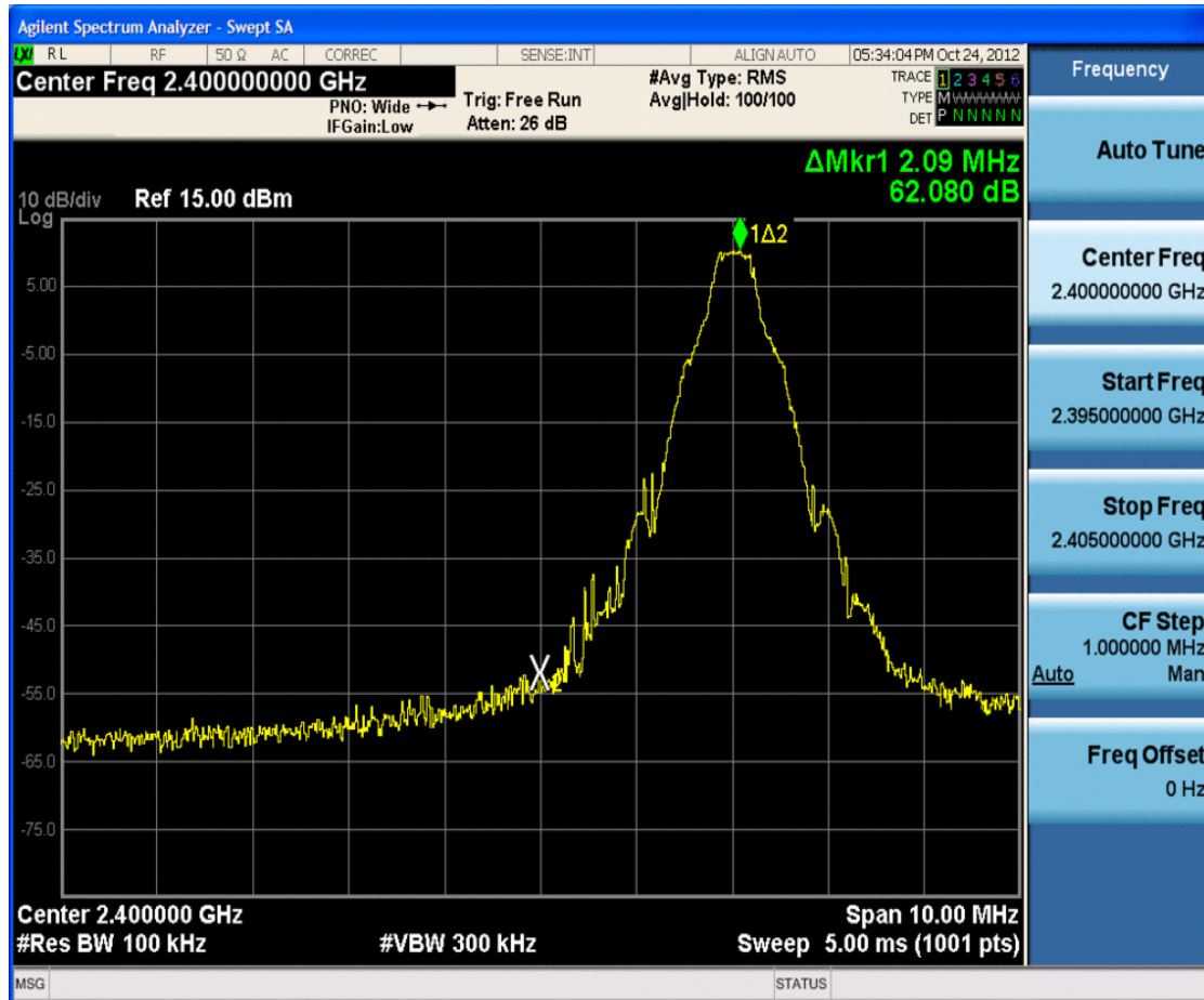
Plot 6-28. Band Edge Plot (Bluetooth with Hopping Disabled, 1Mbps – Ch. 0)
