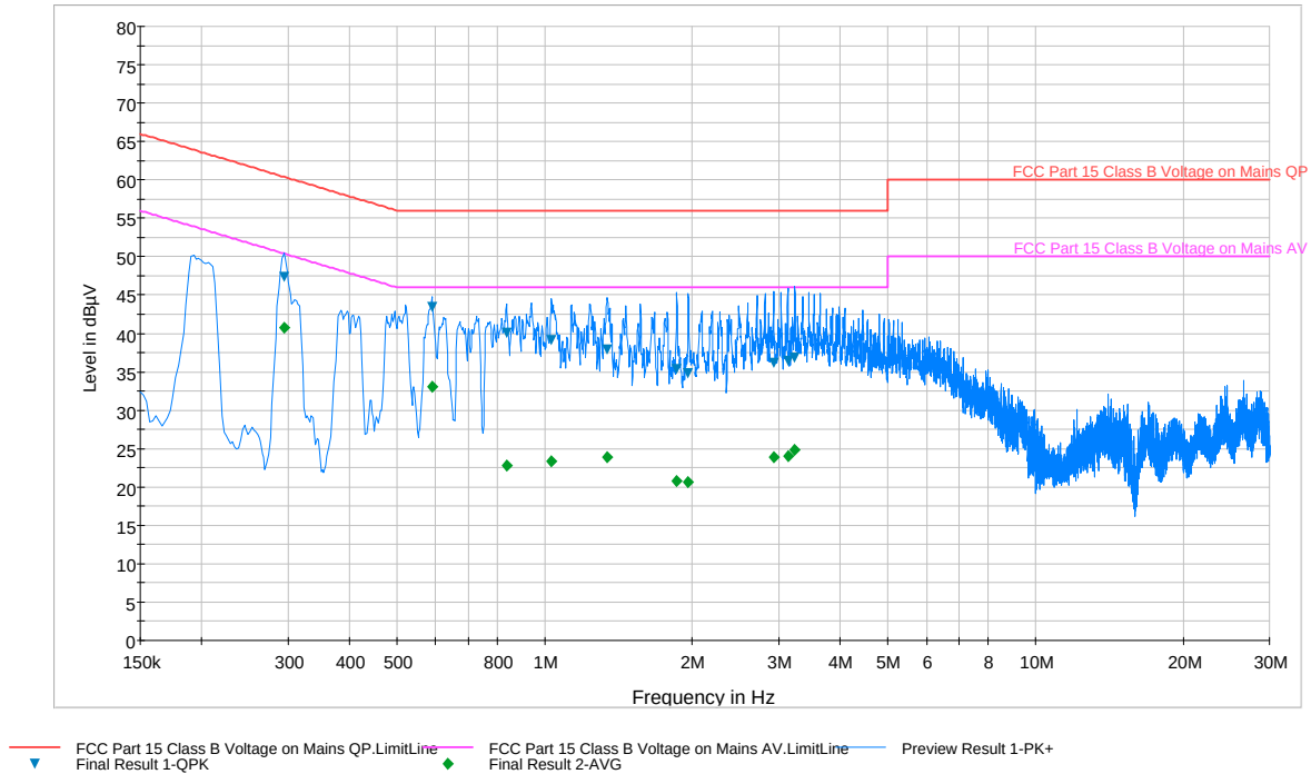
Plot 6-56. Line Conducted Plot with 802.11a UNII Band 2 (L1)
