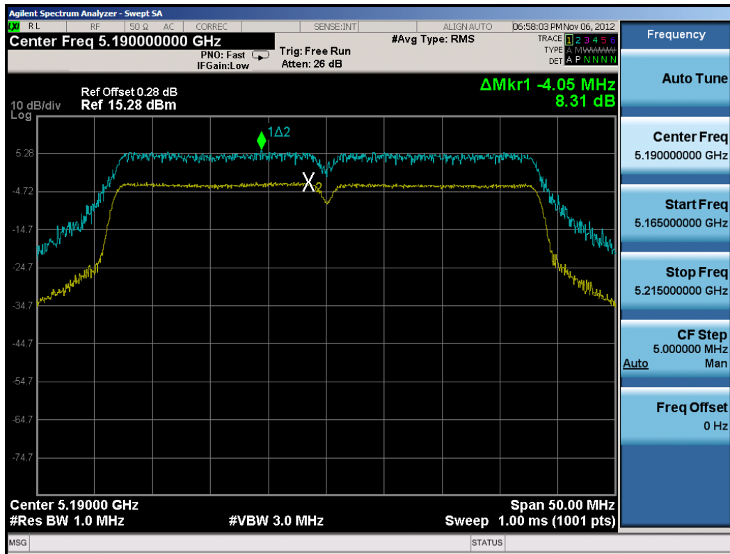
Plot 6-53. Peak Excursion Ratio Plot (40MHz BW 802.11n (UNII Band 1) – Ch. 38)
