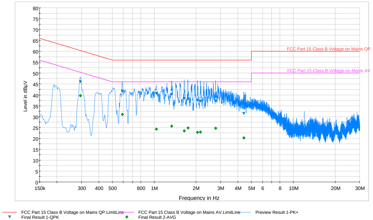
Plot 6-54. Line Conducted Plot with 802.11a UNII Band 1 (L1)
