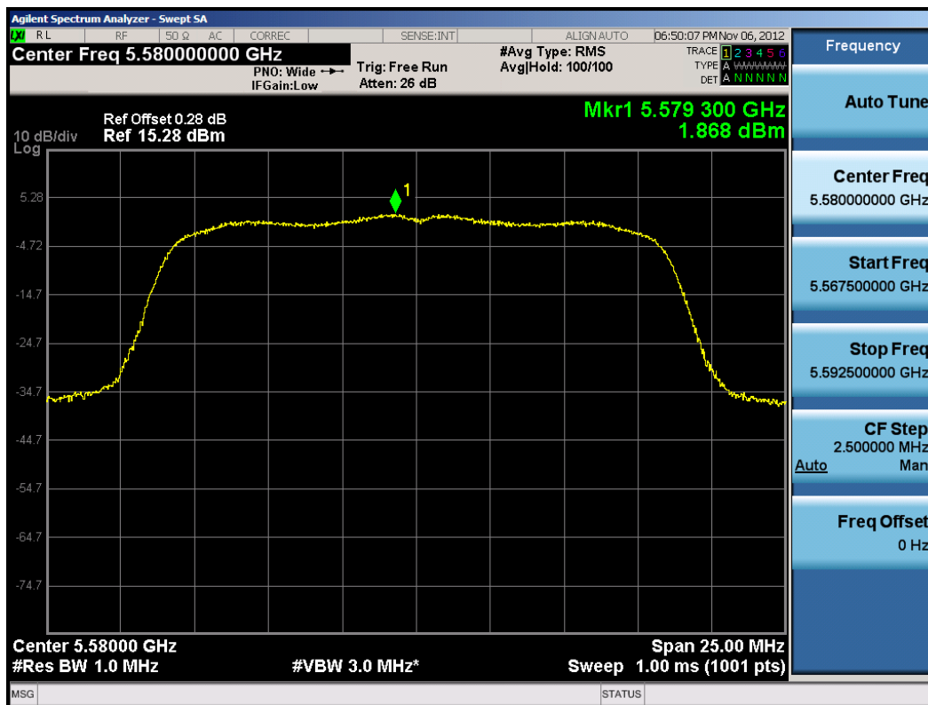
Plot 6-43. Peak Power Spectral Density Plot (802.11a (UNII Band 3) – Ch. 116)
