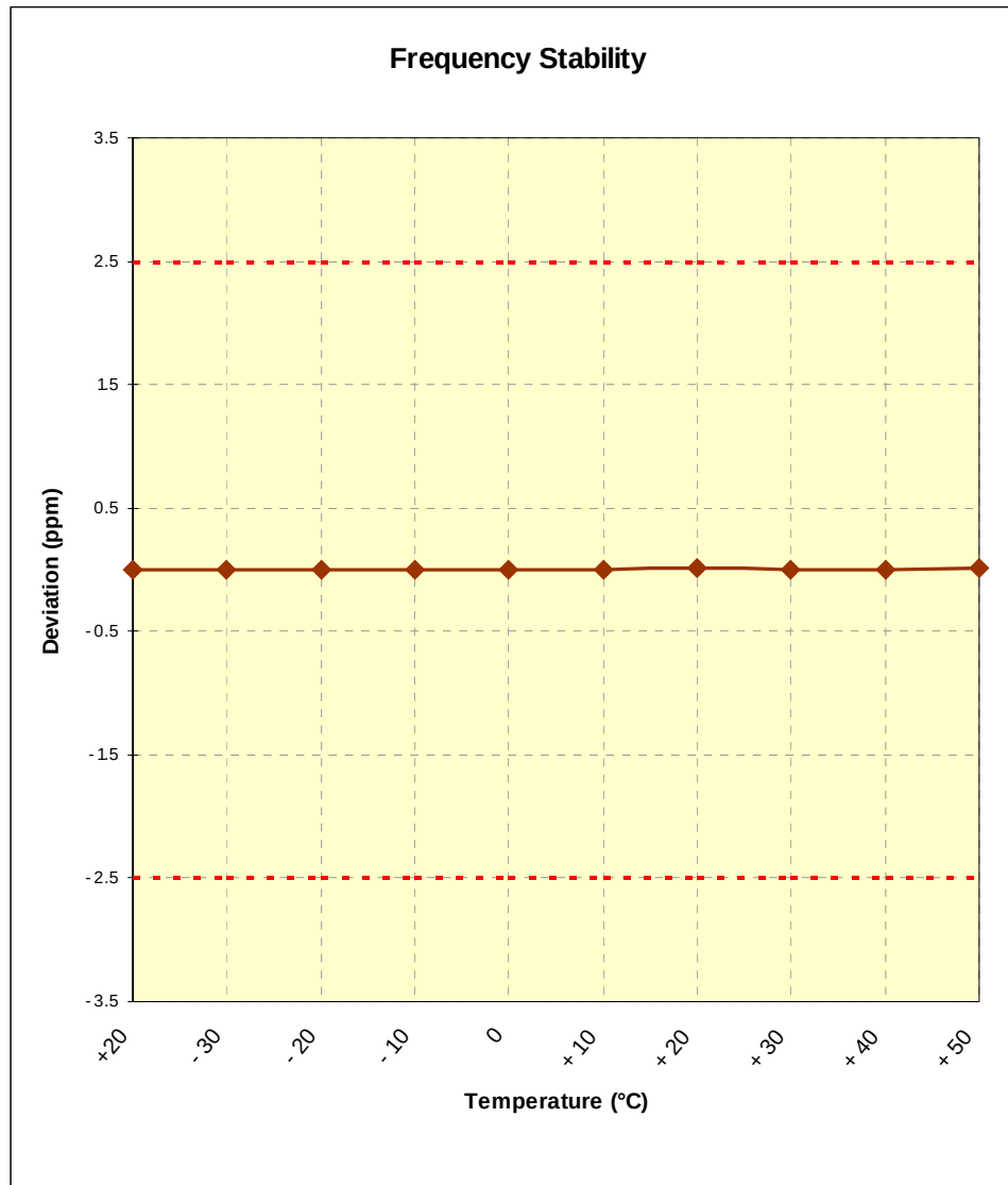
Figure 6-3. Frequency Stability Graph (PCS CDMA Mode – Ch. 600)
