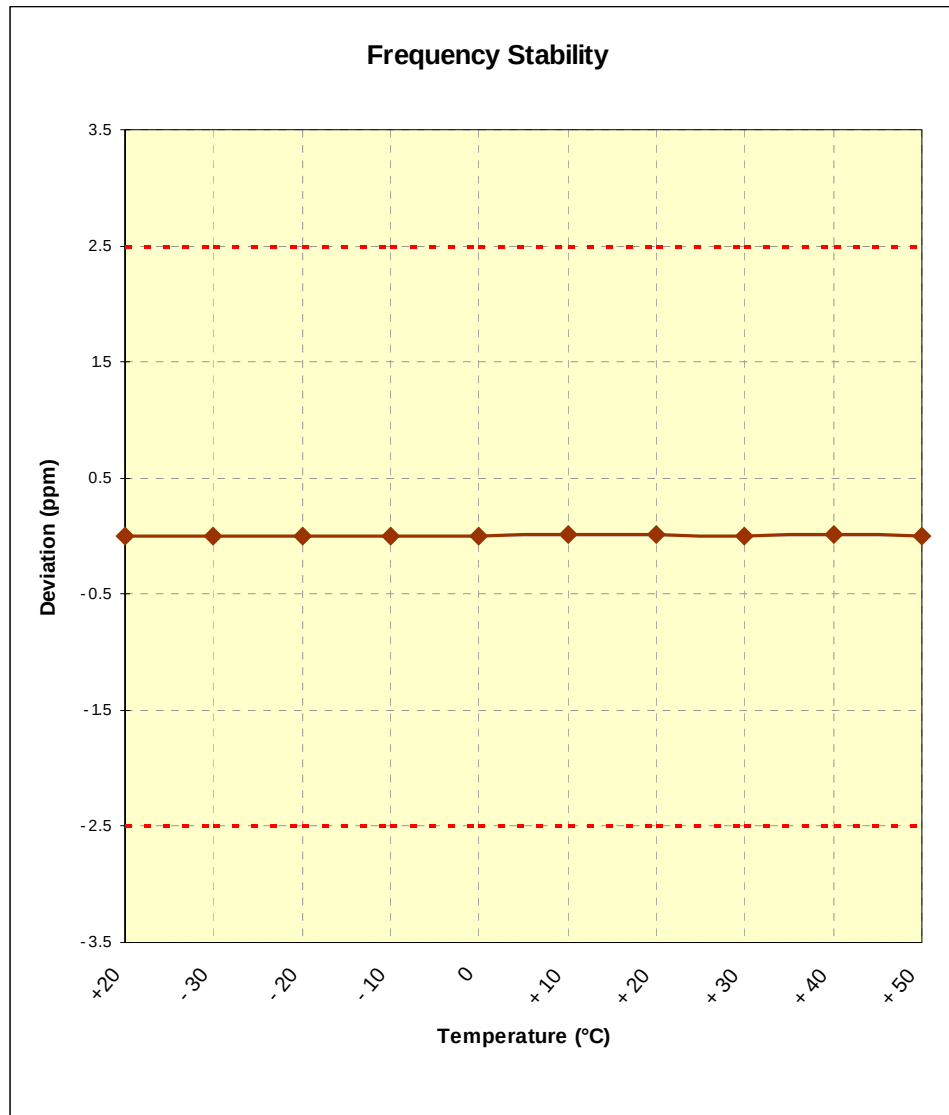
Figure 6-2. Frequency Stability Graph (AWS CDMA Mode – Ch. 450)
