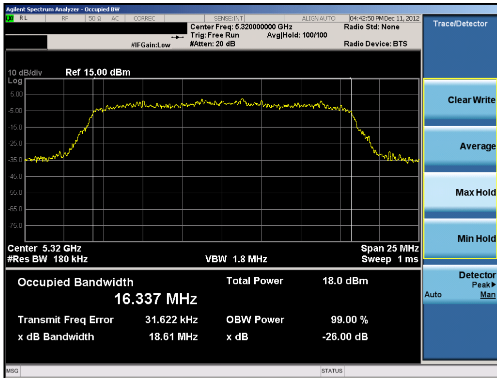
Plot 6-11. 26dB Bandwidth Plot (802.11a (UNII Band 2) – Ch. 64)
