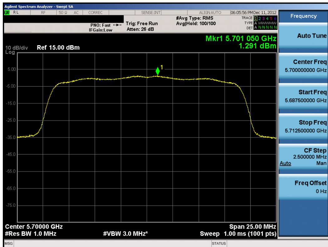
Plot 6-47. Peak Power Spectral Density Plot (20MHz BW 802.11a/n (UNII Band 3) – Ch. 140)
