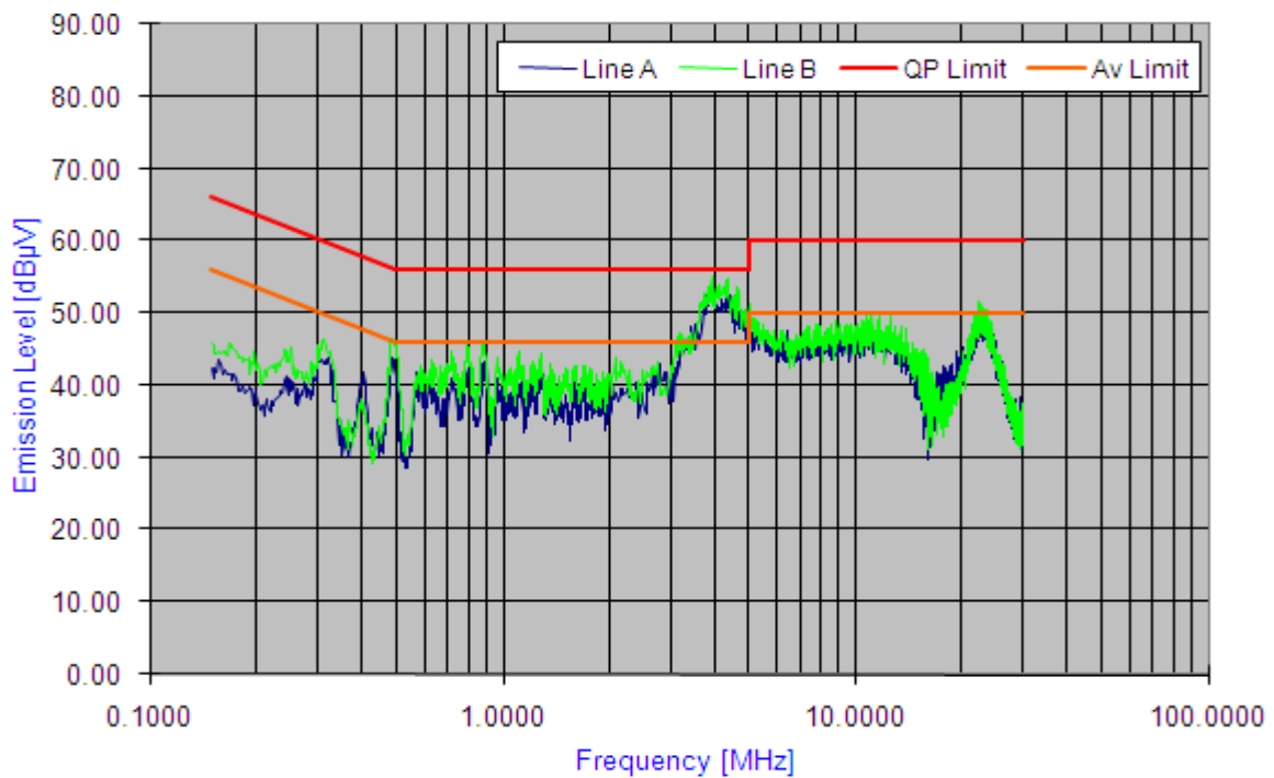
Plot 6-57. Line Conducted Plot with 802.11n (5.8GHz)
