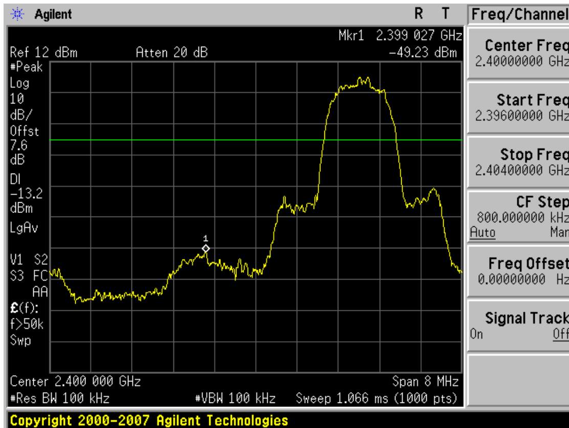
Plot 6-10. Band Edge Plot (Bluetooth, 3Mbps – Ch. 0)
