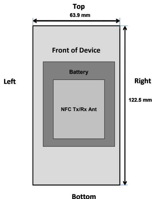
Figure 1-1 NFC Antenna Locations
