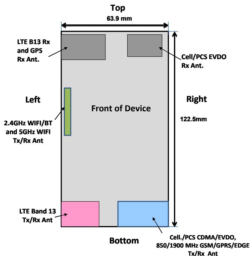
Figure 1-2 EUT Antenna Locations
