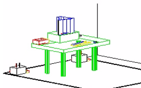
Figure 3-3. Wooden Table & Bonded LISNs
