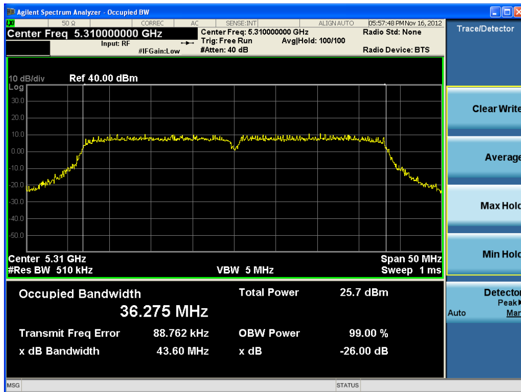
Plot 6-16. 26dB Bandwidth Plot (40MHz BW 802.11a/n (UNII Band 2) – Ch. 62)
