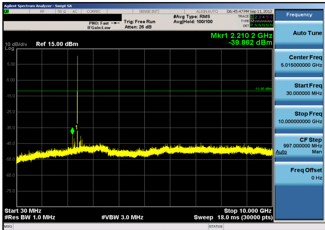
Plot 6-36. Conducted Spurious Plot (Bluetooth, 3Mbps – Ch. 0)
