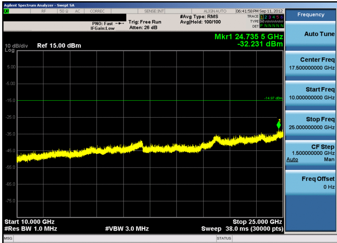
Plot 6-39. Conducted Spurious Plot (Bluetooth, 3Mbps – Ch. 39)
