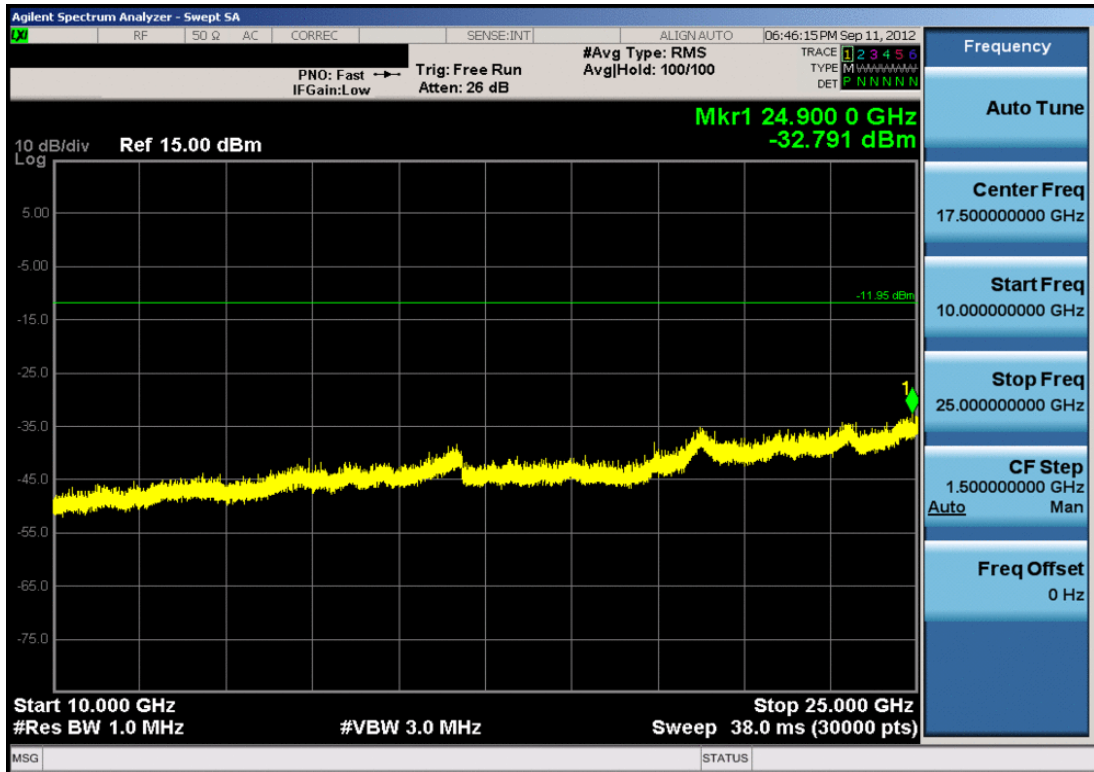
Plot 6-37. Conducted Spurious Plot (Bluetooth, 3Mbps – Ch. 0)
