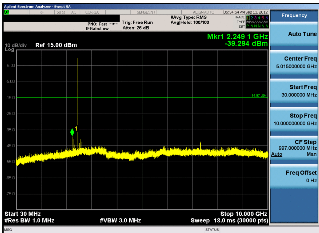
Plot 6-38. Conducted Spurious Plot (Bluetooth, 3Mbps – Ch. 39)
