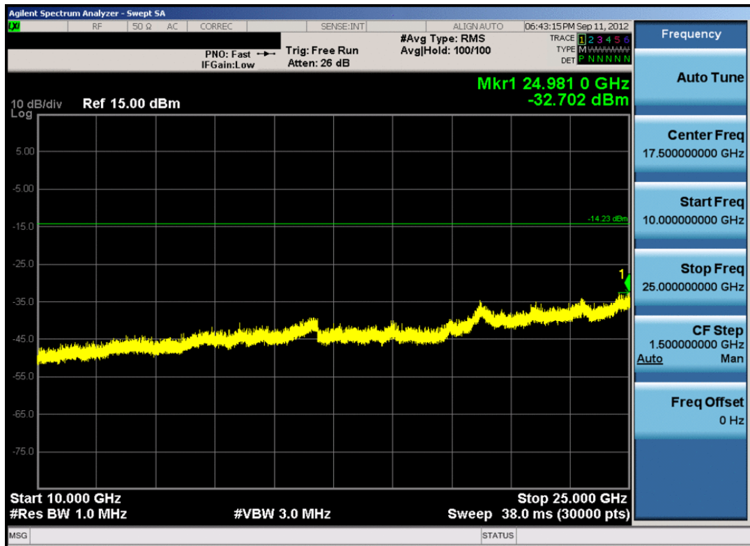
Plot 6-41. Conducted Spurious Plot (Bluetooth, 3Mbps – Ch. 78)
