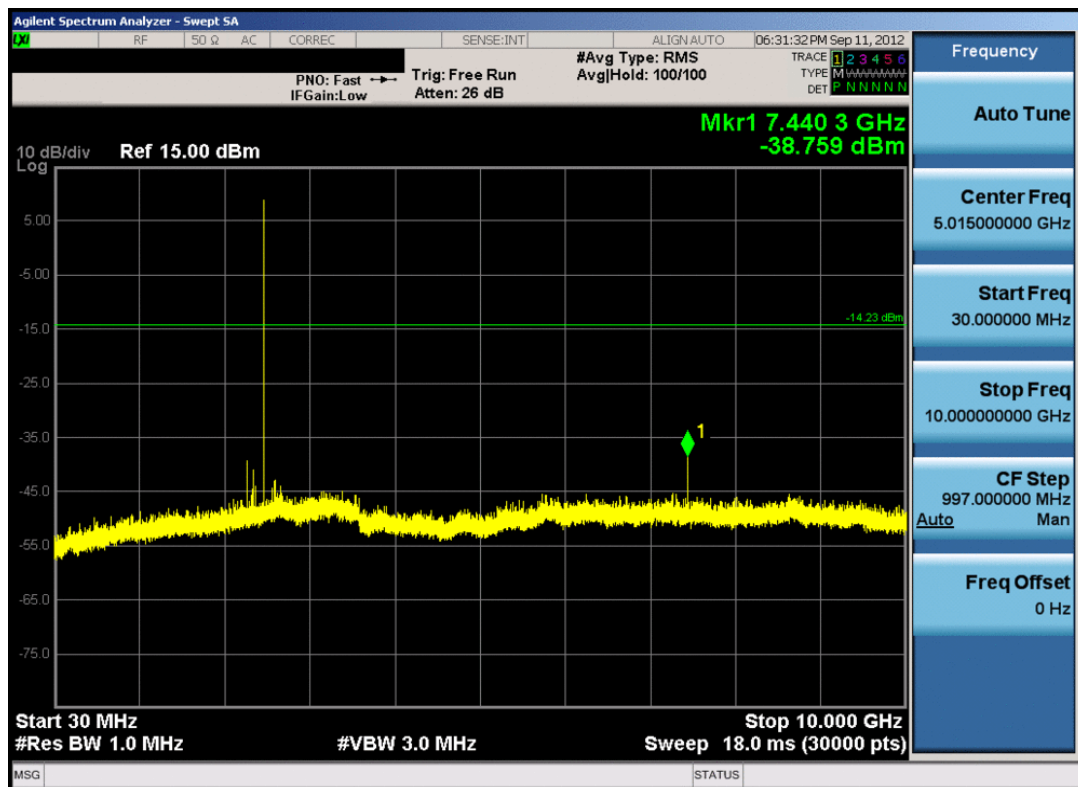
Plot 6-40. Conducted Spurious Plot (Bluetooth, 3Mbps – Ch. 78)
