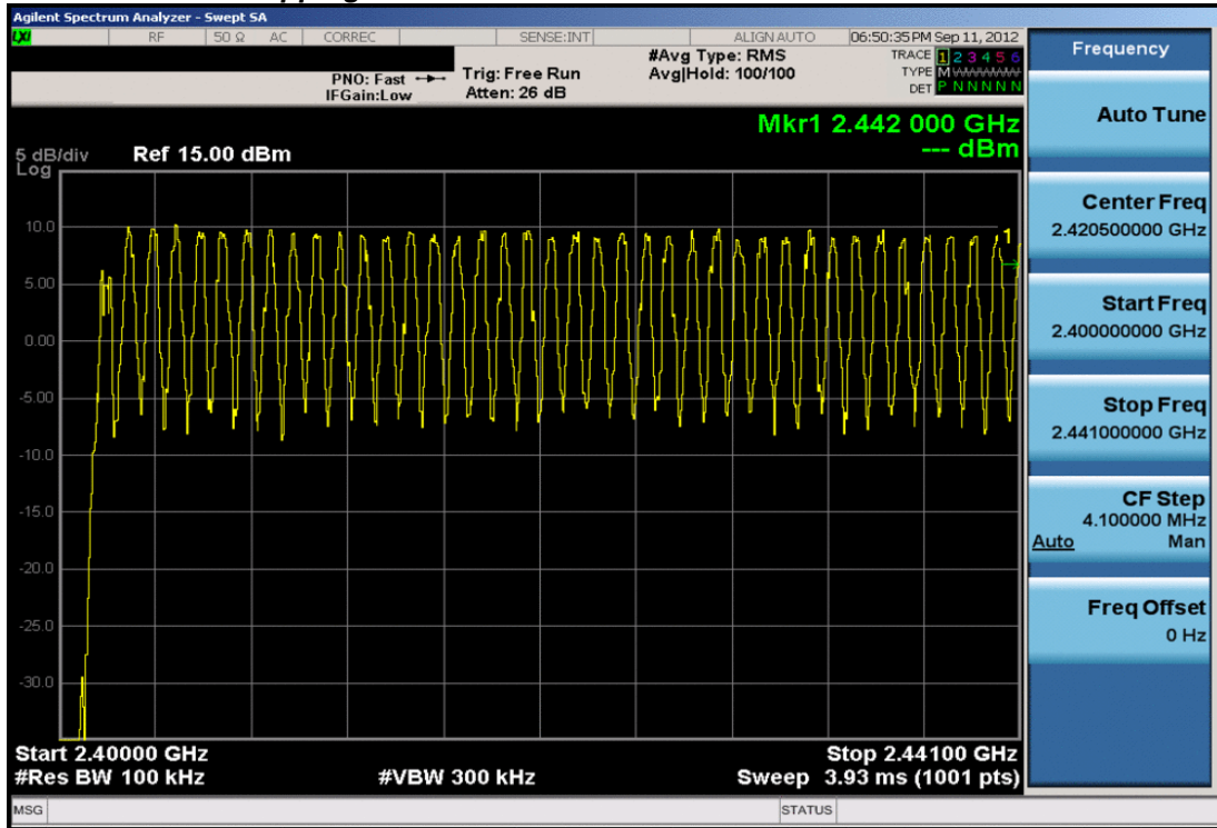
Plot 6-34. Low End Spectrum Channel Hopping Plot (Bluetooth)
