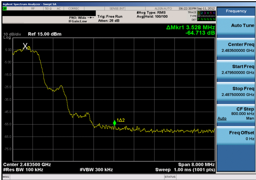
Plot 6-29. Band Edge Plot (Bluetooth with Hopping Disabled, 3Mbps – Ch. 78)
