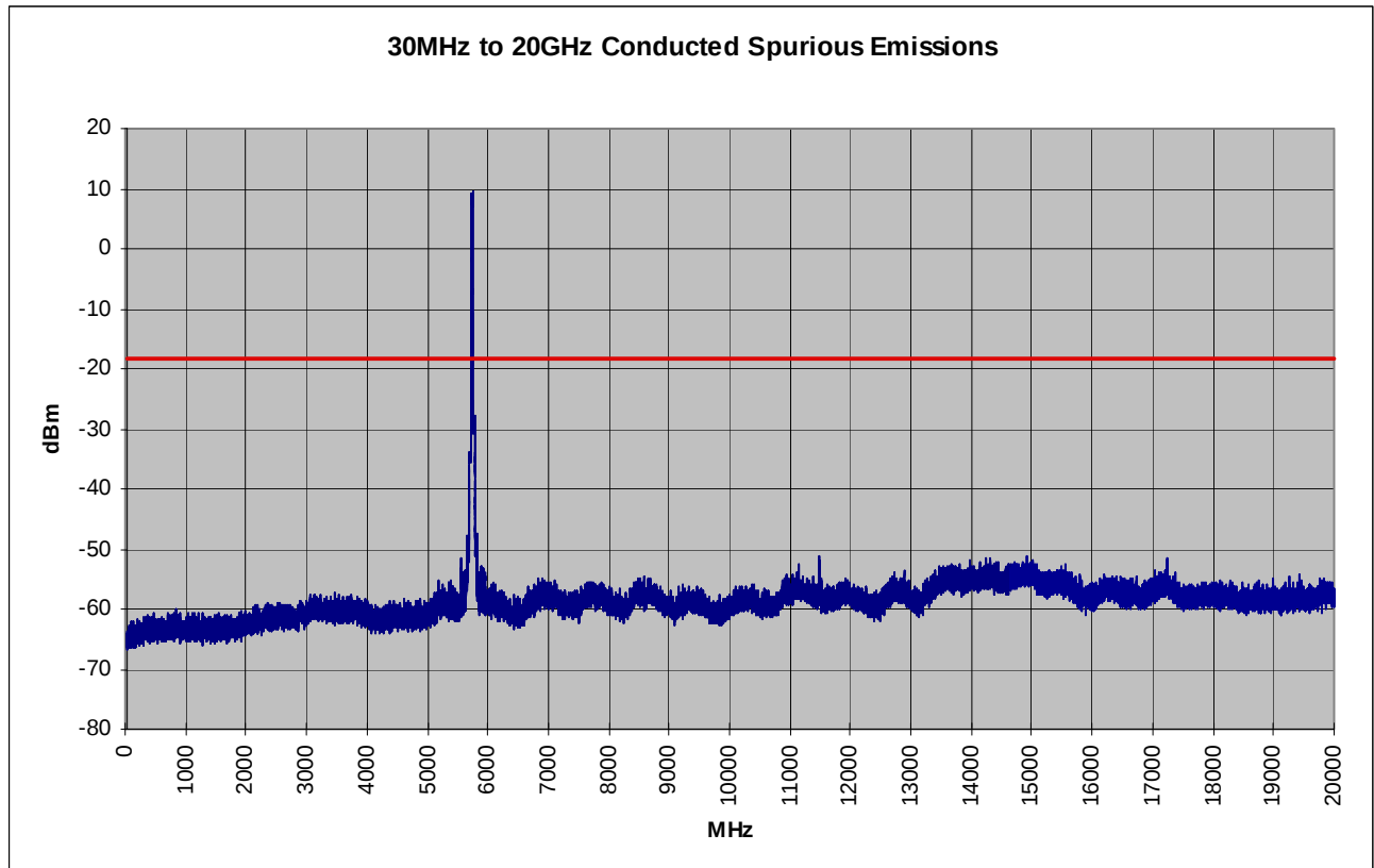
Plot 6-53. Conducted Spurious Plot (802.11a – Ch. 149)
