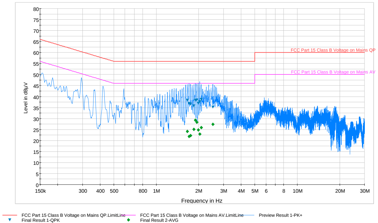
Plot 6-59. Line Conducted Plot with 802.11b (L1)
