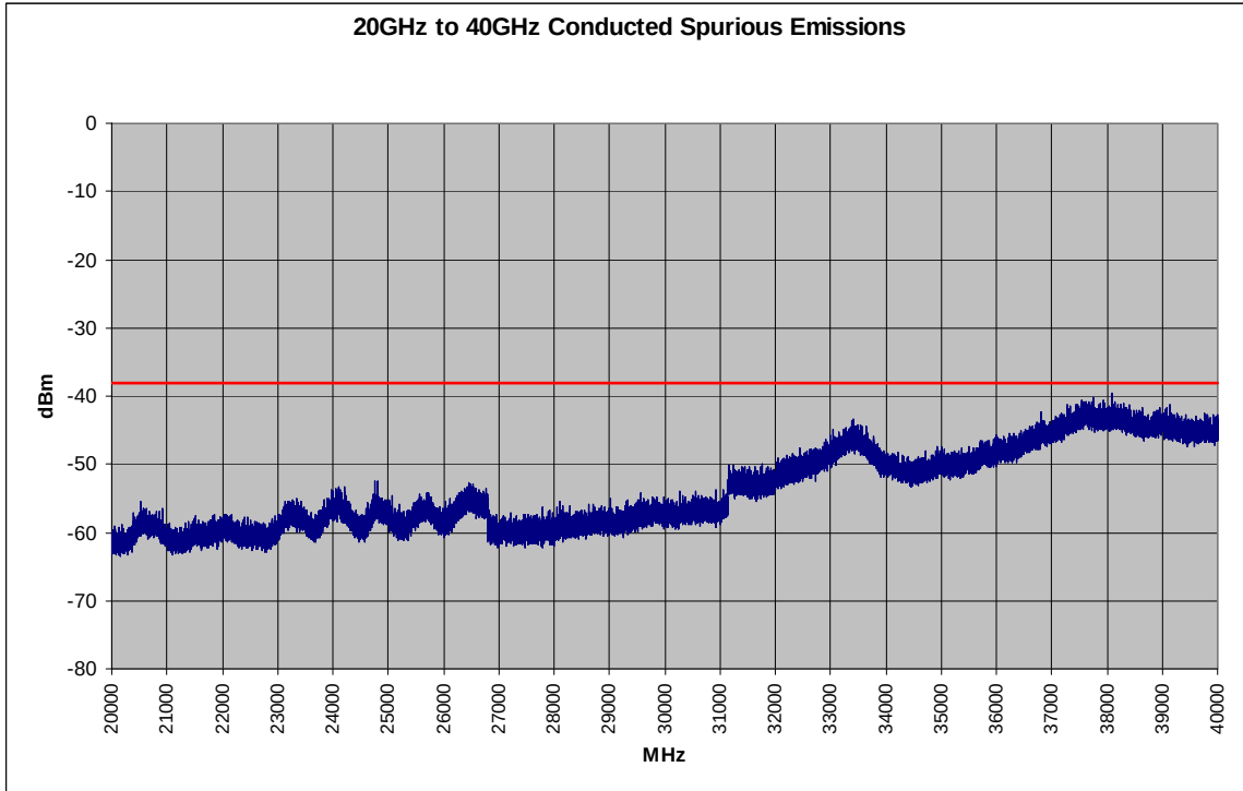
Plot 6-54. Conducted Spurious Plot (802.11a – Ch. 157)
