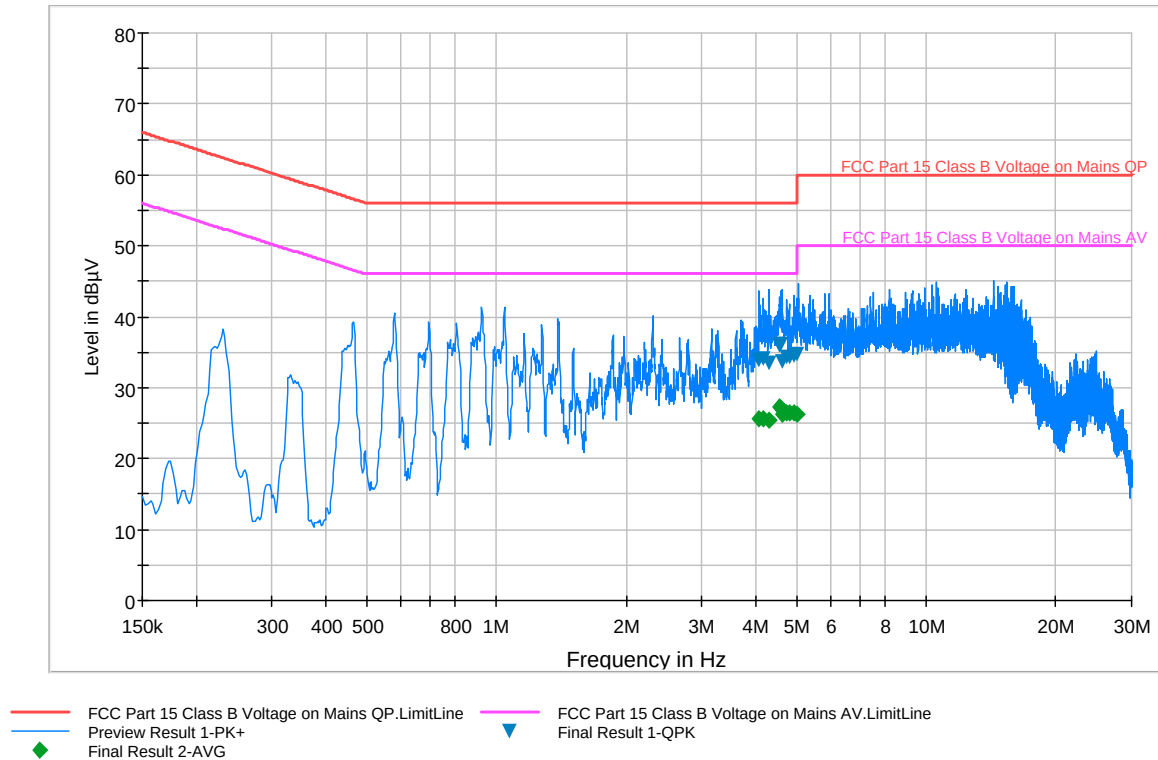
Plot 6-62. Line Conducted Plot with 802.11a (L1)
