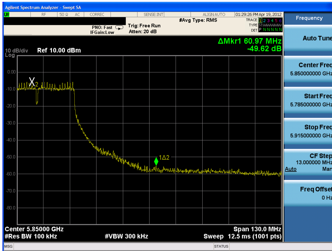
Plot 6-46. Band Edge Plot (802.11n (5.8GHz – 40MHz) – Ch. 165)
