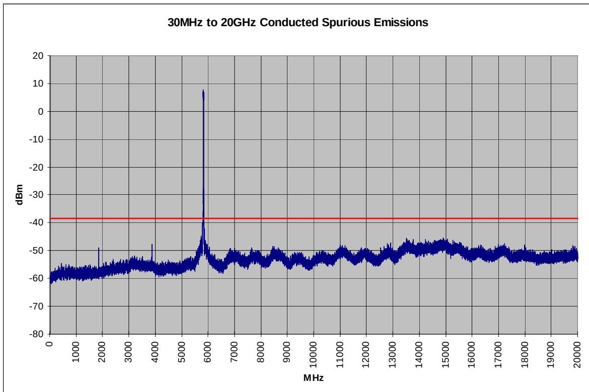
Plot 6-55. Conducted Spurious Plot (802.11a – Ch. 165)
