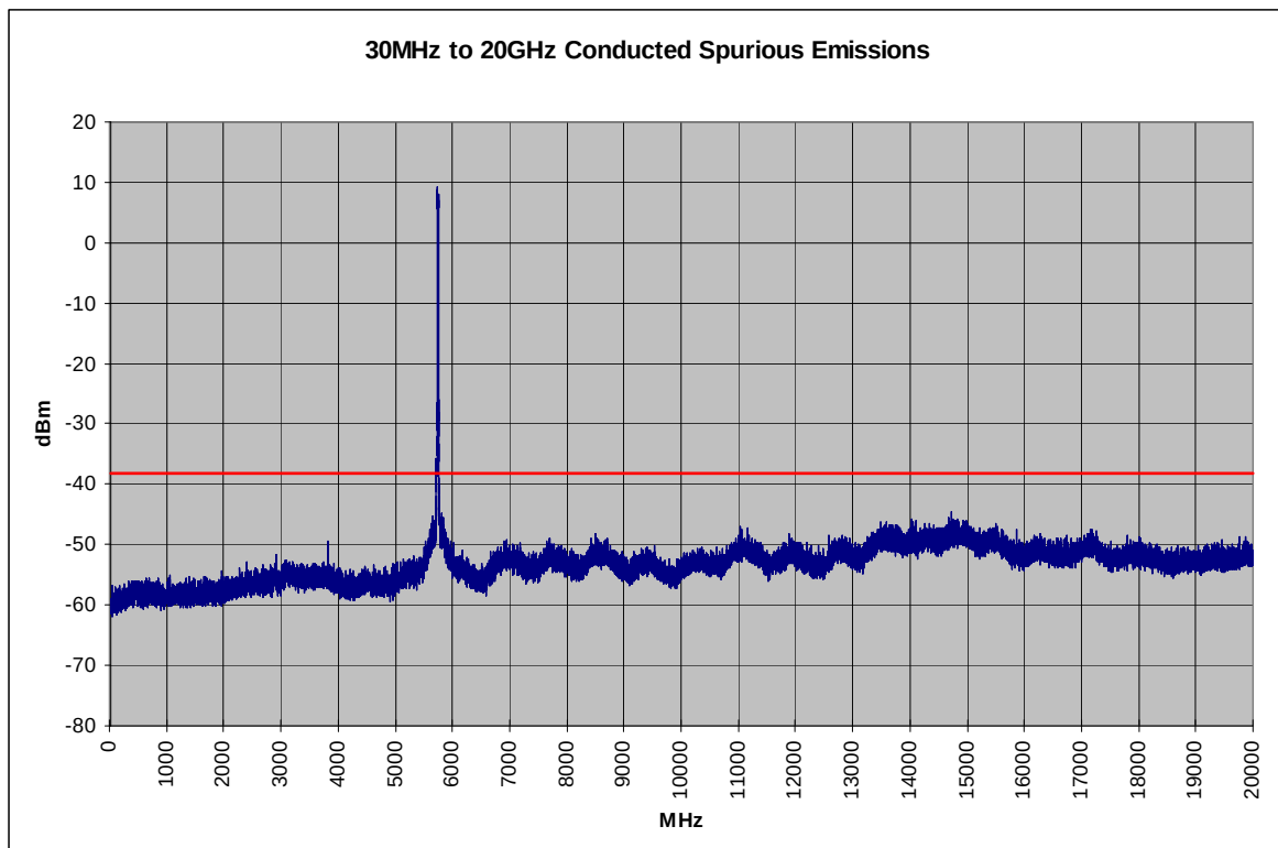
Plot 6-51. Conducted Spurious Plot (802.11a – Ch. 149)
