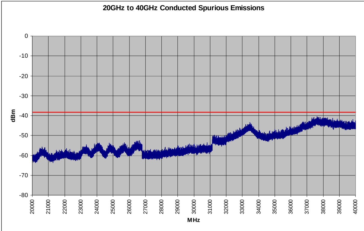
Plot 6-56. Conducted Spurious Plot (802.11a – Ch. 165)
