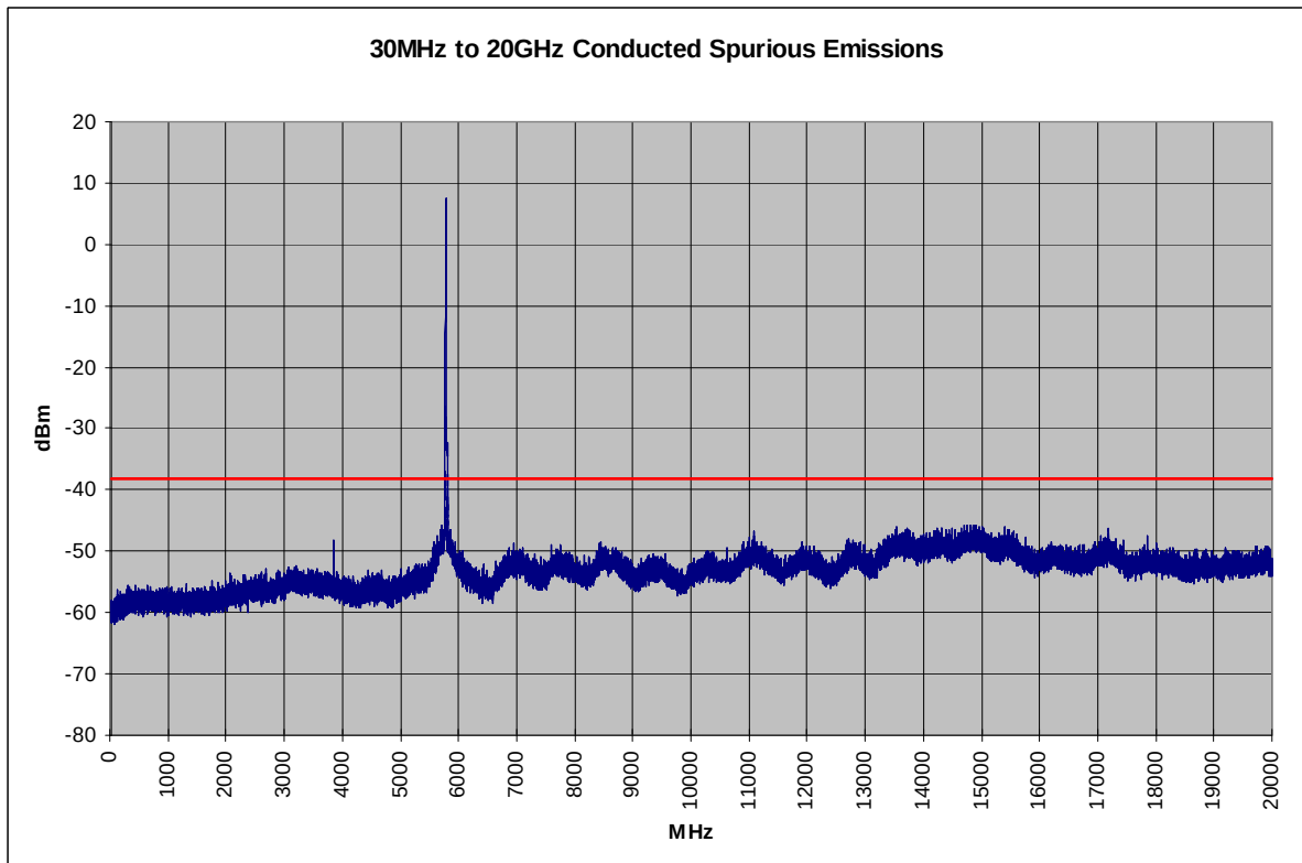
Plot 6-53. Conducted Spurious Plot (802.11a – Ch. 157)
