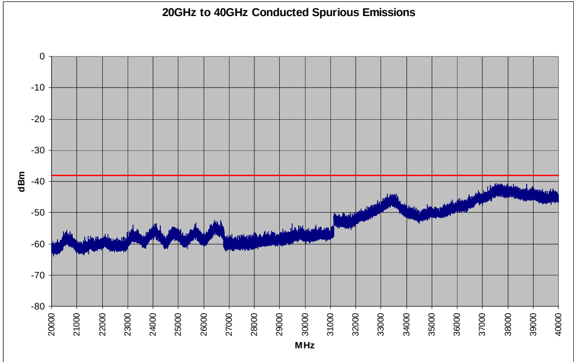
Plot 6-52. Conducted Spurious Plot (802.11a – Ch. 149)
