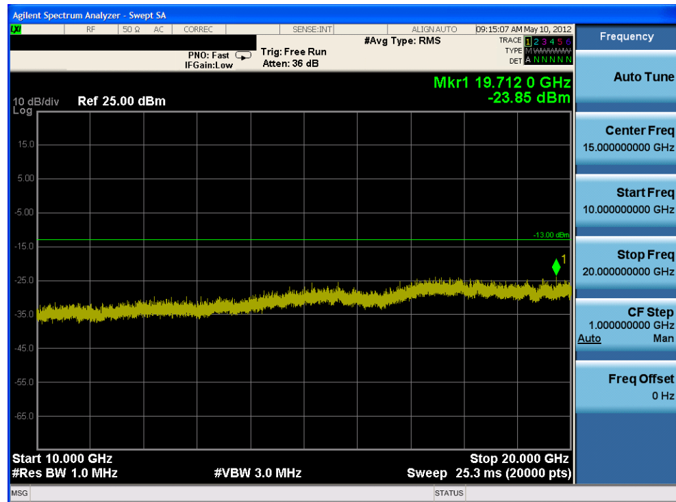
Plot 8-2. Conducted Spurious Plot (PCS CDMA Mode – Ch. 25)
