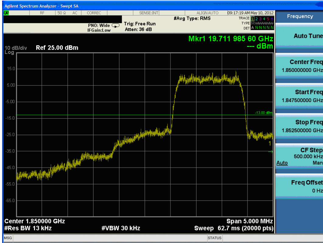
Plot 8-3. Band Edge Plot (PCS CDMA Mode – Ch. 25)
