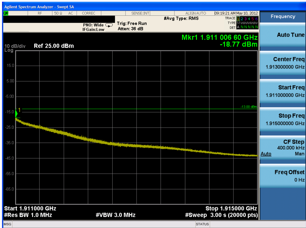
Plot 8-12. Extended Band Edge Plot (PCS CDMA Mode - Ch. 1175)
