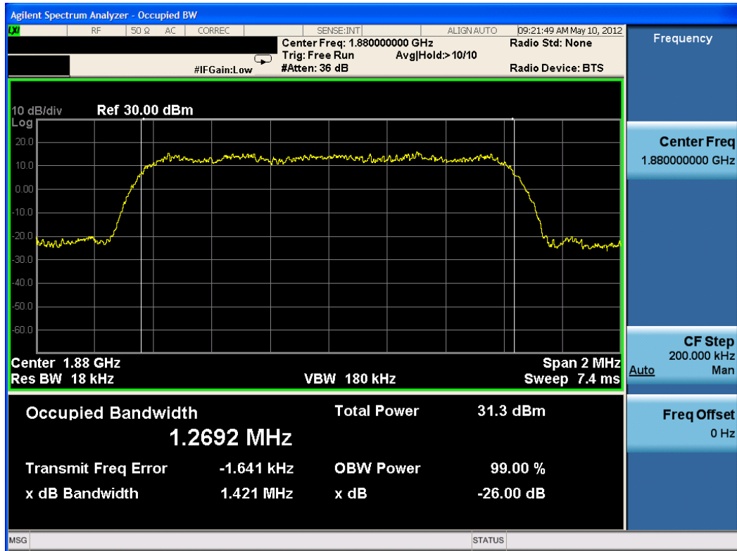
Plot 8-7. Occupied Bandwidth Plot (PCS CDMA Mode – Ch. 600)
