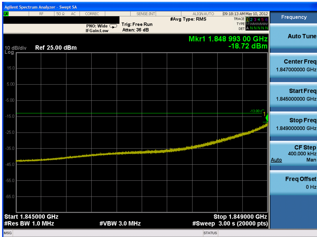
Plot 8-4. Extended Band Edge Plot (PCS CDMA Mode – Ch. 25)
