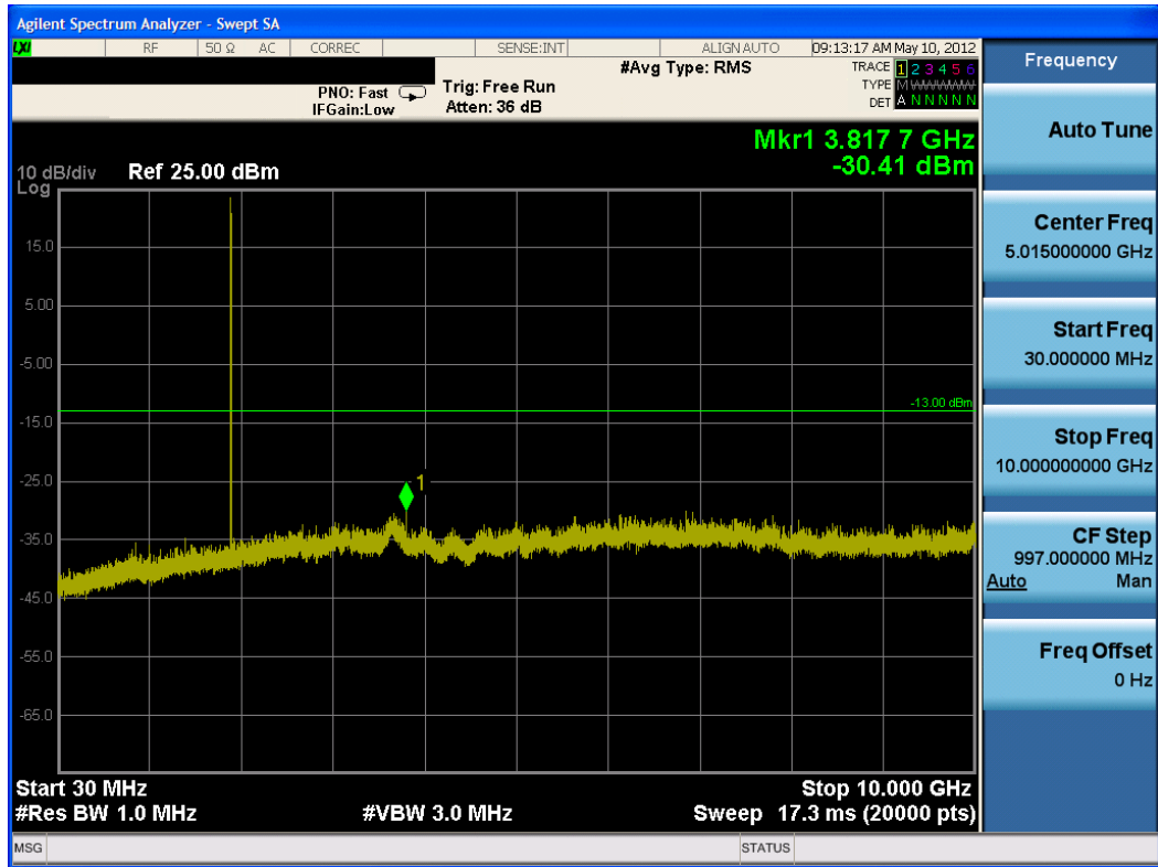
Plot 8-9. Conducted Spurious Plot (PCS CDMA Mode – Ch. 1175)
