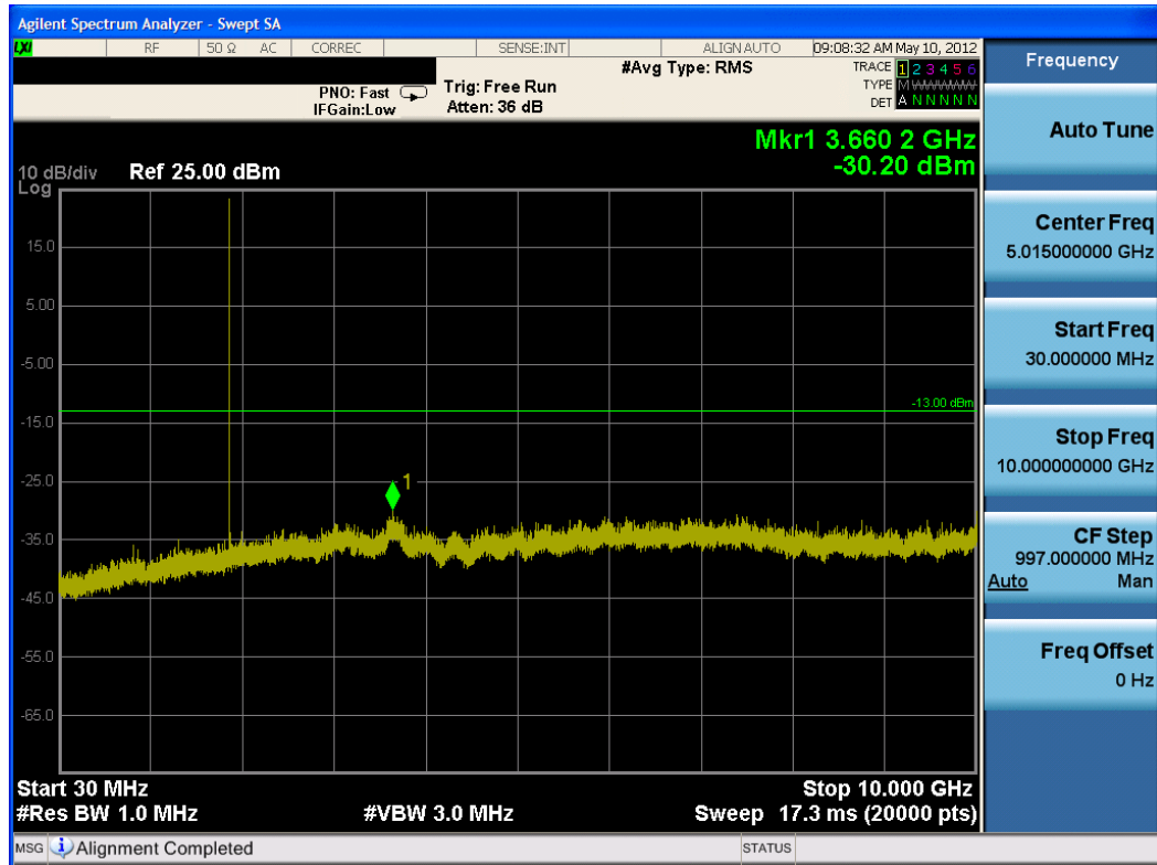
Plot 8-5. Conducted Spurious Plot (PCS CDMA Mode – Ch. 600)
