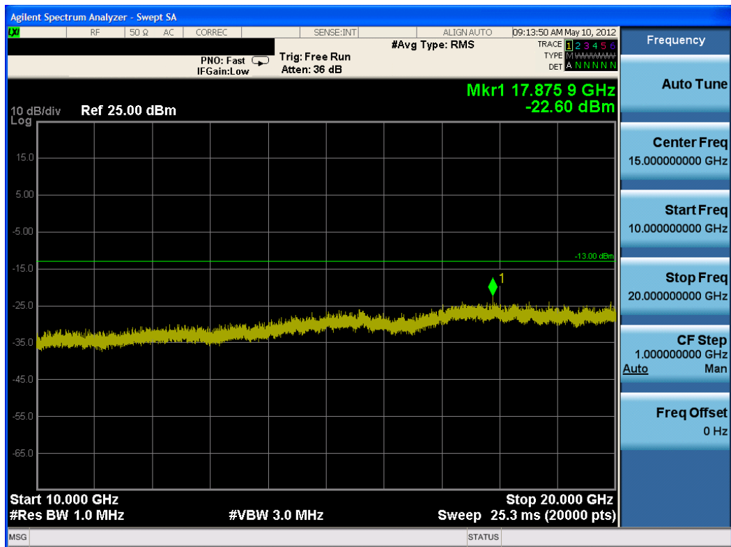
Plot 8-10. Conducted Spurious Plot (PCS CDMA Mode – Ch. 1175)
