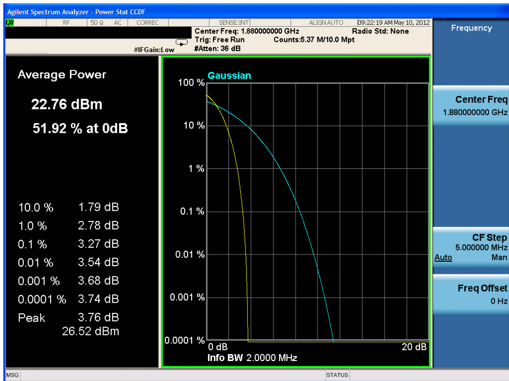
Plot 8-8. Peak-Average Ratio Plot (PCS CDMA Mode – Ch. 600)
