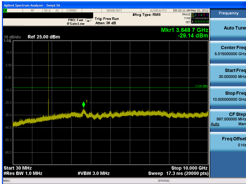
Plot 8-1. Conducted Spurious Plot (PCS CDMA Mode – Ch. 25)
