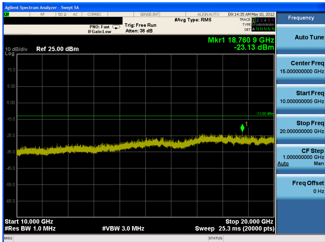
Plot 8-6. Conducted Spurious Plot (PCS CDMA Mode – Ch. 600)
