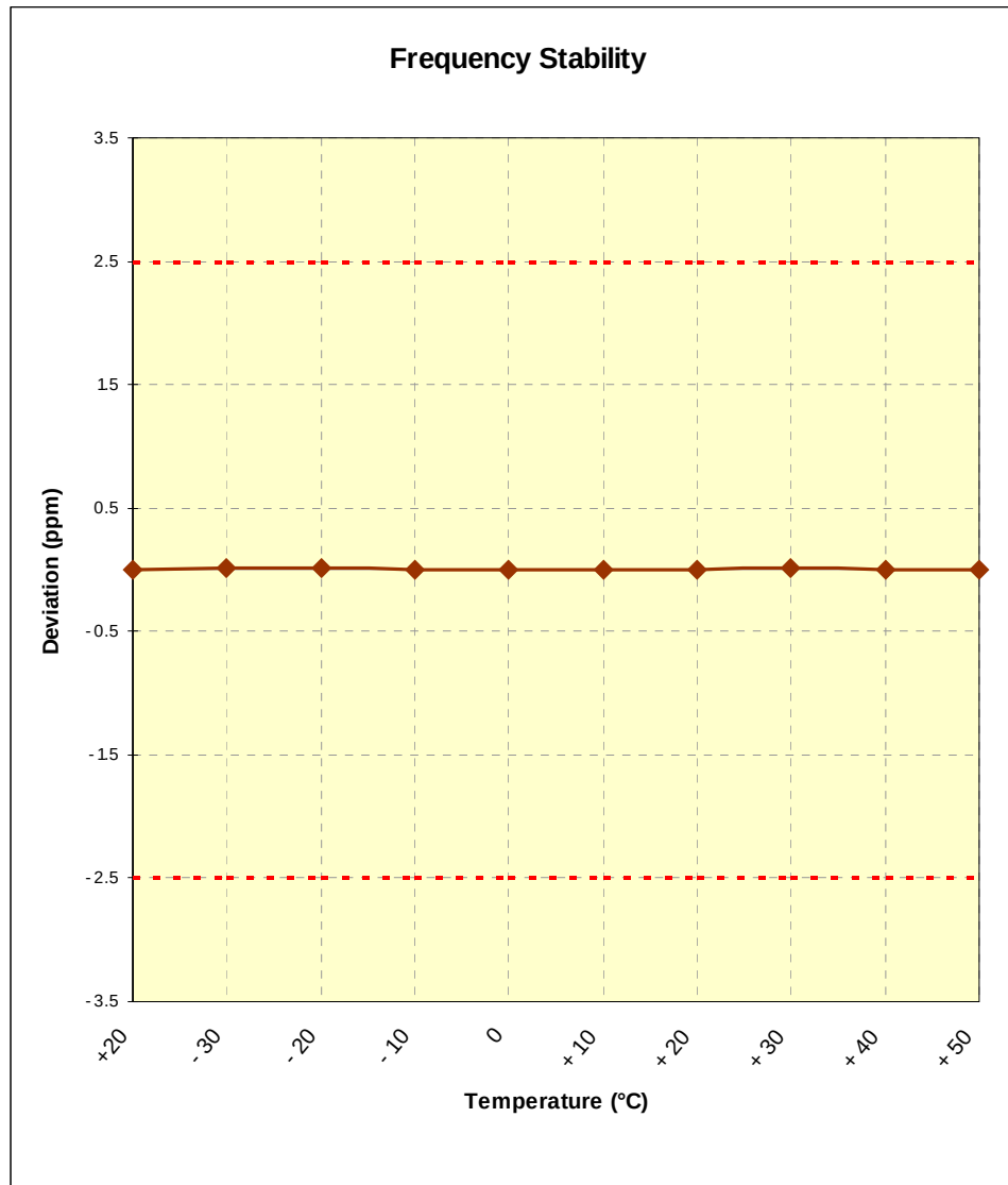
Plot 6-2. Frequency Stability Graph (PCS CDMA Mode – Ch. 600)
