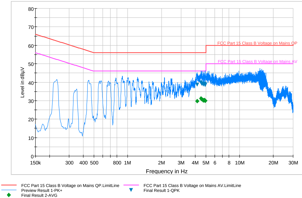
Plot 6-81. Line Conducted Plot with 802.11a (UNII Band 3) (LN)
