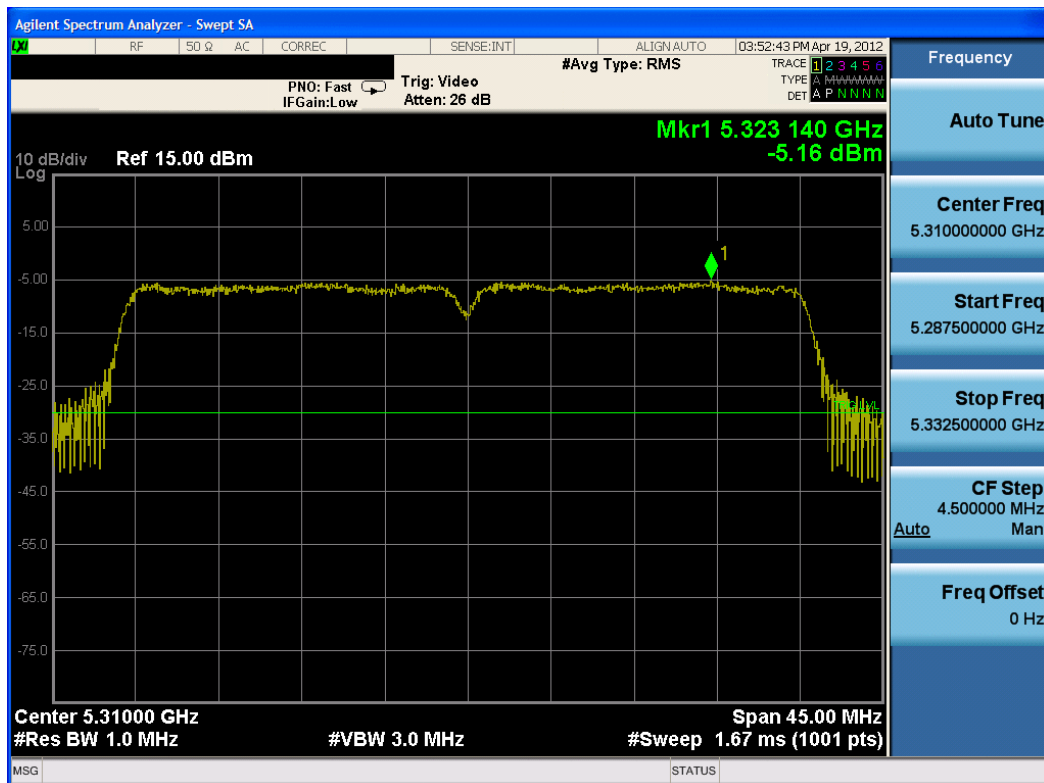
Plot 6-41. Peak Power Spectral Density Plot (802.11n – 40MHz BW (UNII Band 2) – Ch. 62)
