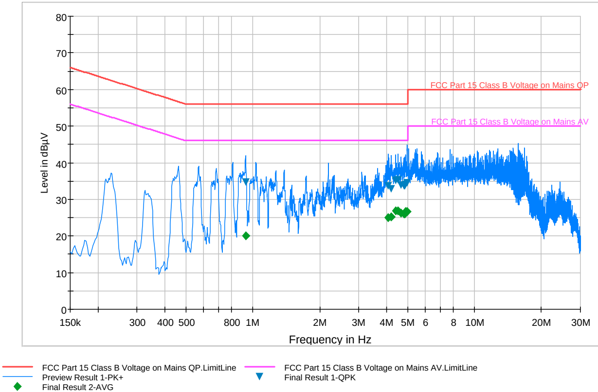
Plot 6-80. Line Conducted Plot with 802.11a (UNII Band 3) (L1)
