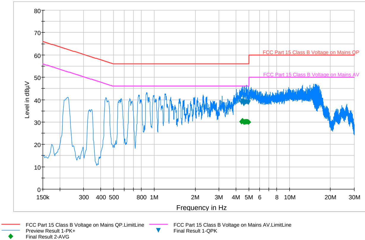
Plot 6-77. Line Conducted Plot with 802.11a (UNII Band 1) (LN)
