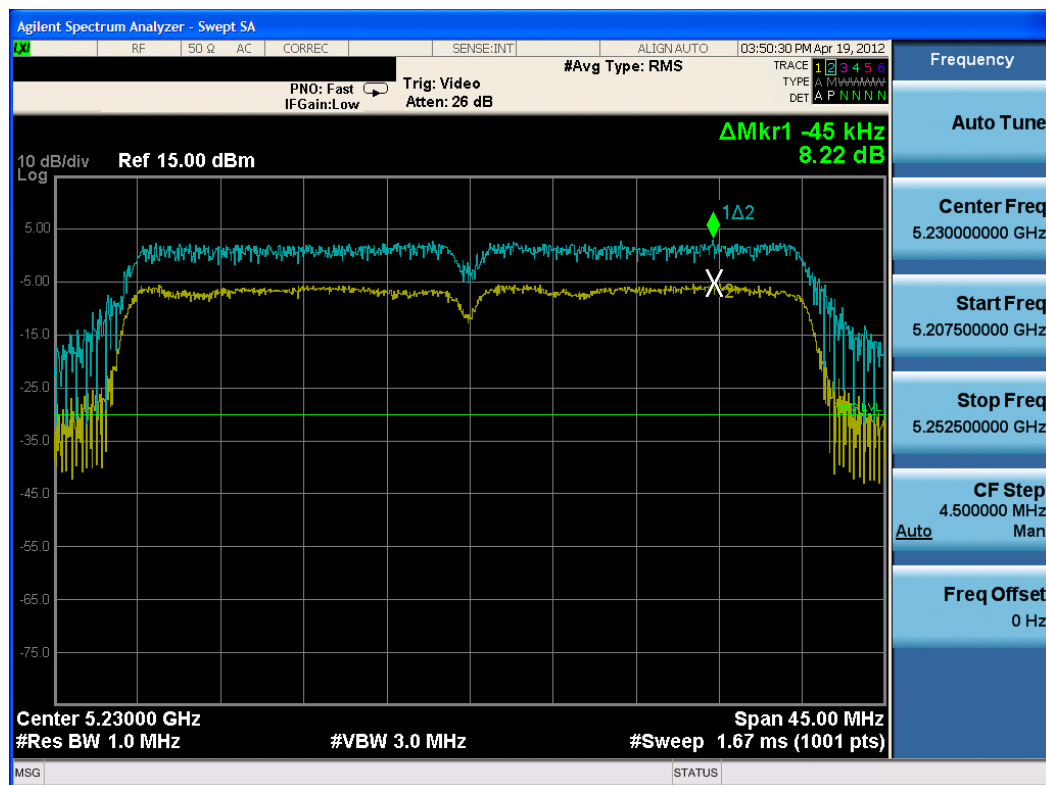
Plot 6-58. Peak Excursion Ratio Plot (802.11n – 40MHz BW (UNII Band 1) – Ch. 46)
