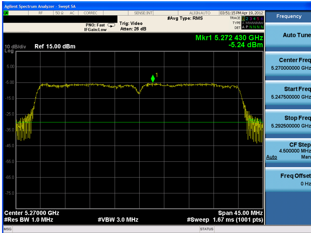
Plot 6-40. Peak Power Spectral Density Plot (802.11n – 40MHz BW (UNII Band 2) – Ch. 54)
