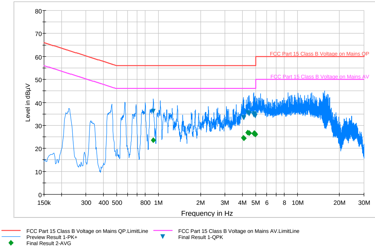
Plot 6-76. Line Conducted Plot with 802.11a (UNII Band 1) (L1)
