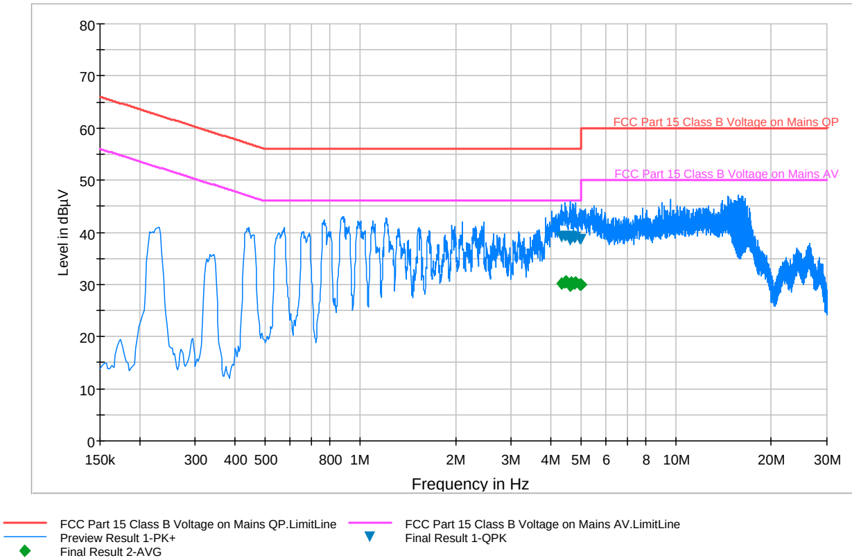
Plot 6-79. Line Conducted Plot with 802.11a (UNII Band 2) (LN)
