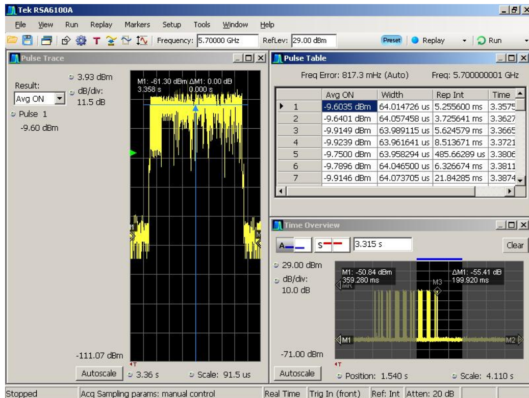
Figure 6-6. Aggregate Time using Pulse Table Capability
