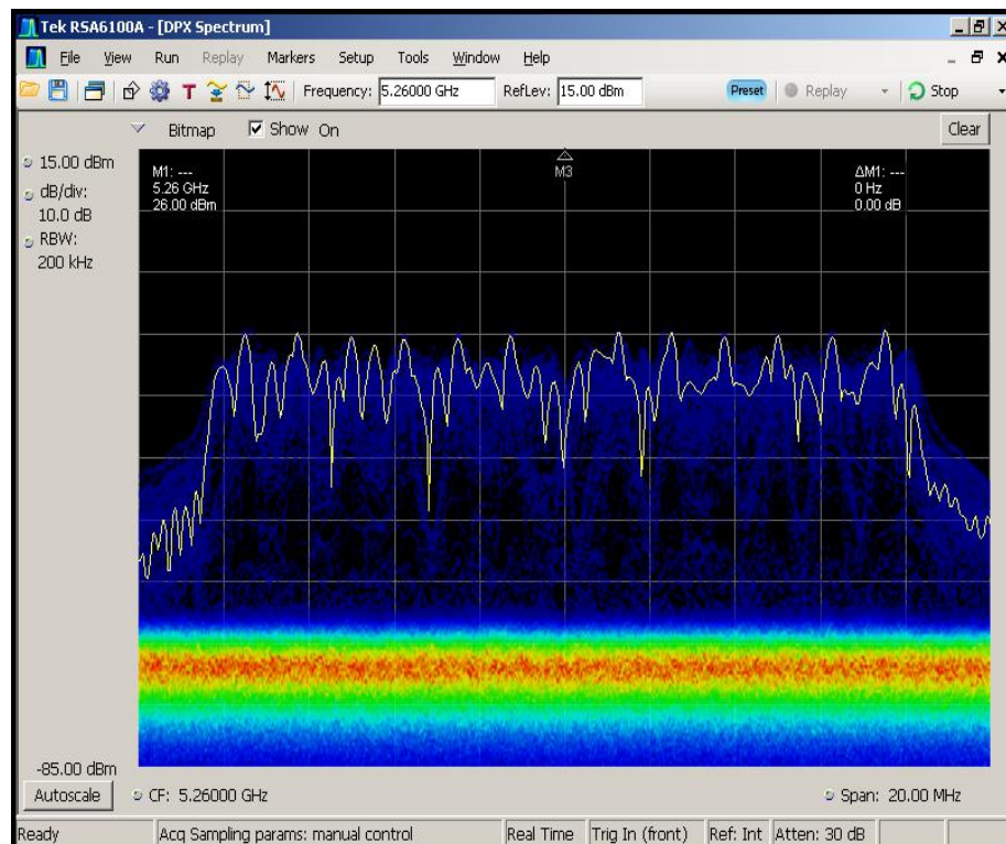
Figure 5-4. Real-Time Spectrum Display, WLAN Traffic (Streaming Video)
