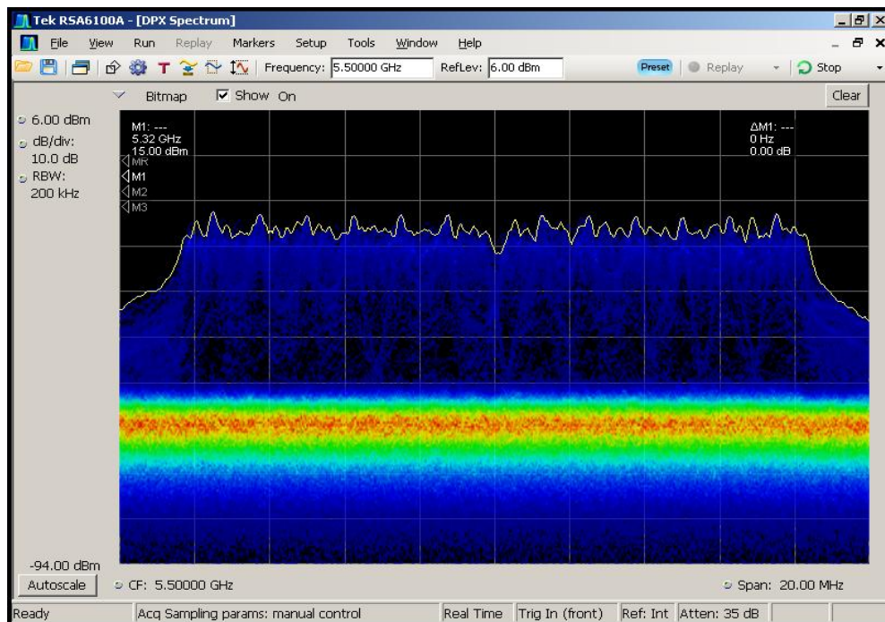
Figure 6-4. Real-Time Spectrum Display, WLAN Traffic (Streaming Video)
