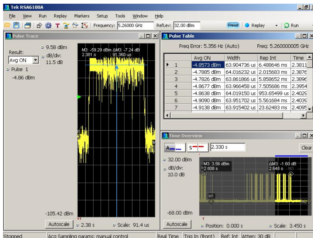
Figure 5-6. Aggregate Time using Pulse Table Capability
