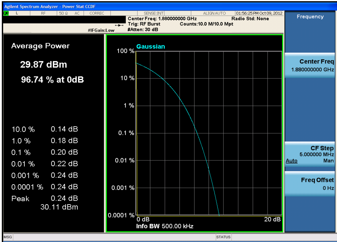
Plot 7-7. Peak-Average Ratio Plot (PCS GSM Mode – Ch. 661)
