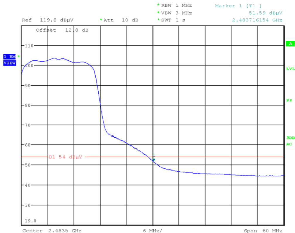
Plot 6-53. Radiated Upper Band Measurement (Average)
