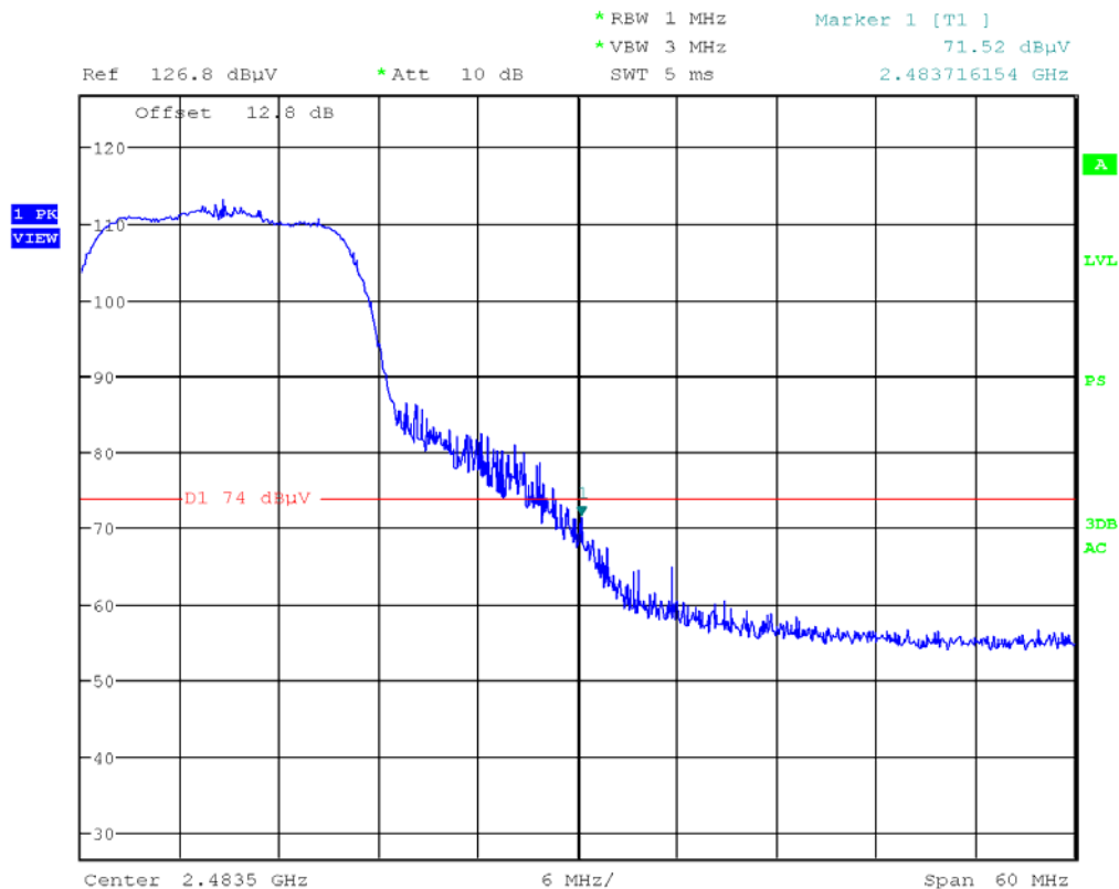
Plot 6-54. Radiated Upper Band Measurement (Peak)
