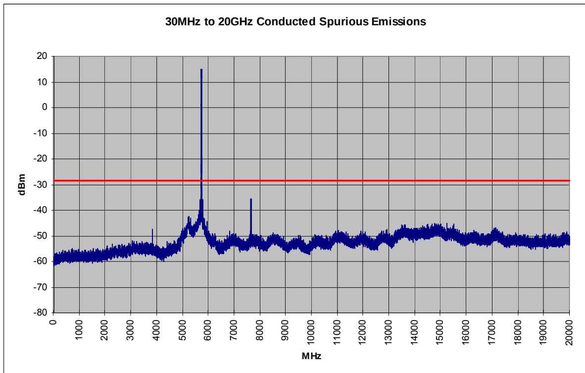
Plot 6-47. Conducted Spurious Plot (802.11a – Ch. 149)
