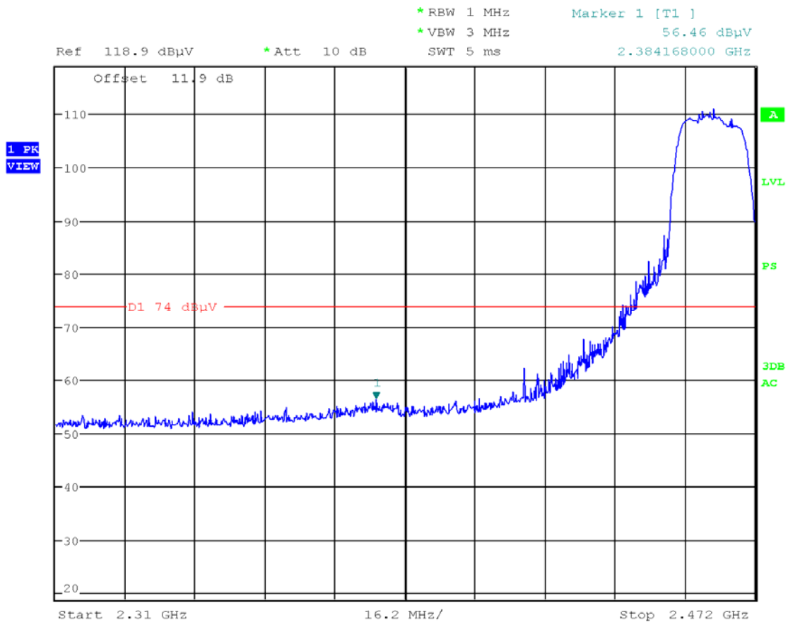
Plot 6-56. Radiated Lower Band Measurement (Peak)
