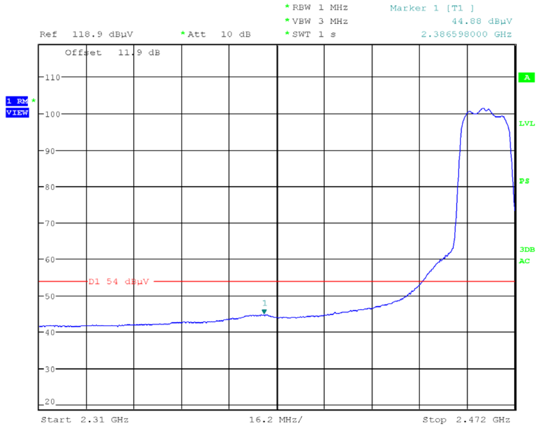
Plot 6-55. Radiated Lower Band Measurement (Average)
