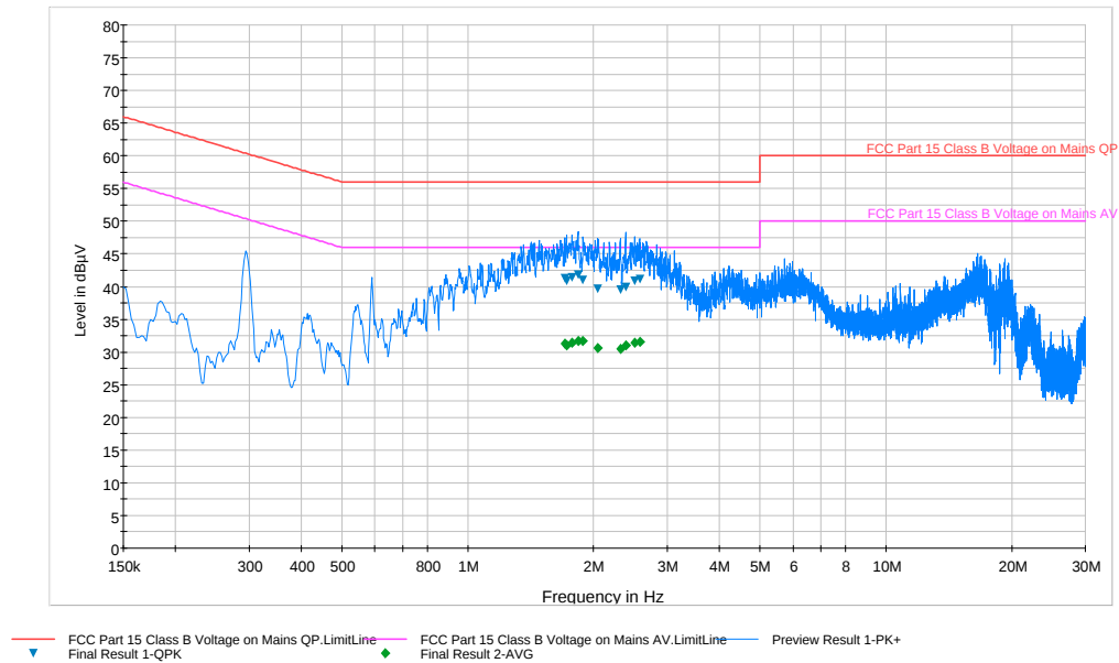
Plot 6-44. Line Conducted Plot with 802.11a UNII Band 3 (N)
