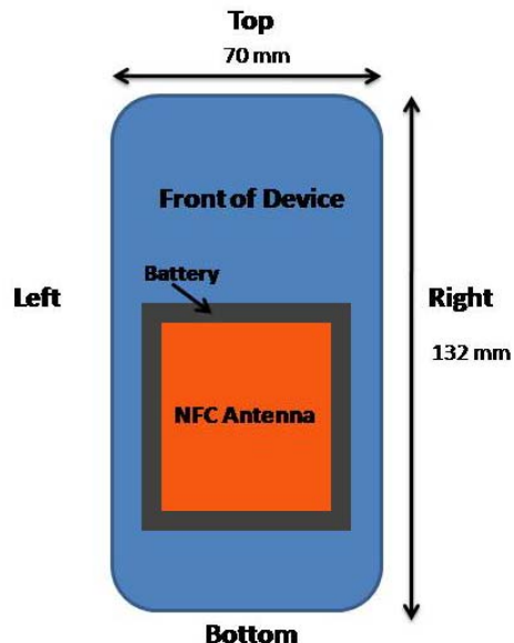
Figure 1-2 NFC Antenna Locations
