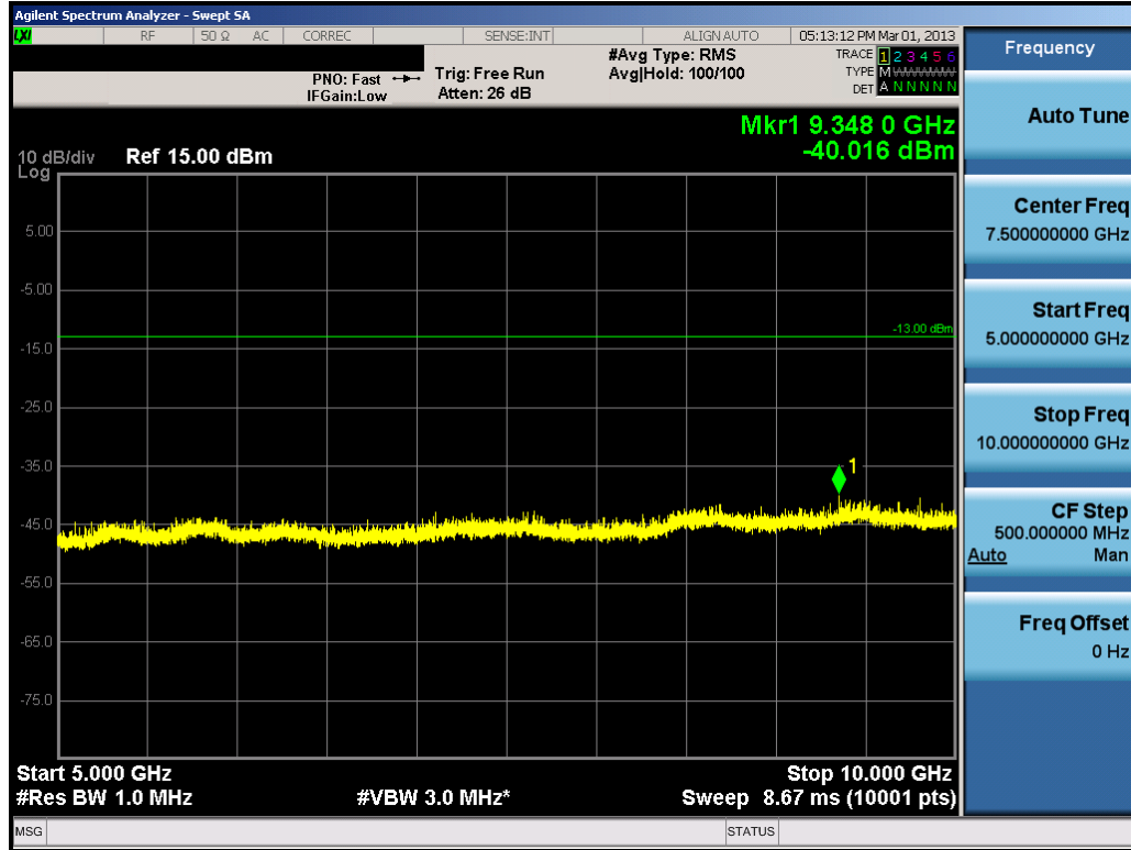
Plot 7-18. Conducted Spurious Plot (Cellular CDMA Mode – Ch. 384)
