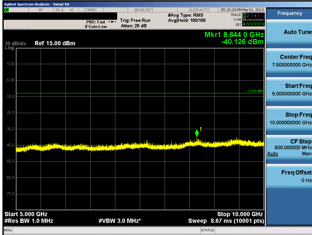
Plot 7-14. Conducted Spurious Plot (Cellular CDMA Mode – Ch. 1013)
