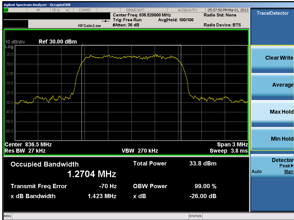
Plot 7-19. Occupied Bandwidth Plot (Cellular CDMA Mode – Ch. 384)
