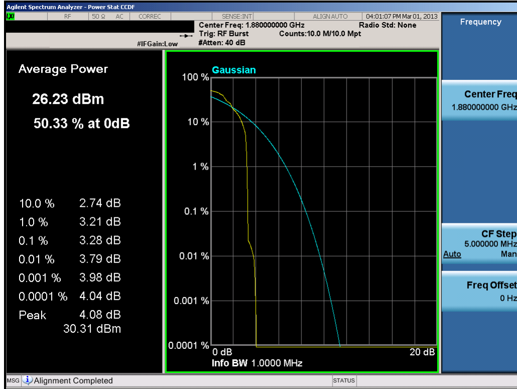
Plot 7-12. Peak-Average Ratio Plot (EDGE1900 Mode – Ch. 661, 1-slot EDGE)
