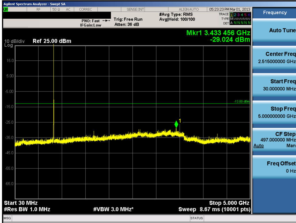
Plot 7-20. Conducted Spurious Plot (Cellular CDMA Mode – Ch. 777)
