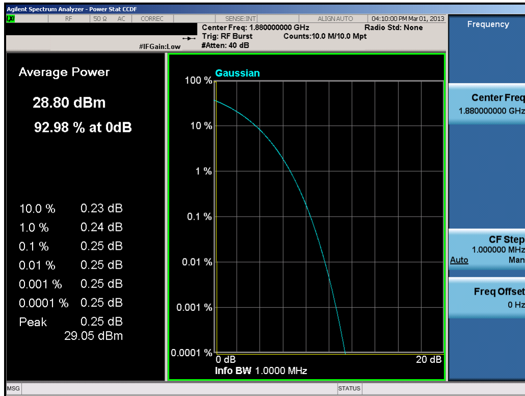
Plot 7-7. Peak-Average Ratio Plot (PCS GSM Mode – Ch. 661, 1-slot GPRS)
