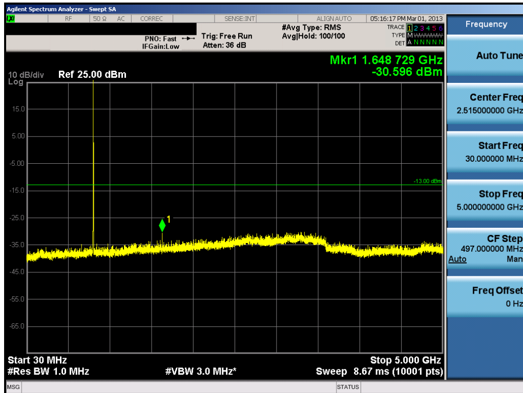
Plot 7-13. Conducted Spurious Plot (Cellular CDMA Mode – Ch. 1013)
