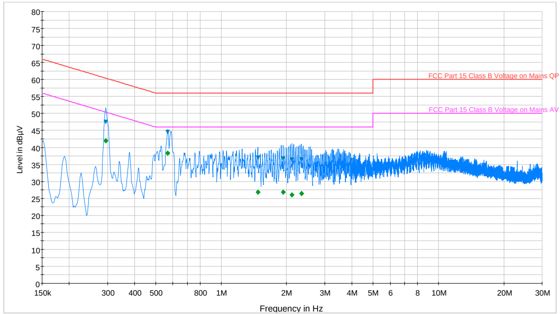
Plot 6-85. Line Conducted Plot with 802.11a UNII Band 3 (L1)
