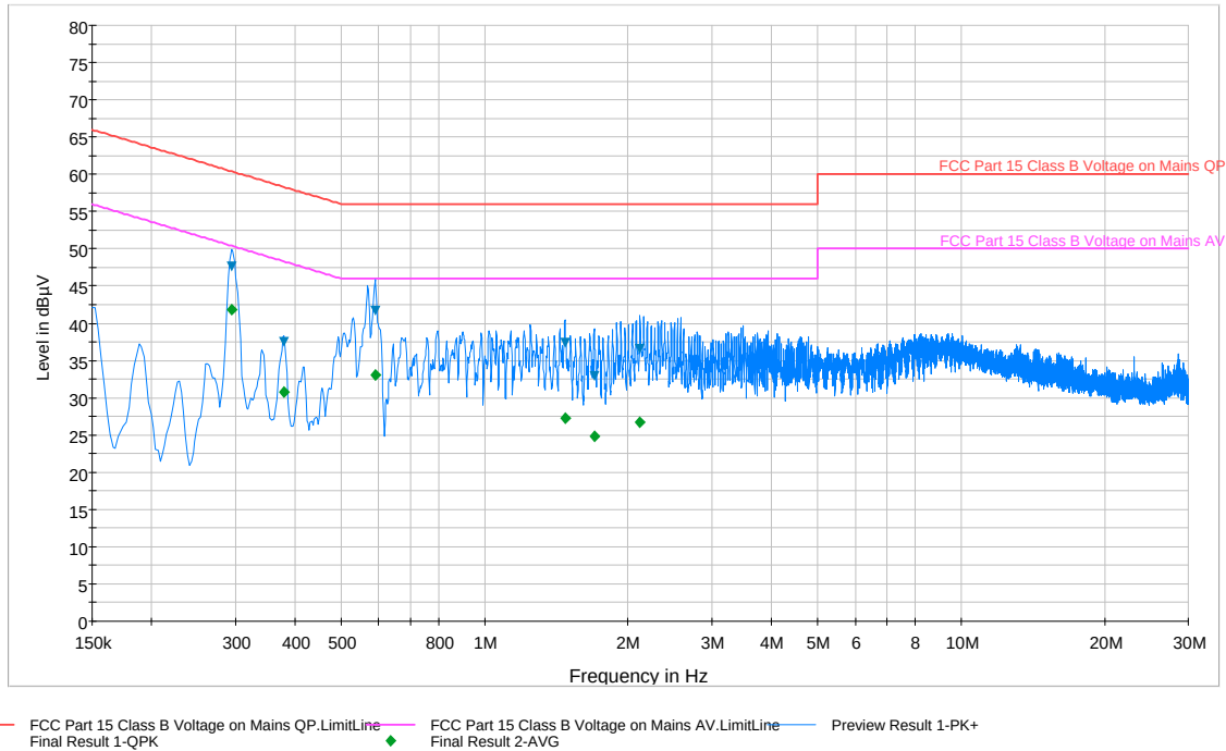
Plot 6-81. Line Conducted Plot with 802.11a UNII Band 1 (L1)
