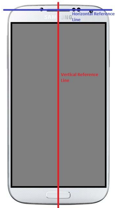
SAR Test Setup Photo 6 – DUT Horizontal and Vertical Reference Lines
