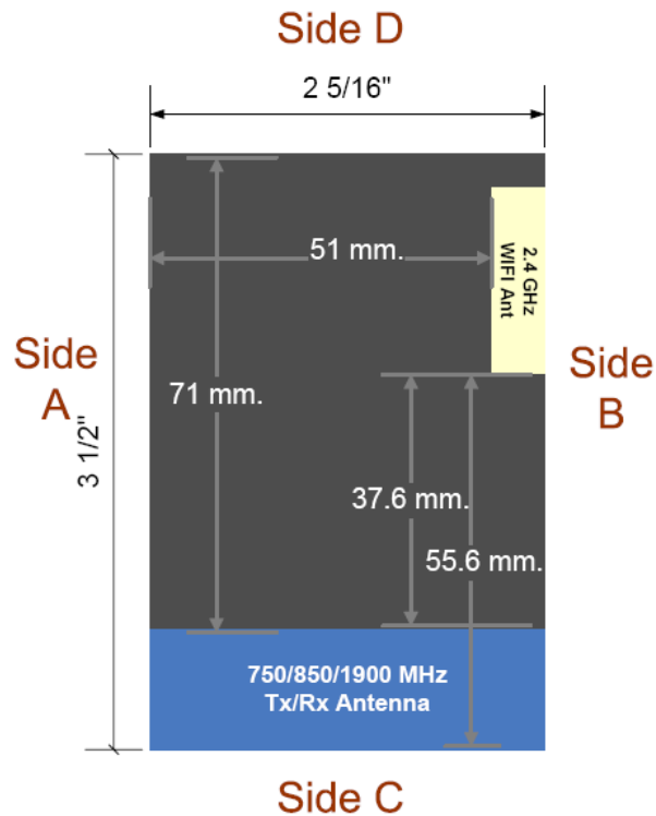
Figure 13-1 Antenna Locations, as viewed from back of device
