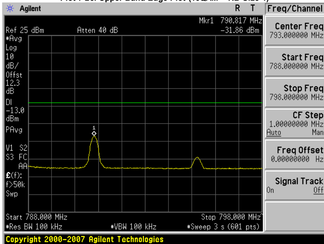
Plot 7-26. Upper Band Edge Plot (QPSK – RB Size 1)
