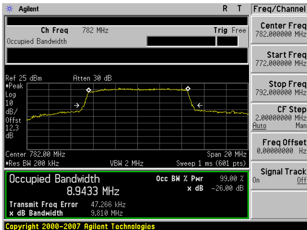
Plot 7-14. Occupied Bandwidth Plot (QPSK - RB Size 25, RB Offset 13)
