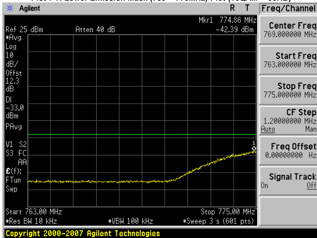
Plot 7-8. Lower Emission Mask (763 – 775MHz) Plot (QPSK– 50RB)
