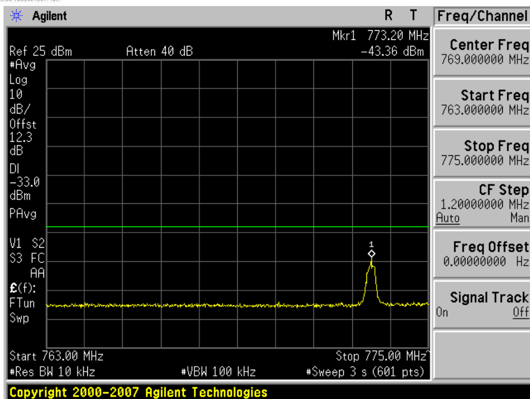
Plot 7-6. Lower Emission Mask (763 – 775MHz) Plot (QPSK– 1RB)
