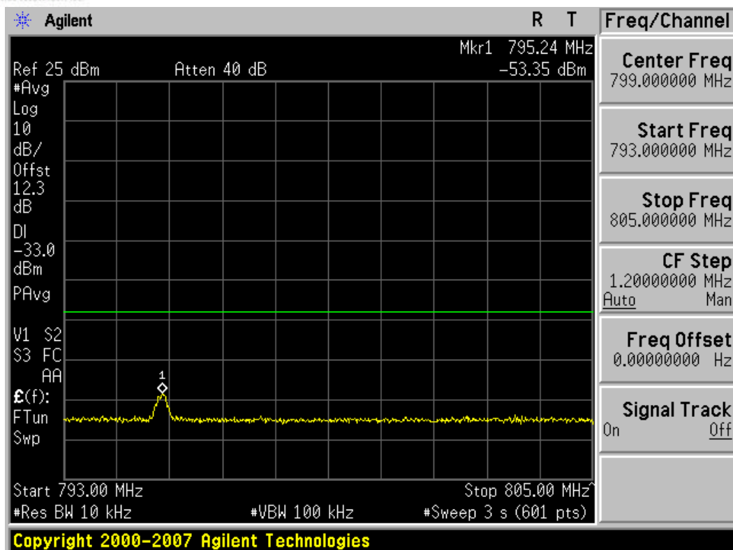
Plot 7-30. Upper Emissions Mask (793 – 805MHz) Plot (QPSK – RB Size 1)
