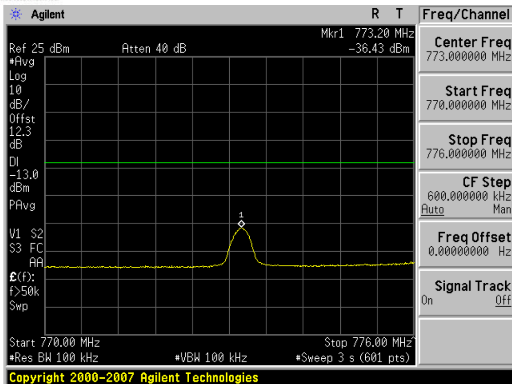
Plot 7-2. Lower Band Edge Plot (QPSK – RB Size 1)
