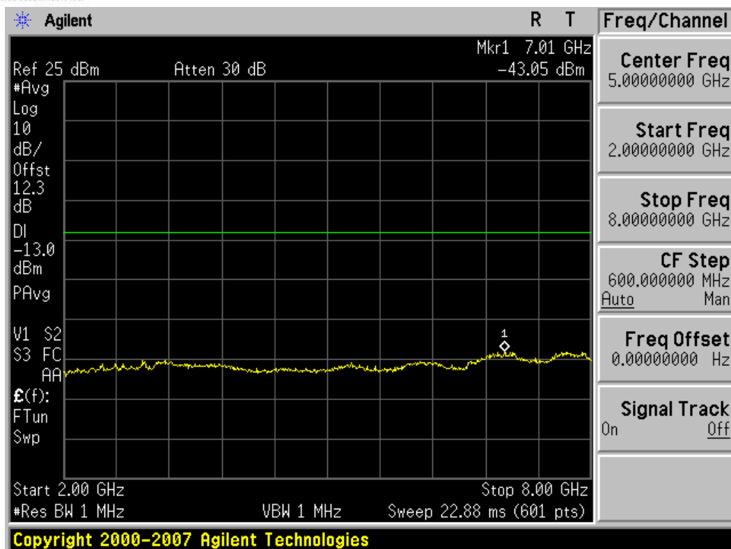
Plot 7-22. Conducted Spurious Plot (16QAM – RB Size 50)
