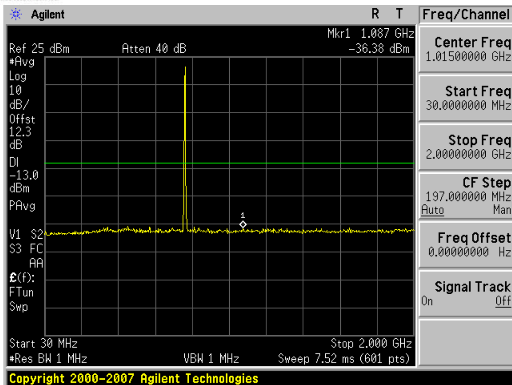
Plot 7-17. Conducted Spurious Plot (16QAM – RB Size 1)
