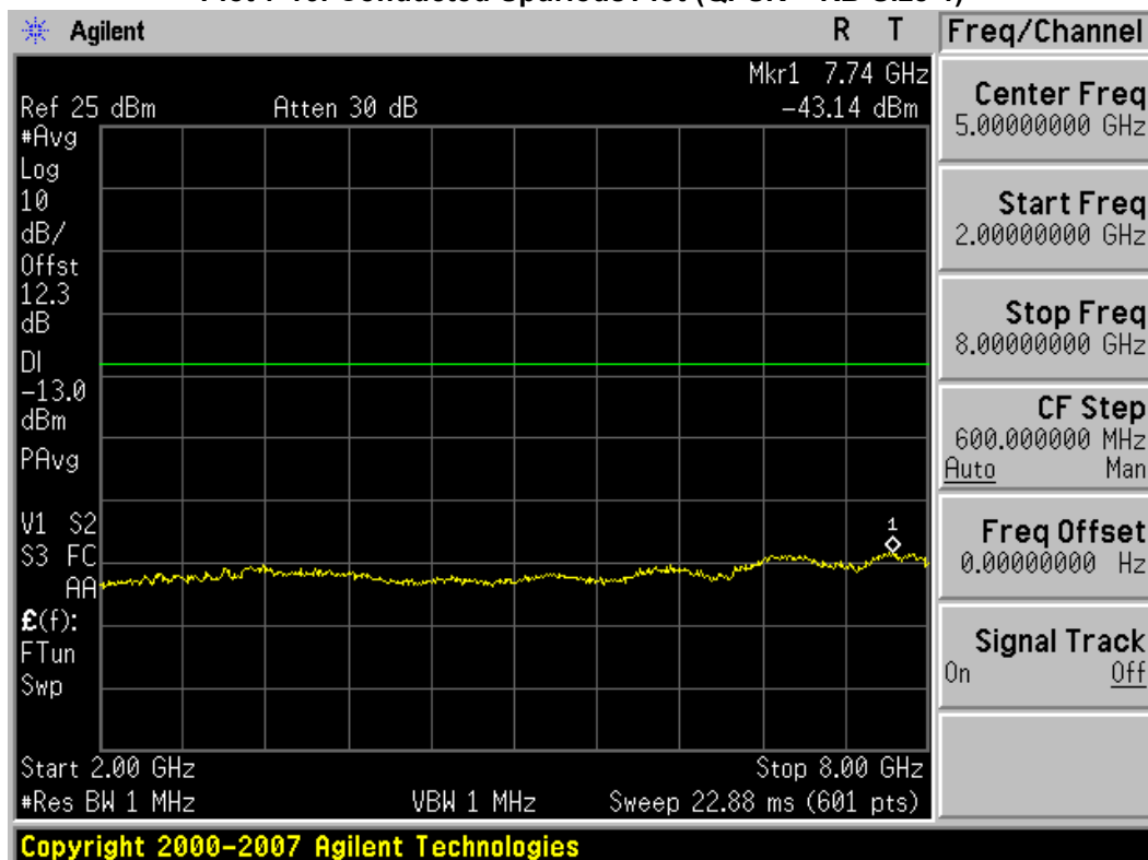
Plot 7-19. Conducted Spurious Plot (QPSK – RB Size 1)
