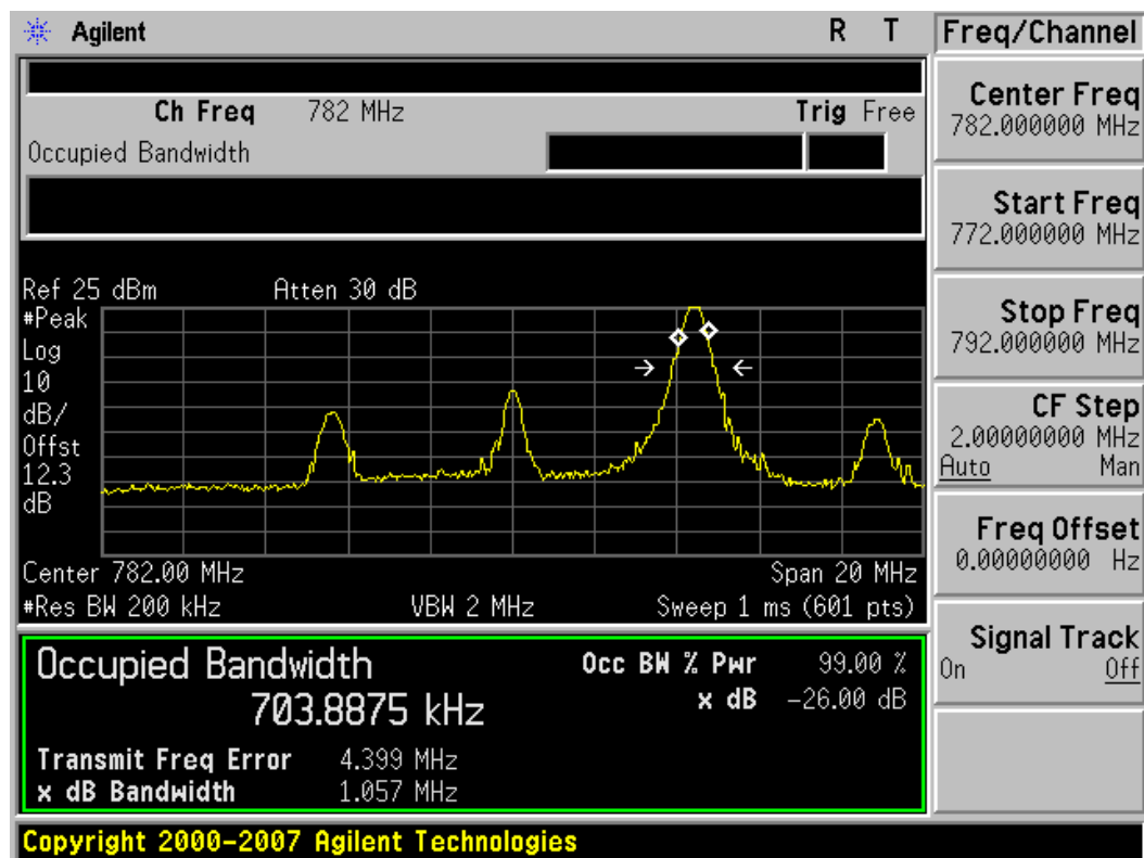
Plot 7-9. Occupied Bandwidth Plot (16QAM – RB Size 1, RB Offset 49)
