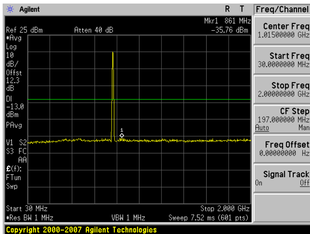
Plot 7-21. Conducted Spurious Plot (16QAM – RB Size 50)
