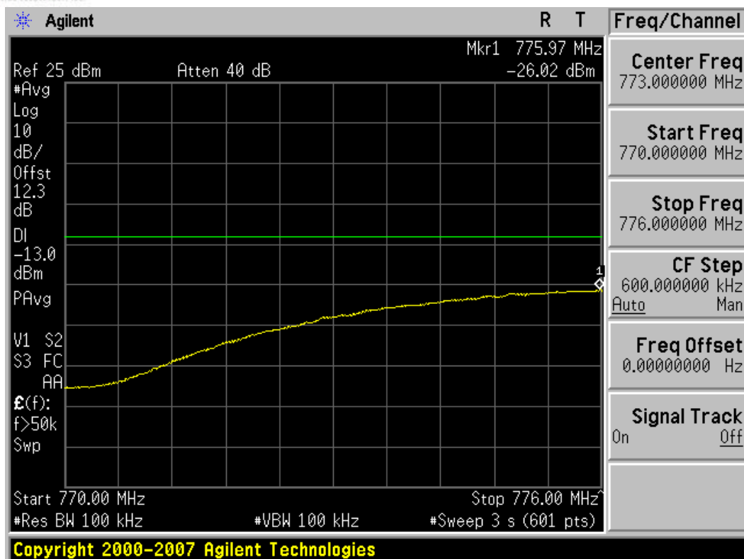
Plot 7-3. Lower Band Edge Plot (16QAM – RB Size 50)
