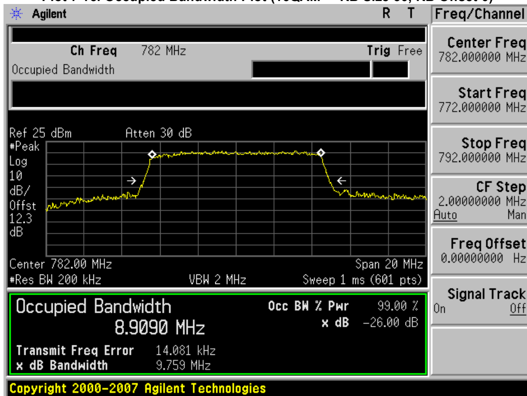
Plot 7-16. Occupied Bandwidth Plot (QPSK – RB Size 50, RB Offset 0)
