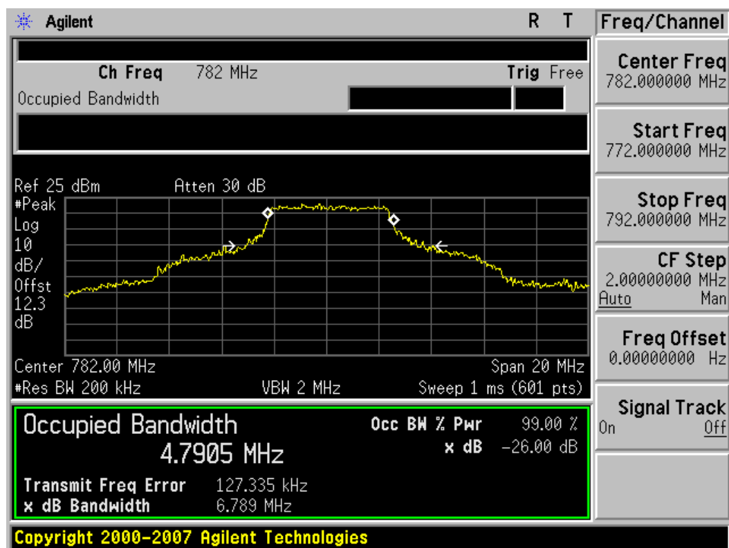
Plot 7-13. Occupied Bandwidth Plot (16QAM – RB Size 25, RB Offset 13)
