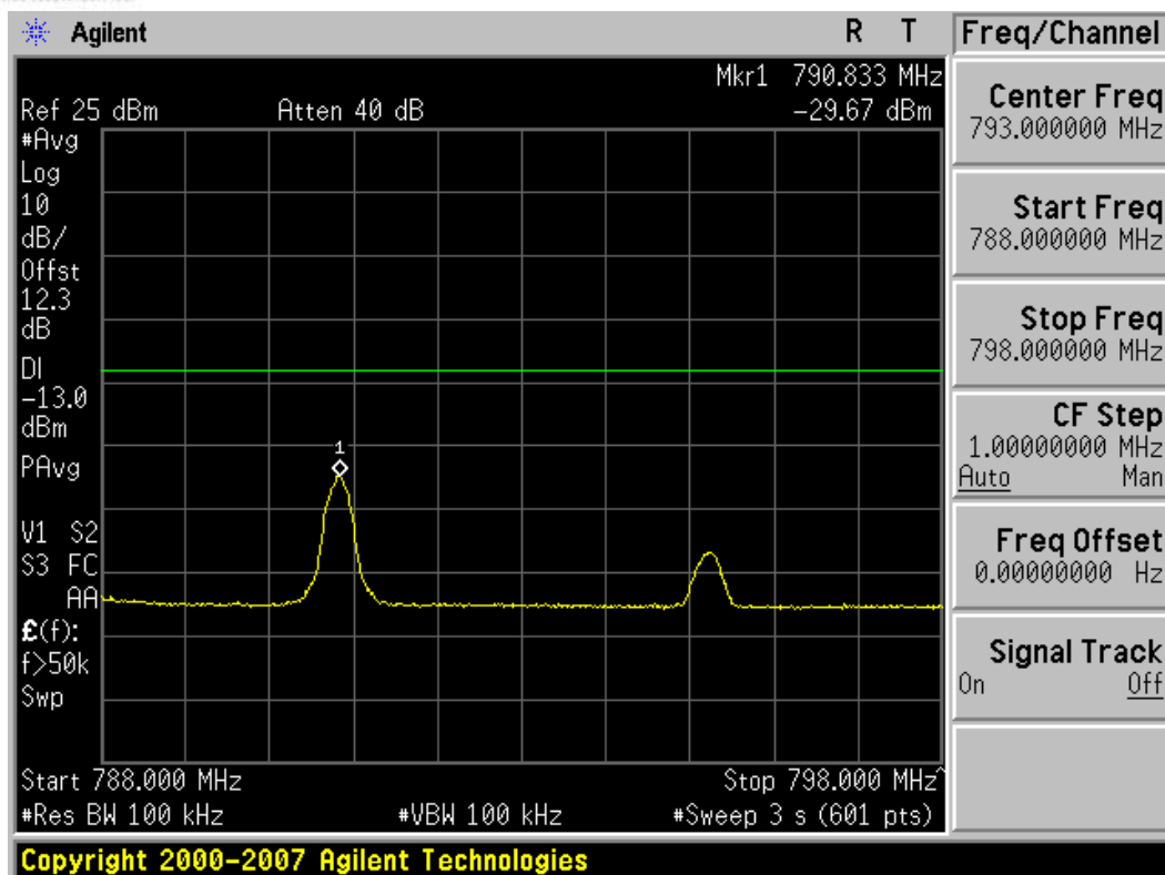
Plot 7-25. Upper Band Edge Plot (16QAM – RB Size 1)
