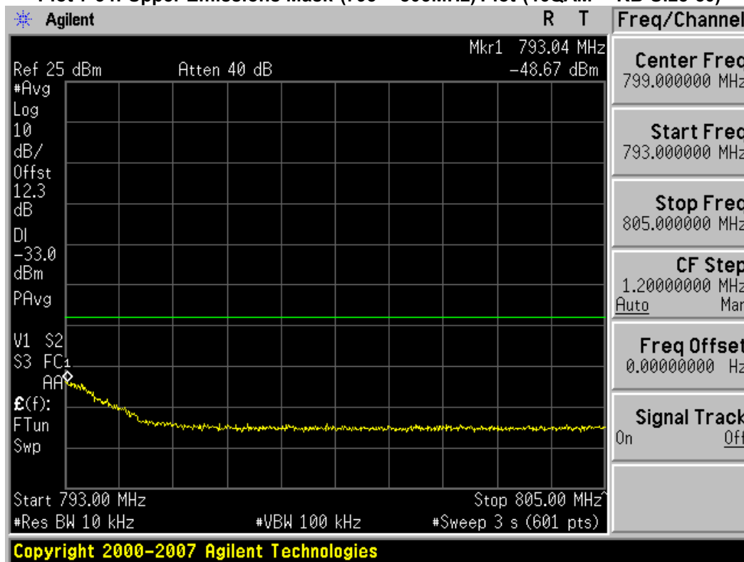
Plot 7-32. Upper Emissions Mask (793 – 805MHz) Plot (QPSK – RB Size 50)
