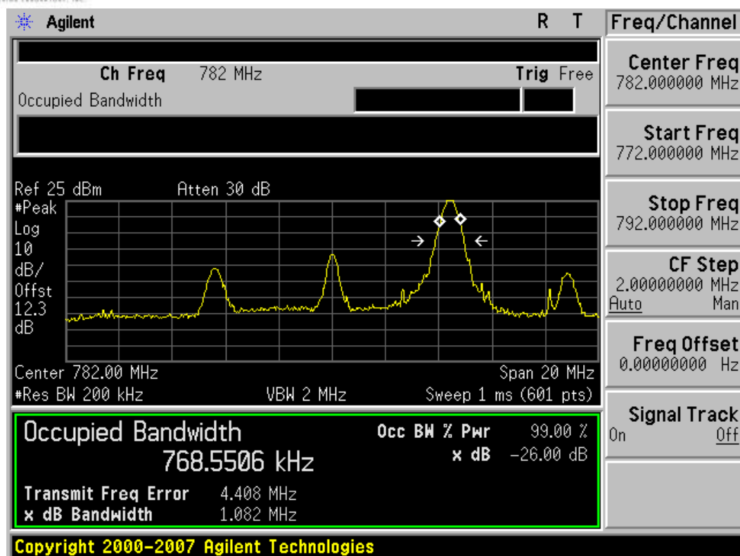
Plot 7-10. Occupied Bandwidth Plot (QPSK – RB Size 1, RB Offset 49)
