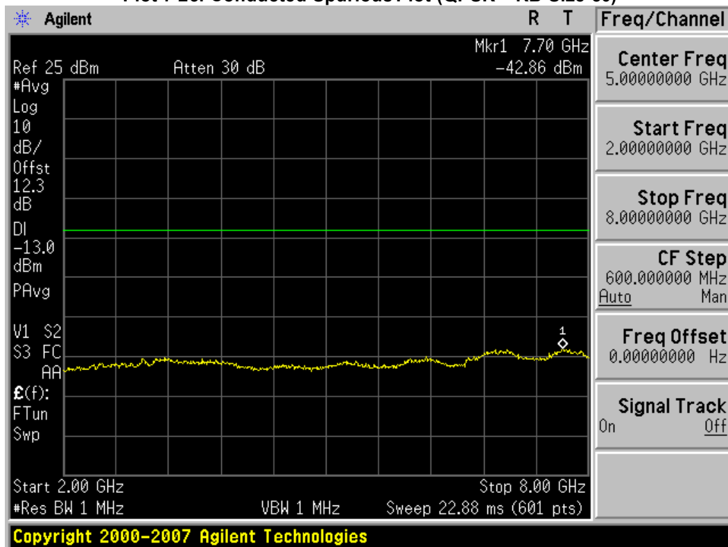
Plot 7-24. Conducted Spurious Plot (QPSK – RB Size 50)
