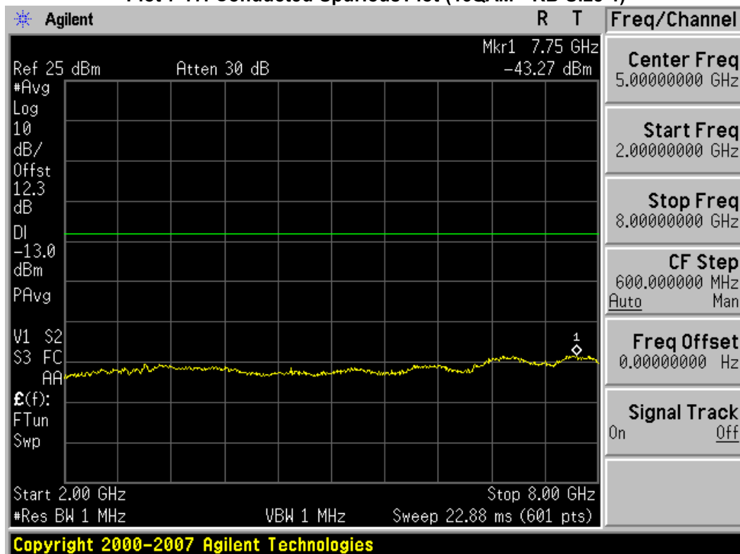
Plot 7-18. Conducted Spurious Plot (16QAM – RB Size 1)
