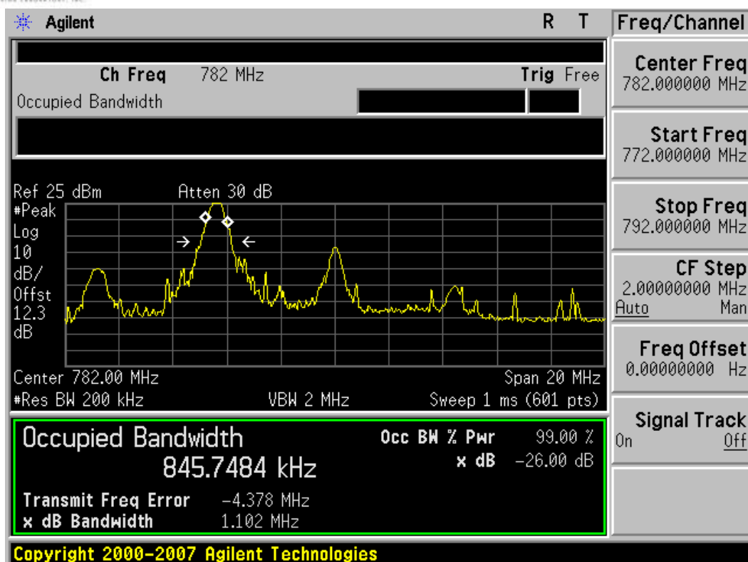
Plot 7-11. Occupied Bandwidth Plot (16QAM – RB Size 1, RB Offset 0)
