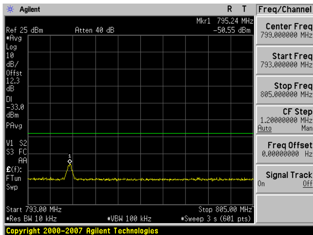
Plot 7-29. Upper Emissions Mask (793 – 805MHz) Plot (16QAM – RB Size 1)
