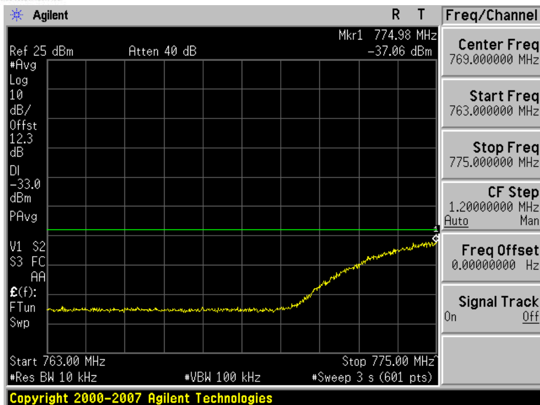
Plot 7-7. Lower Emission Mask (763 – 775MHz) Plot (16QAM – 50RB)
