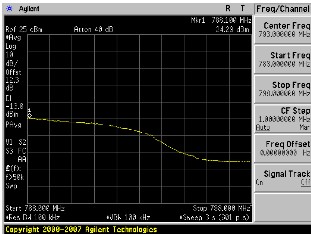
Plot 7-27. Upper Band Edge Plot (16QAM – RB Size 50)
