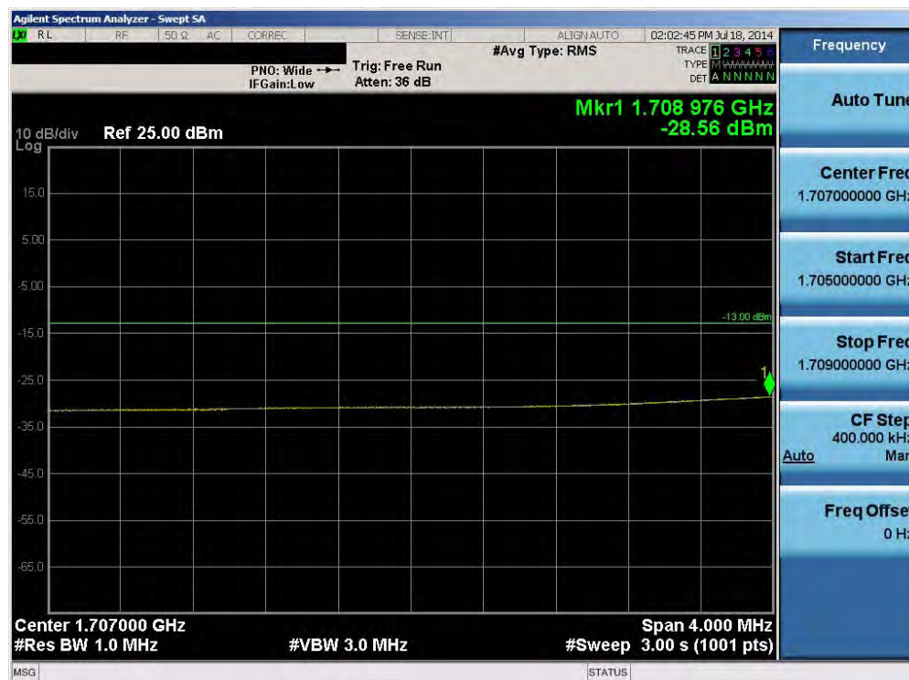
Plot 6-46. Lower Extended Band Edge Plot (Band 4 – 20.0MHz QPSK – RB Size 100)
