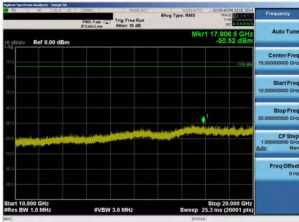
Plot 6-12. Conducted Spurious Plot (Band 4 – 15.0MHz QPSK – RB Size 1, RB Offset 0 – Low Channel)
