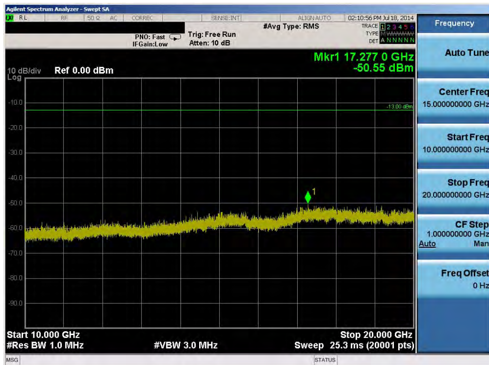
Plot 6-16. Conducted Spurious Plot (Band 4 – 15.0MHz QPSK – RB Size 1, RB Offset 0 – High Channel)
