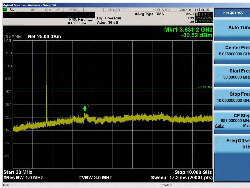
Plot 6-17. Conducted Spurious Plot (Band 4 - 20.0MHz QPSK - RB Size 1, RB Offset 0- Low Channel)
