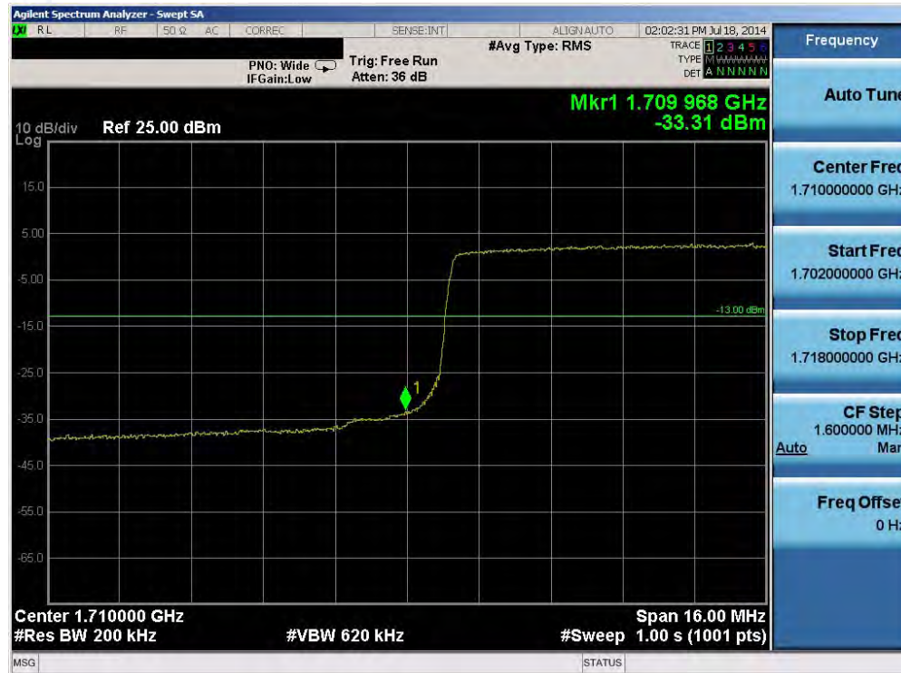
Plot 6-45. Lower Band Edge Plot (Band 4 – 20.0MHz QPSK – RB Size 100)
