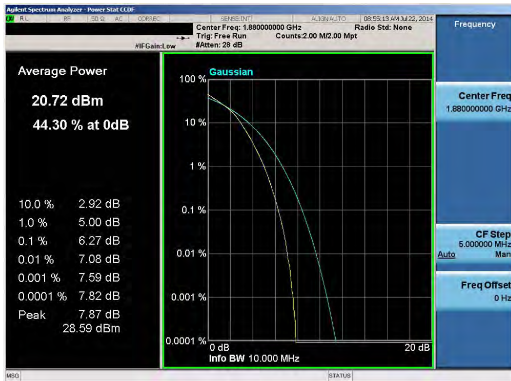
Plot 6-62. PAR Plot (Band 2 – 10.0MHz 16-QAM – RB Size 50)
