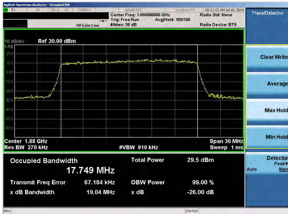
Plot 6-10. Occupied Bandwidth Plot (Band 2 – 20.0MHz 16-QAM – RB Size 100)
