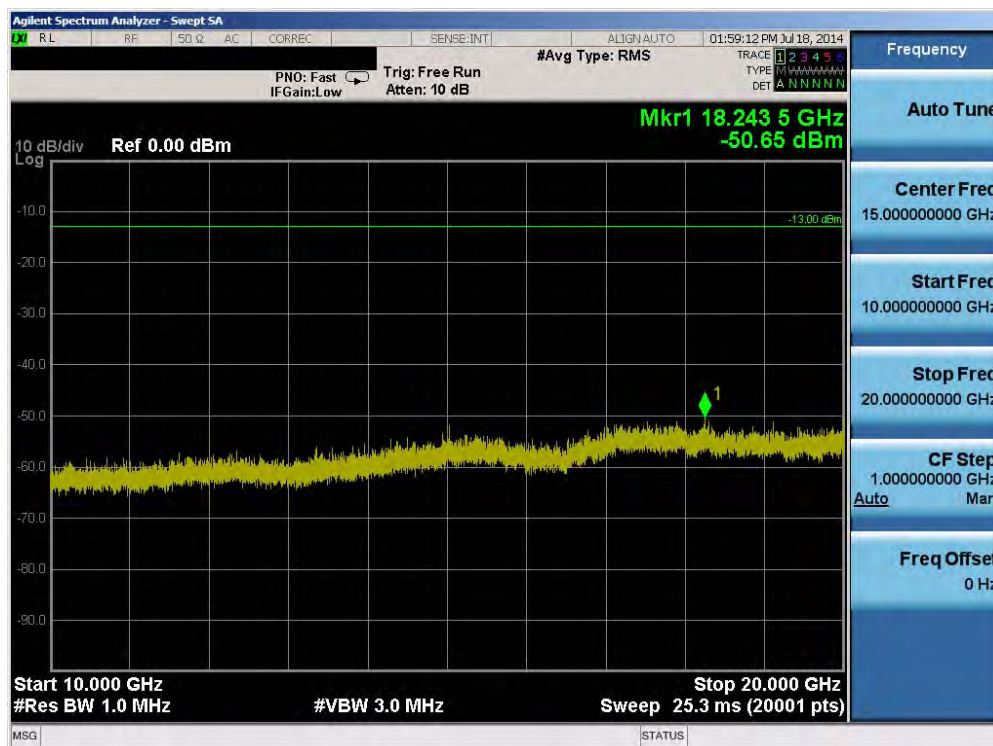
Plot 6-20. Conducted Spurious Plot (Band 4 - 20.0MHz QPSK - RB Size 1, RB Offset 0 - Mid Channel)
