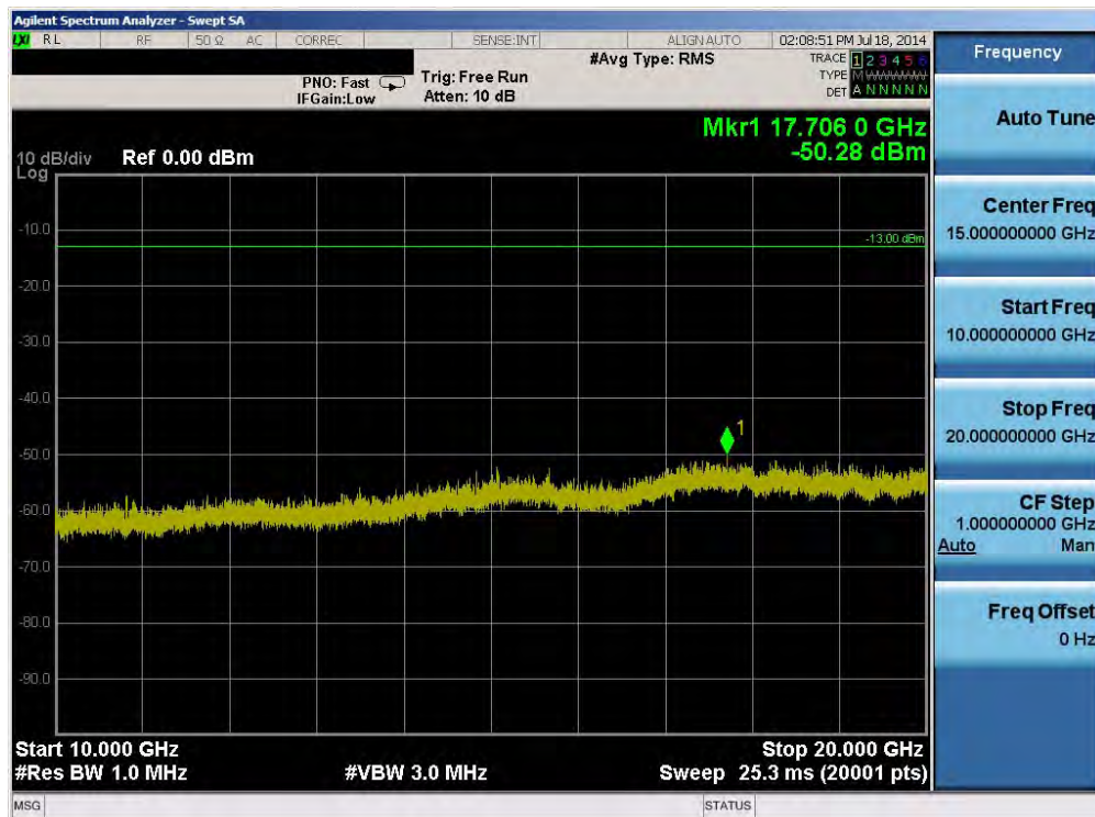
Plot 6-14. Conducted Spurious Plot (Band 4 – 15.0MHz QPSK – RB Size 1, RB Offset 0 – Mid Channel)
