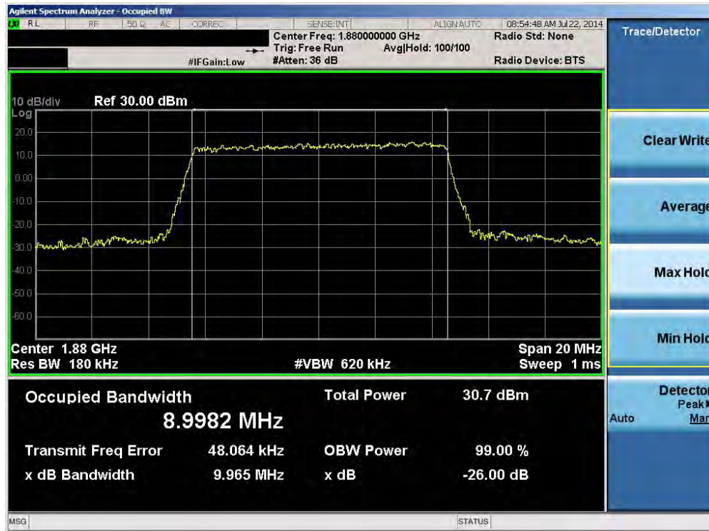
Plot 6-5. Occupied Bandwidth Plot (Band 2 – 10.0MHz QPSK – RB Size 50)
