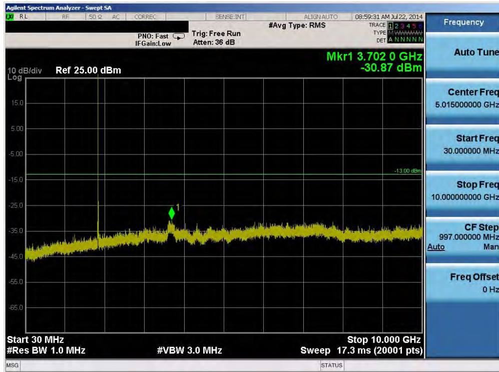
Plot 6-23. Conducted Spurious Plot (Band 2 - 10.0MHz QPSK - RB Size 1, RB Offset 0- Low Channel)
