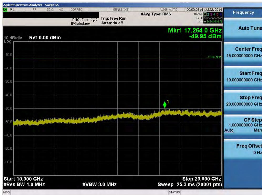
Plot 6-24. Conducted Spurious Plot (Band 2 - 10.0MHz QPSK - RB Size 1, RB Offset 0 - Low Channel)
