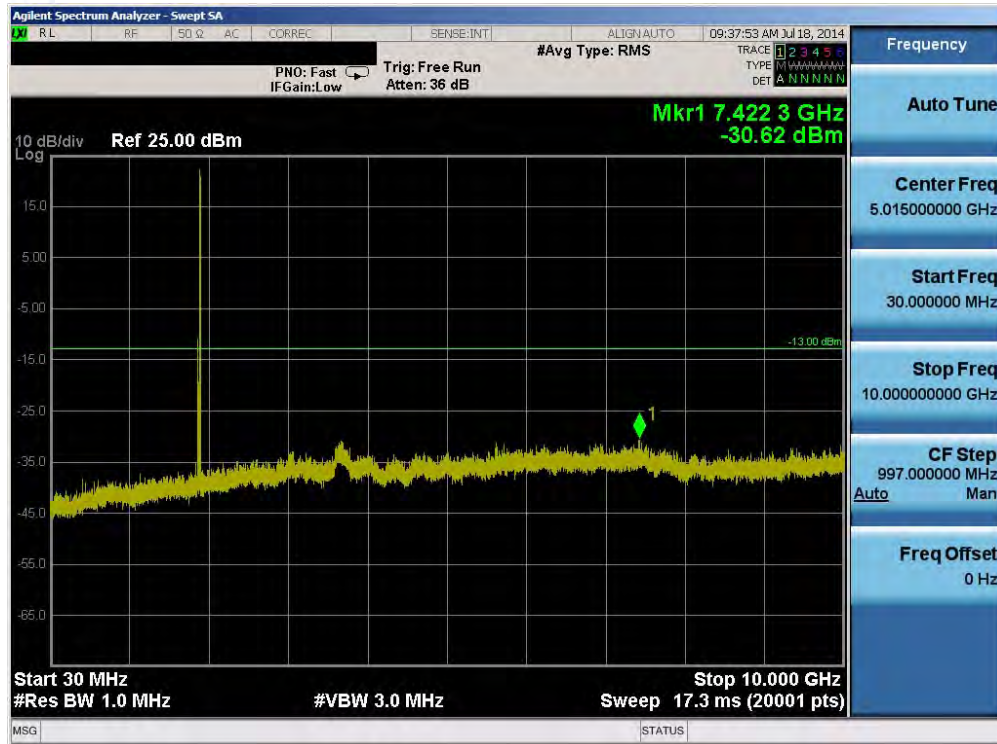
Plot 6-33. Conducted Spurious Plot (Band 2 – 15.0MHz QPSK – RB Size 1, RB Offset 0 – High Channel)
