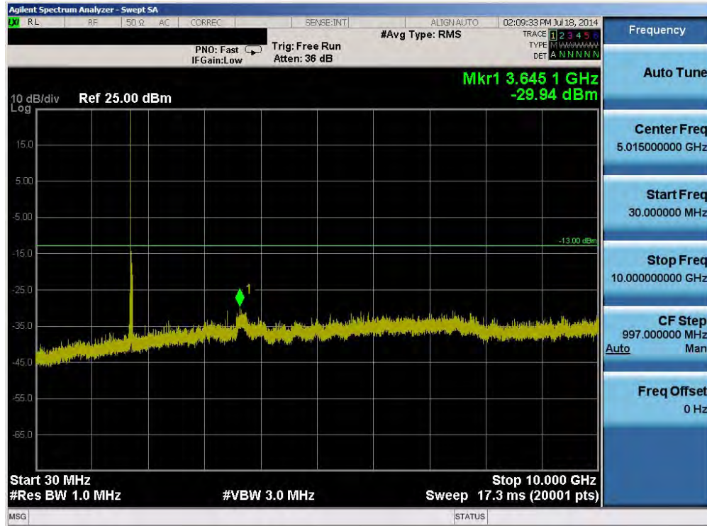
Plot 6-11. Conducted Spurious Plot (Band 4 – 15.0MHz QPSK – RB Size 1, RB Offset 0 – Low Channel)
