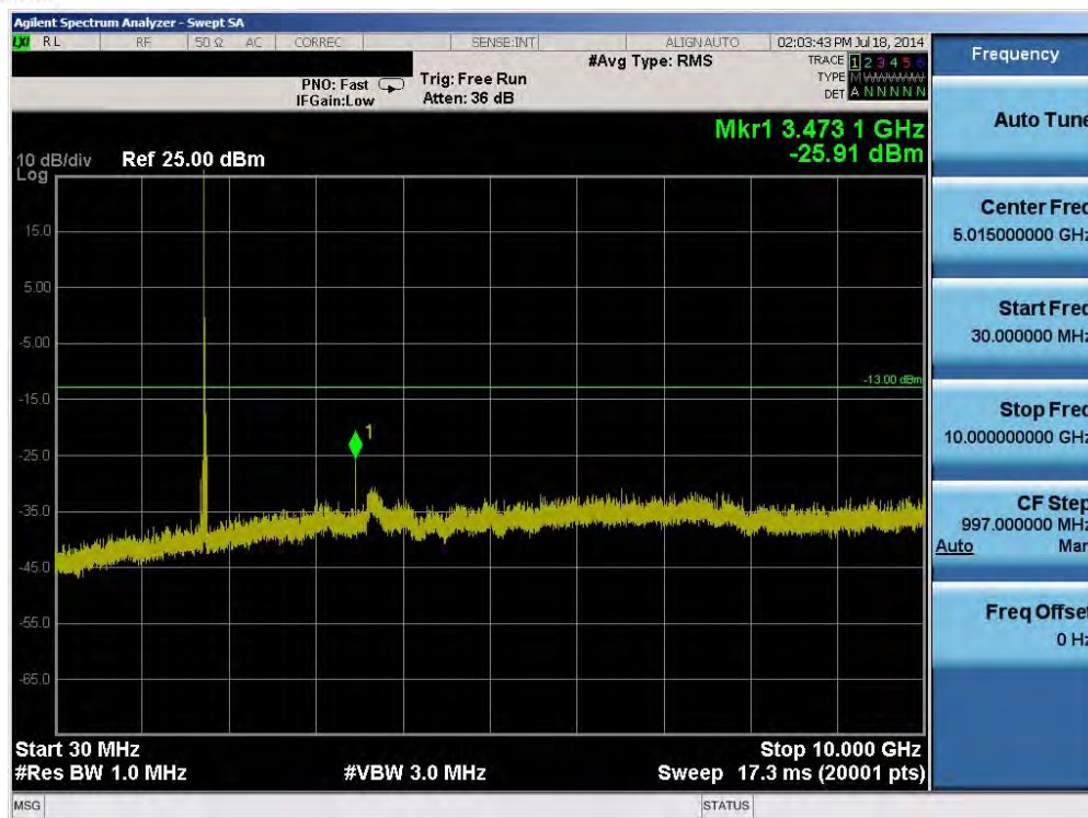
Plot 6-21. Conducted Spurious Plot (Band 4 – 20.0MHz QPSK – RB Size 1, RB Offset 0 – High Channel)
