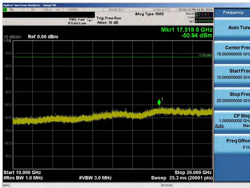
Plot 6-18. Conducted Spurious Plot (Band 4 - 20.0MHz QPSK - RB Size 1, RB Offset 0 - Low Channel)
