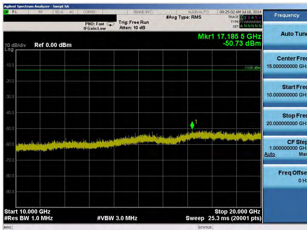
Plot 6-40. Conducted Spurious Plot (Band 2 – 20.0MHz QPSK – RB Size 1, RB Offset 0 – High Channel)
