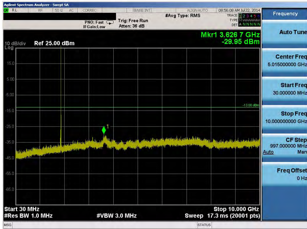
Plot 6-25. Conducted Spurious Plot (Band 2 – 10.0MHz QPSK – RB Size 1, RB Offset 0 – Mid Channel)
