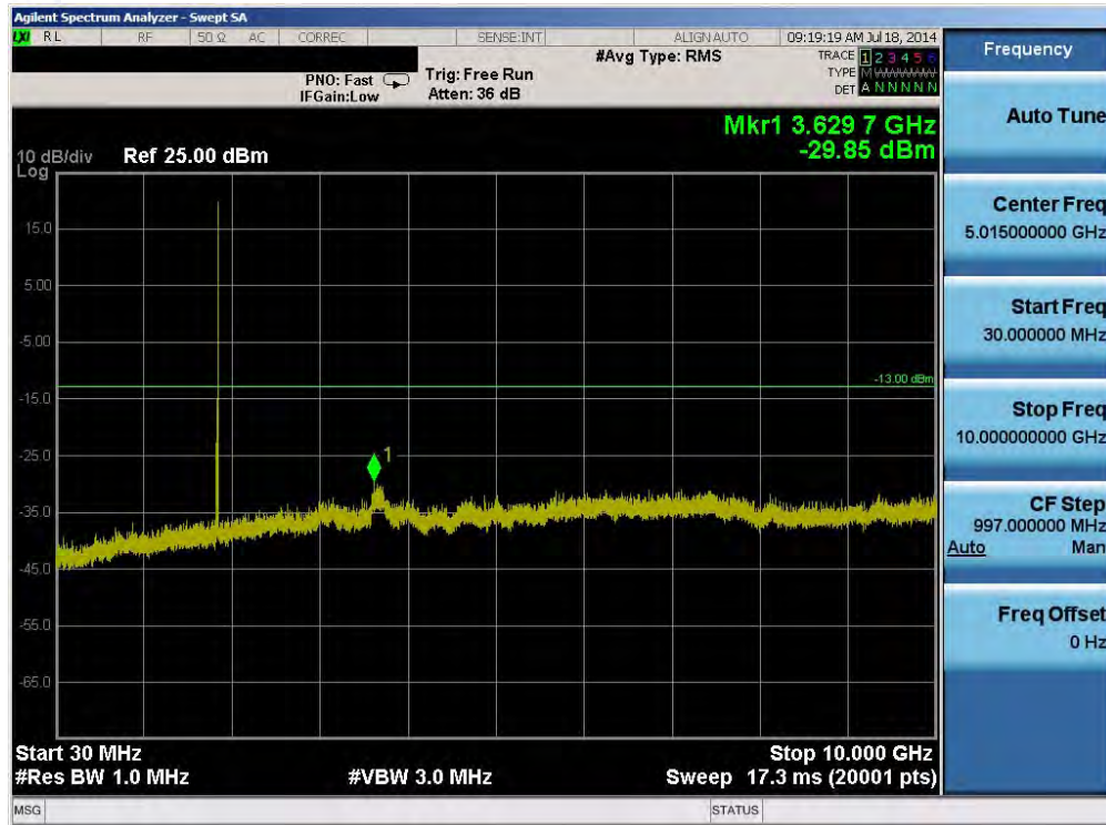
Plot 6-35. Conducted Spurious Plot (Band 2 – 20.0MHz QPSK – RB Size 1, RB Offset 0– Low Channel)
