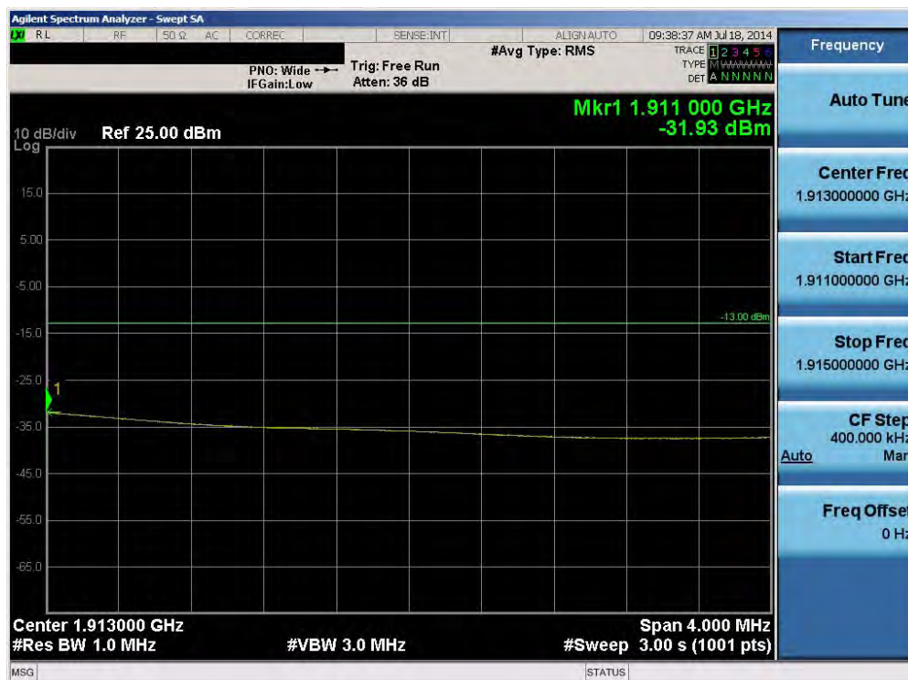
Plot 6-56. Upper Extended Band Edge Plot (Band 2 – 15.0MHz QPSK – RB Size 75)
