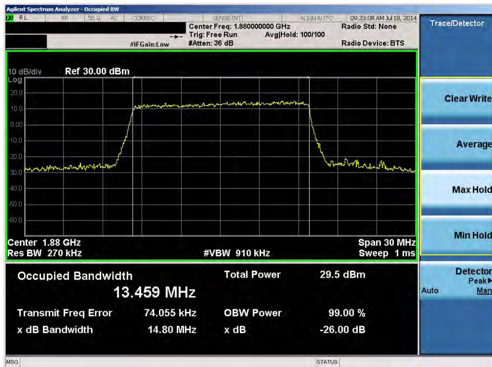
Plot 6-8. Occupied Bandwidth Plot (Band 2 – 15.0MHz 16-QAM – RB Size 75)
