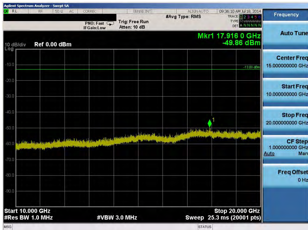
Plot 6-30. Conducted Spurious Plot (Band 2 – 15.0MHz QPSK – RB Size 1, RB Offset 0 – Low Channel)
