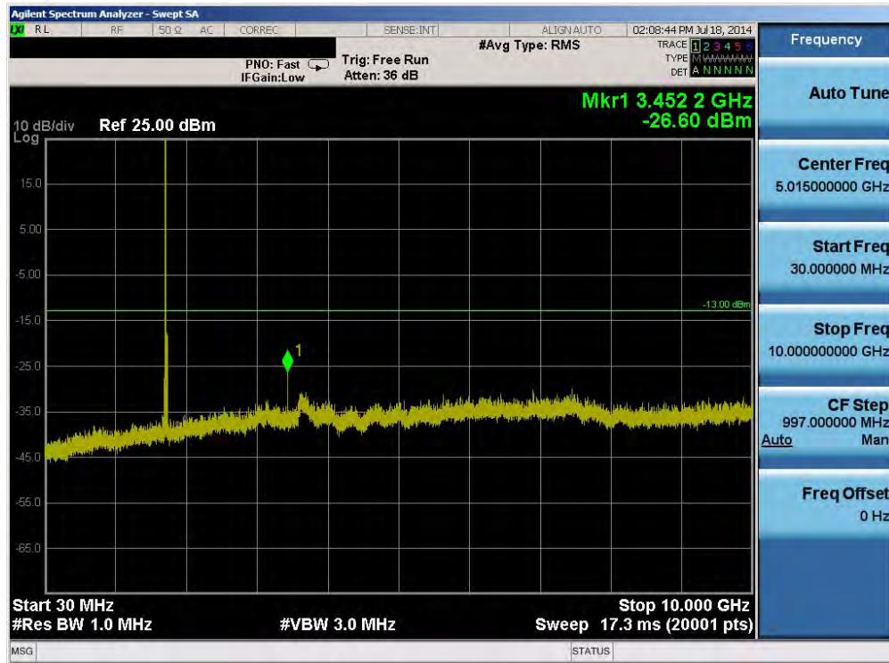
Plot 6-13. Conducted Spurious Plot (Band 4 – 15.0MHz QPSK – RB Size 1, RB Offset 0 – Mid Channel)
