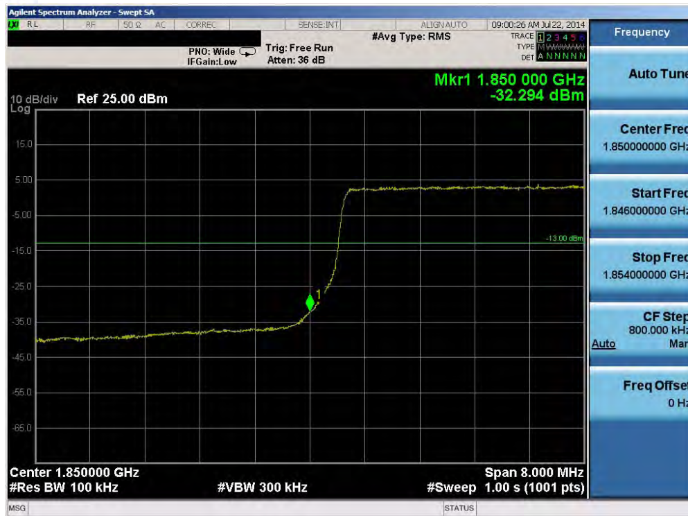
Plot 6-49. Lower Band Edge Plot (Band 2 – 10.0MHz QPSK – RB Size 50)
