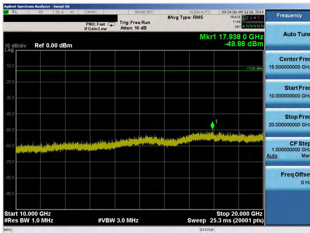
Plot 6-32. Conducted Spurious Plot (Band 2 – 15.0MHz QPSK – RB Size 1, RB Offset 0 – Mid Channel)
