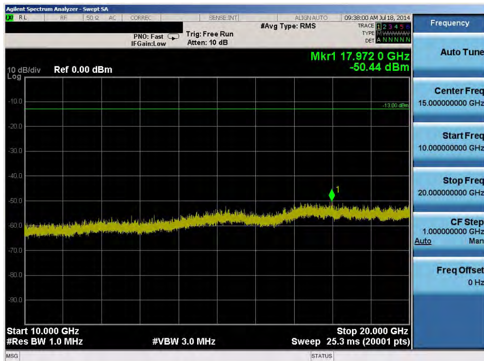
Plot 6-34. Conducted Spurious Plot (Band 2 – 15.0MHz QPSK – RB Size 1, RB Offset 0 – High Channel)
