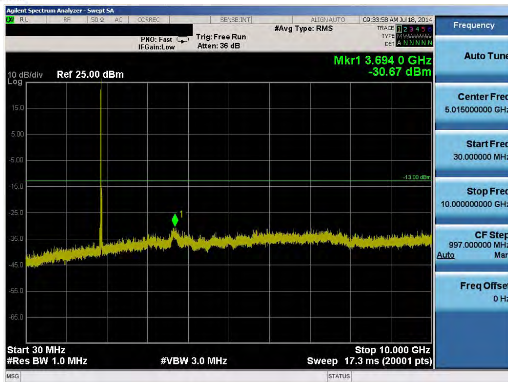
Plot 6-31. Conducted Spurious Plot (Band 2 – 15.0MHz QPSK – RB Size 1, RB Offset 0 – Mid Channel)
