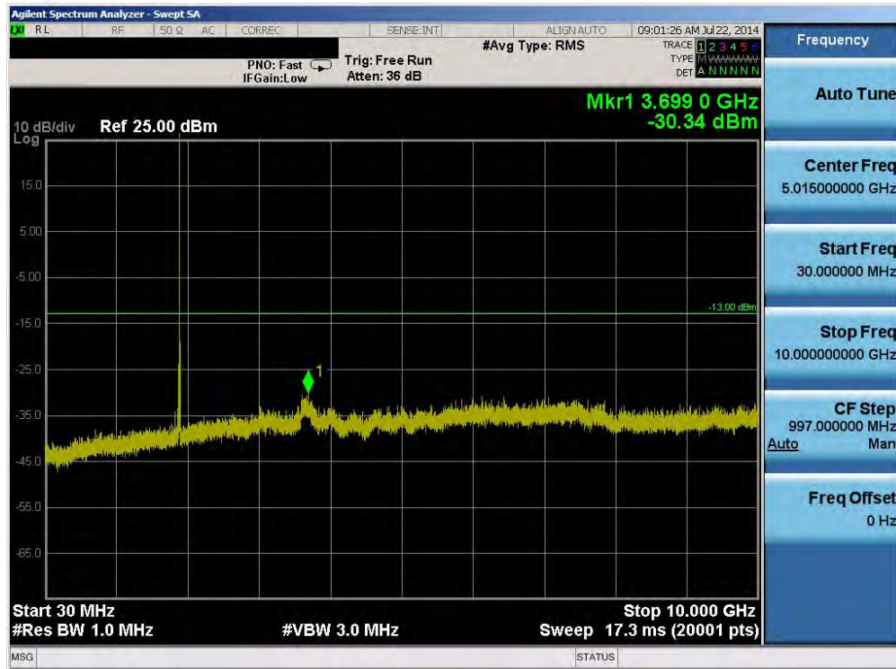
Plot 6-27. Conducted Spurious Plot (Band 2 – 10.0MHz QPSK – RB Size 1, RB Offset 0 – High Channel)
