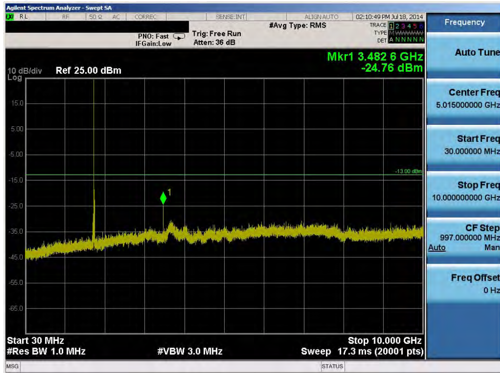
Plot 6-15. Conducted Spurious Plot (Band 4 – 15.0MHz QPSK – RB Size 1, RB Offset 0 – High Channel)
