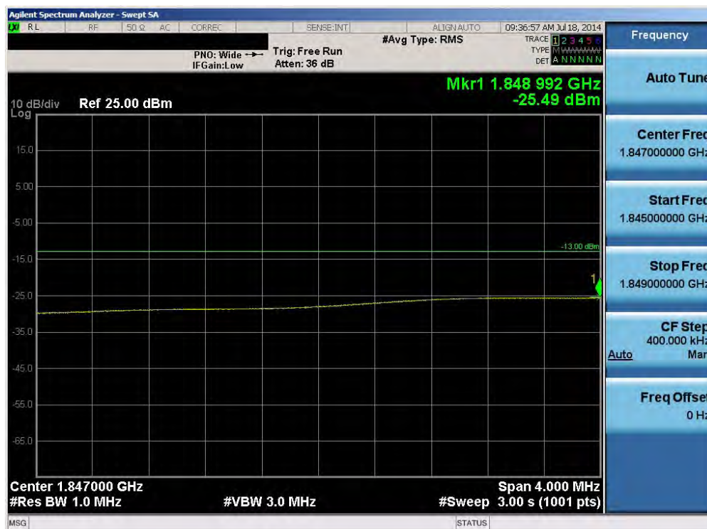
Plot 6-54. Lower Extended Band Edge Plot (Band 2 – 15.0MHz QPSK – RB Size 75)
