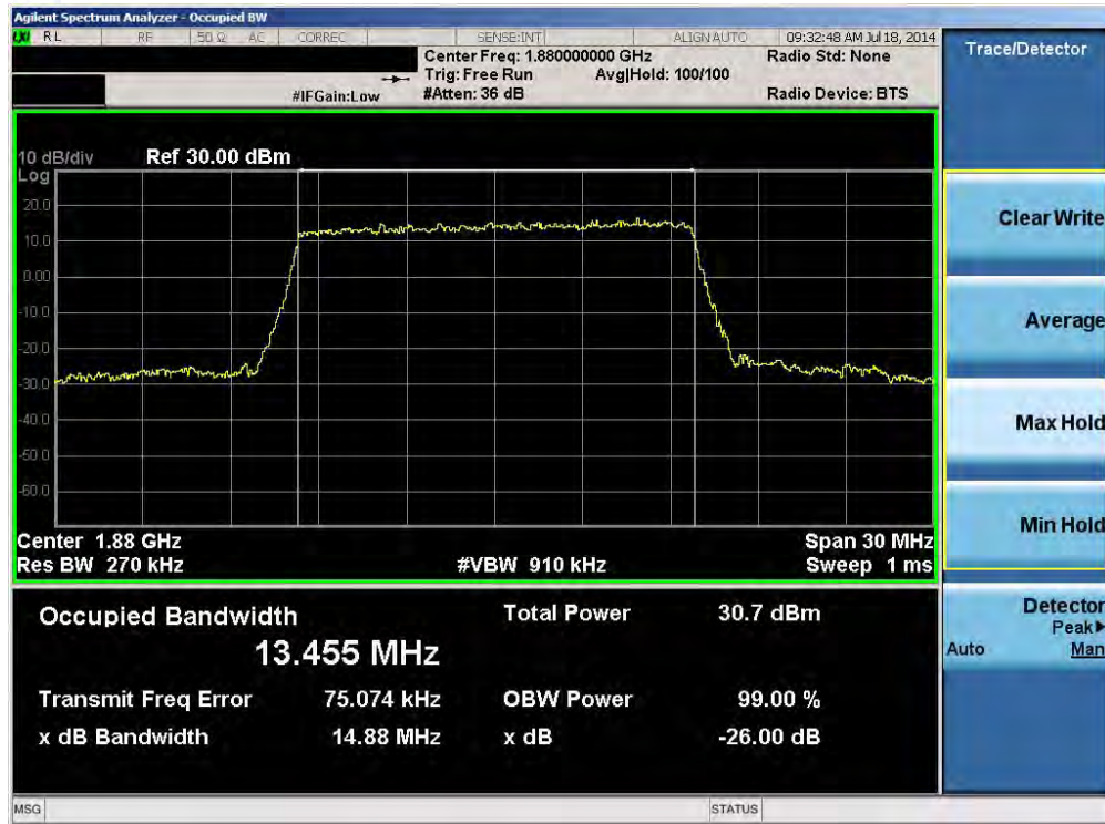
Plot 6-7. Occupied Bandwidth Plot (Band 2 – 15.0MHz QPSK – RB Size 75)
