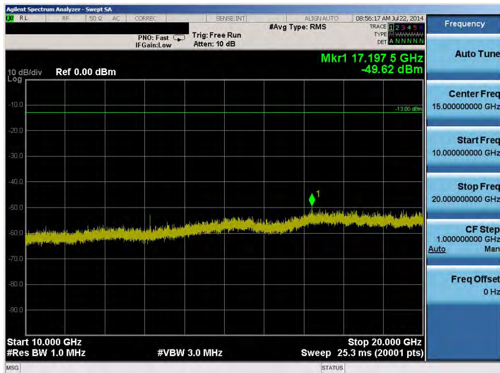
Plot 6-26. Conducted Spurious Plot (Band 2 – 10.0MHz QPSK – RB Size 1, RB Offset 0 – Mid Channel)
