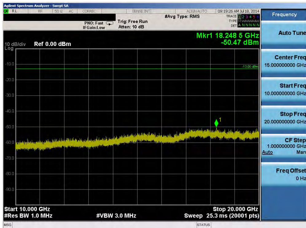
Plot 6-36. Conducted Spurious Plot (Band 2 – 20.0MHz QPSK – RB Size 1, RB Offset 0 – Low Channel)
