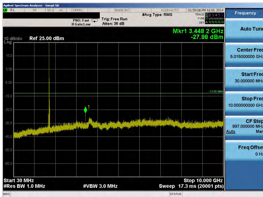
Plot 6-19. Conducted Spurious Plot (Band 4 - 20.0MHz QPSK - RB Size 1, RB Offset 0 - Mid Channel)
