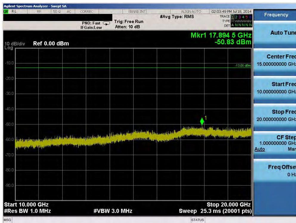
Plot 6-22. Conducted Spurious Plot (Band 4 – 20.0MHz QPSK – RB Size 1, RB Offset 0 – High Channel)
