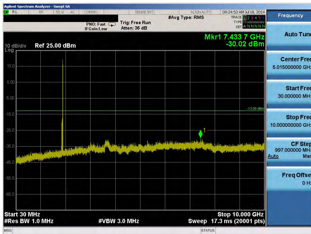
Plot 6-39. Conducted Spurious Plot (Band 2 – 20.0MHz QPSK – RB Size 1, RB Offset 0 – High Channel)
