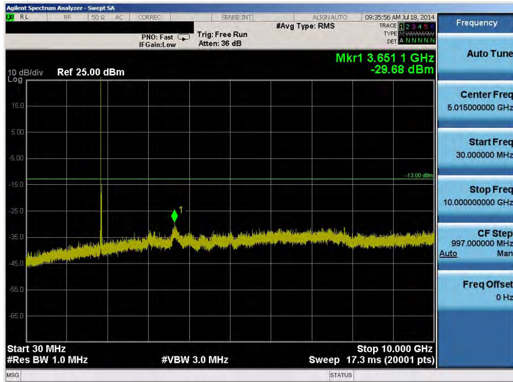
Plot 6-29. Conducted Spurious Plot (Band 2 – 15.0MHz QPSK – RB Size 1, RB Offset 0 – Low Channel)
