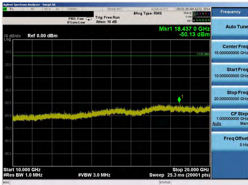
Plot 6-28. Conducted Spurious Plot (Band 2 – 10.0MHz QPSK – RB Size 1, RB Offset 0 – High Channel)
