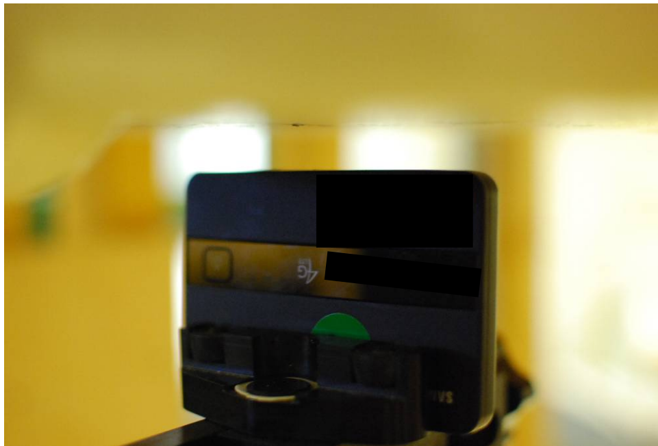
SAR Test Setup Photo 4 – Bottom at 1.0 cm
