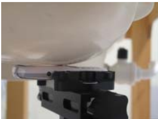
Figure 8.2 Right Head SAR Test Setup -- Cheek / Touch Position--
