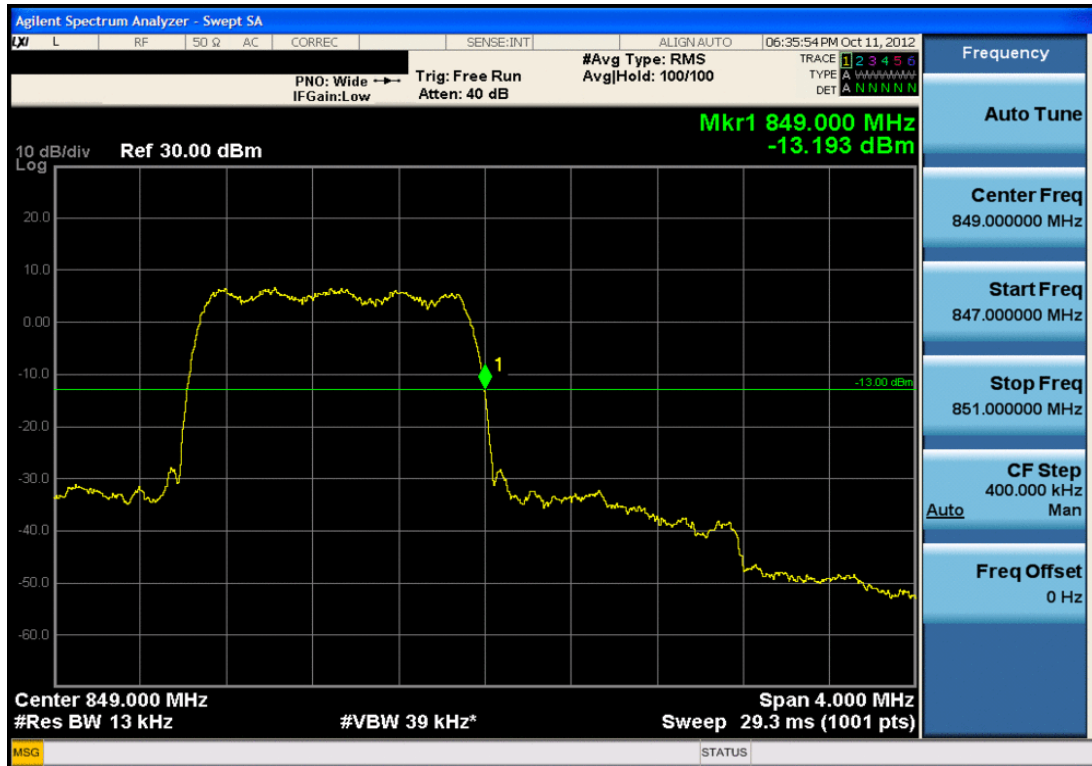
Plot 7-22. Band Edge Plot (Cellular CDMA Mode – Ch. 777)
