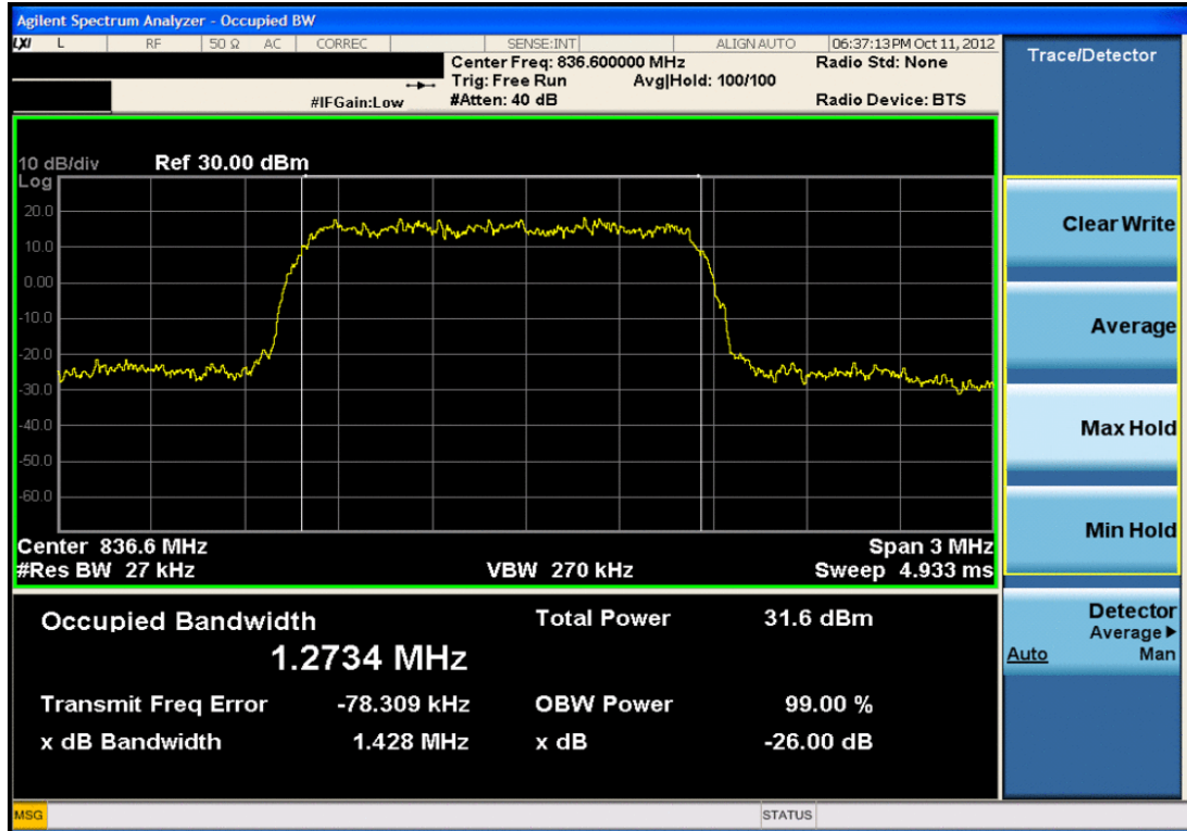
Plot 7-19. Occupied Bandwidth Plot (Cellular CDMA Mode – Ch. 384)
