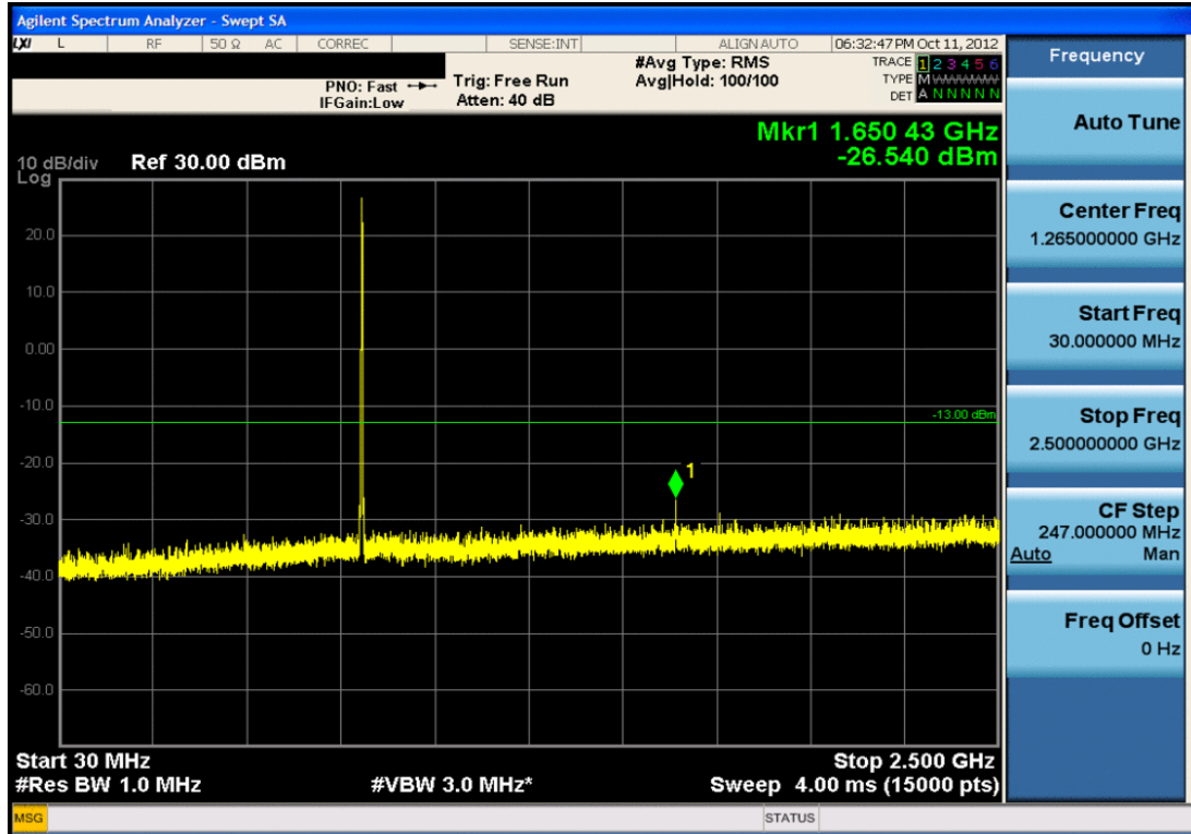
Plot 7-13. Conducted Spurious Plot (Cellular CDMA Mode – Ch. 1013)
