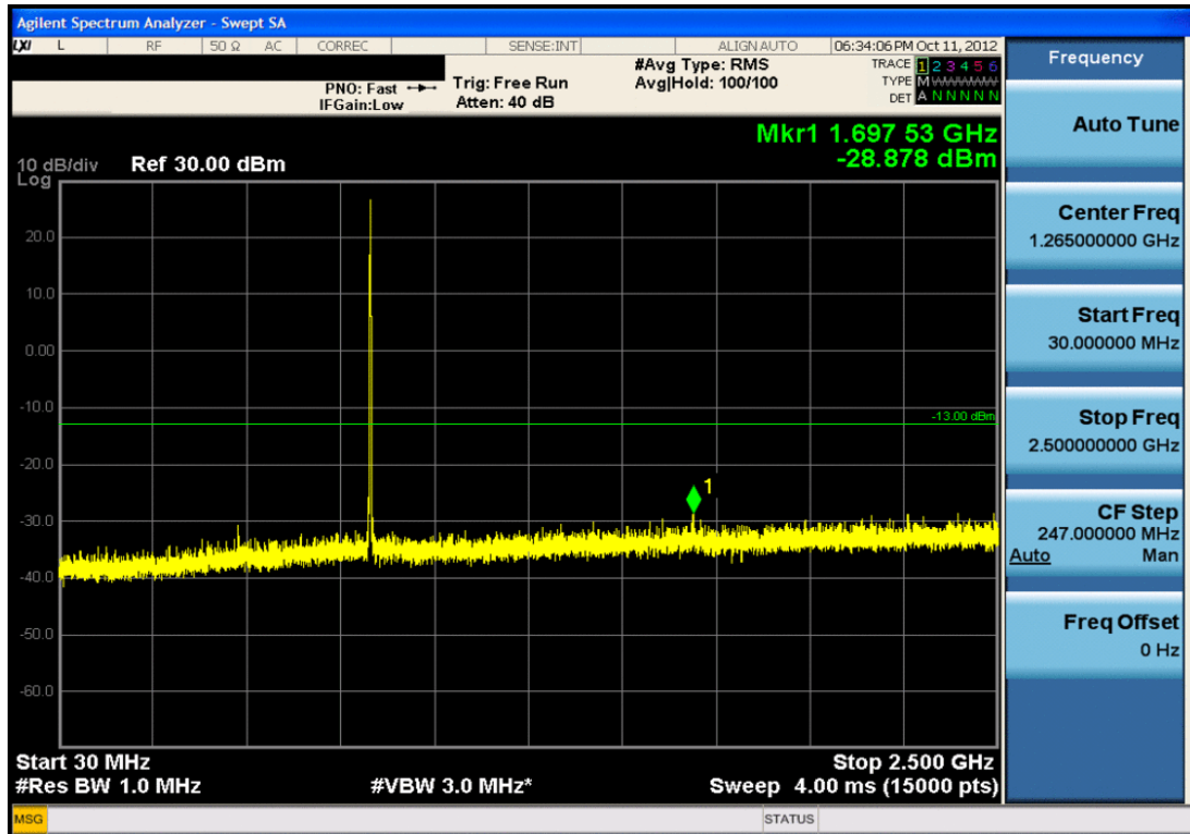
Plot 7-20. Conducted Spurious Plot (Cellular CDMA Mode – Ch. 777)
