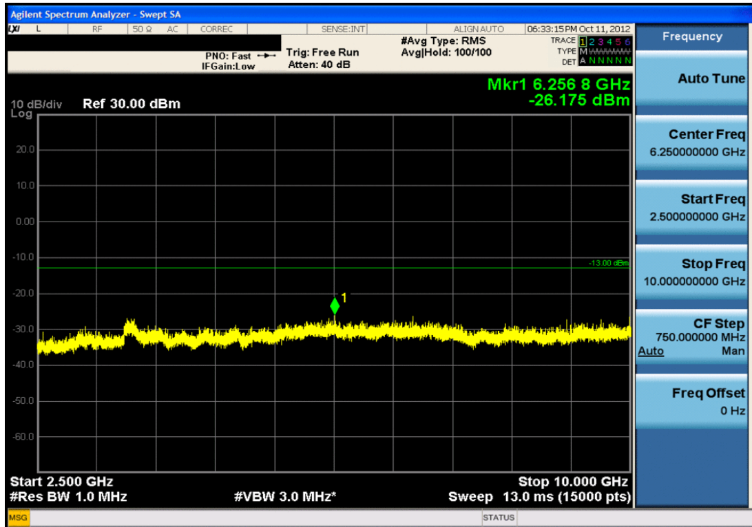
Plot 7-14. Conducted Spurious Plot (Cellular CDMA Mode – Ch. 1013)
