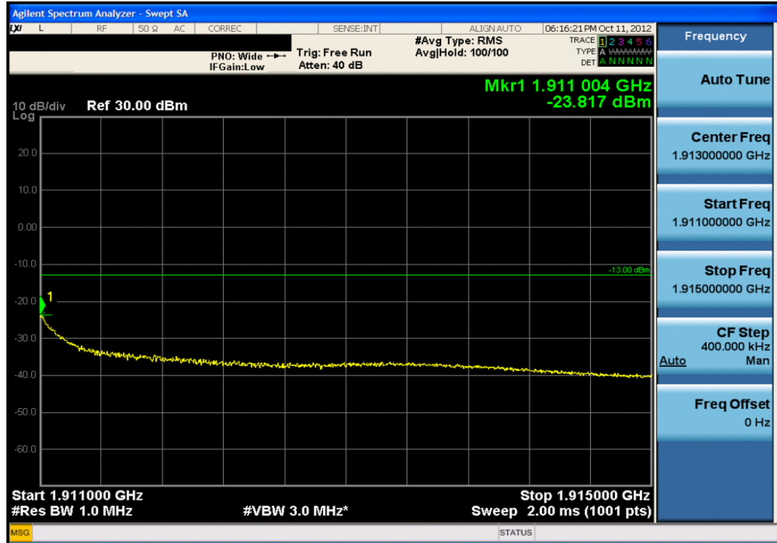
Plot 7-35. 4MHz Span Plot (PCS CDMA Mode – Ch. 1175)
