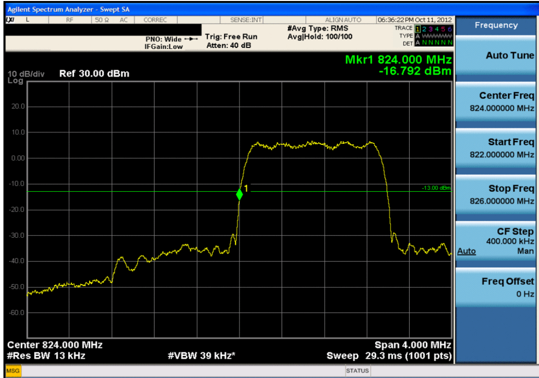
Plot 7-15. Band Edge Plot (Cellular CDMA Mode – Ch. 1013)
