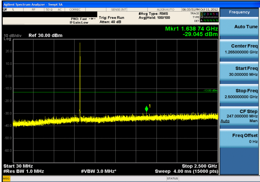
Plot 7-17. Conducted Spurious Plot (Cellular CDMA Mode – Ch. 384)
