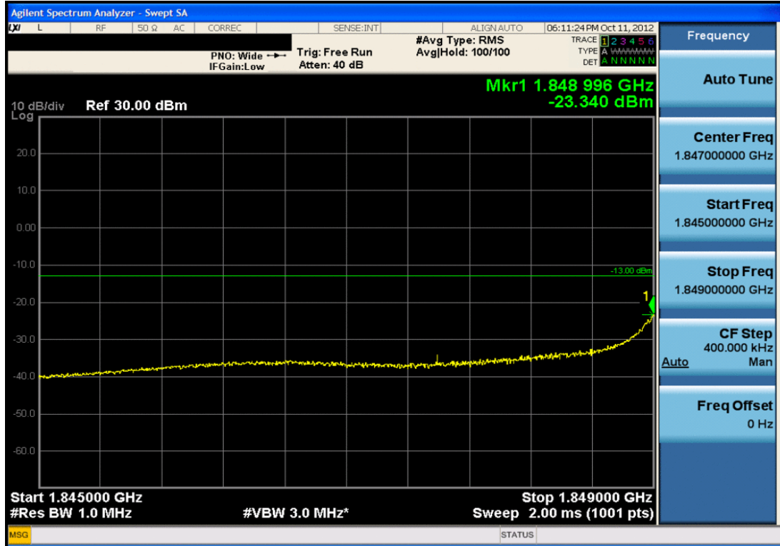
Plot 7-27. 4MHz Span Plot (PCS CDMA Mode – Ch. 25)
