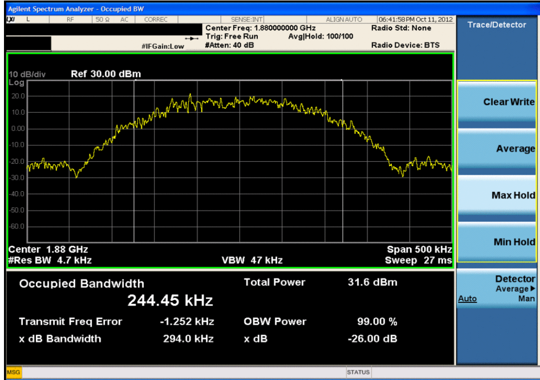
Plot 7-11. Occupied Bandwidth Plot (EDGE1900 Mode – Ch. 661)
