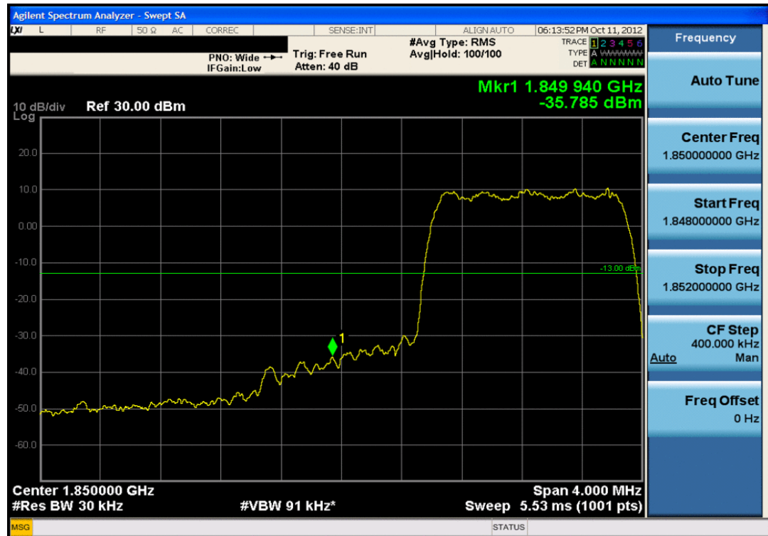
Plot 7-26. Band Edge Plot (PCS CDMA Mode – Ch. 25)
