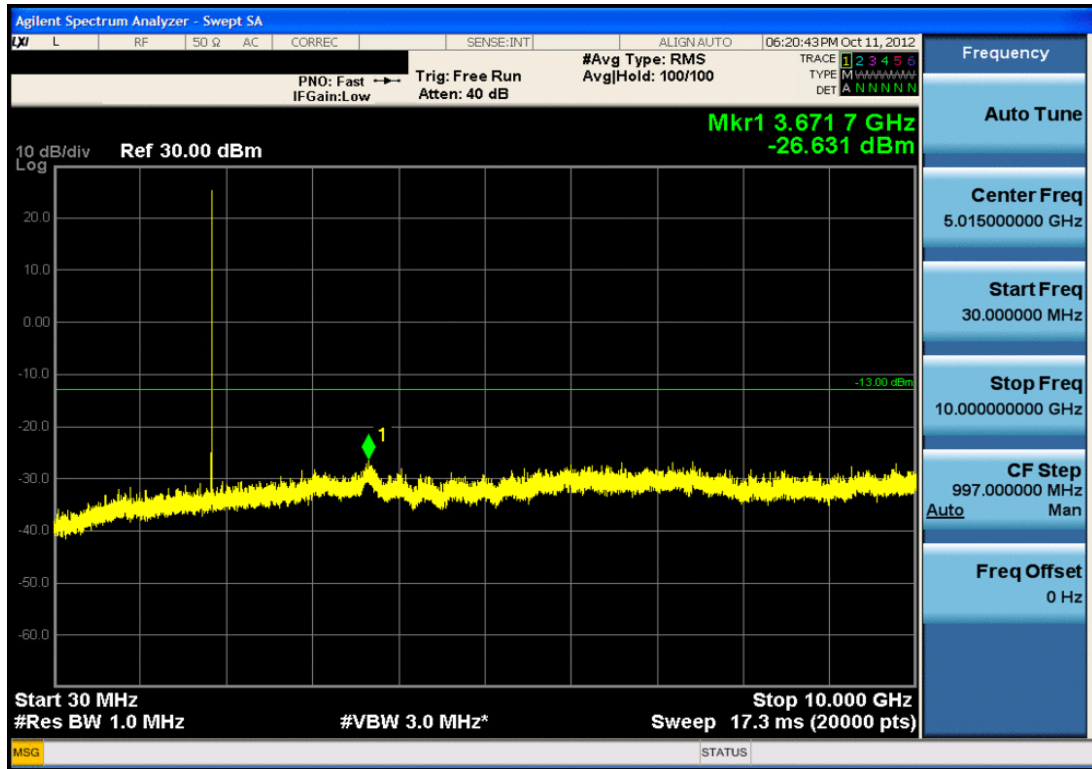
Plot 7-24. Conducted Spurious Plot (PCS CDMA Mode – Ch. 25)
