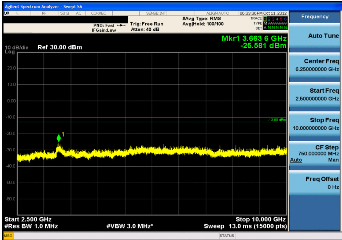
Plot 7-18. Conducted Spurious Plot (Cellular CDMA Mode – Ch. 384)
