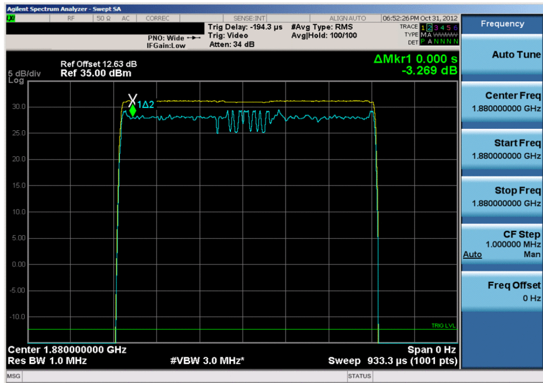
Plot 7-12. Peak-Average Ratio Plot (EDGE1900 Mode – Ch. 661)
