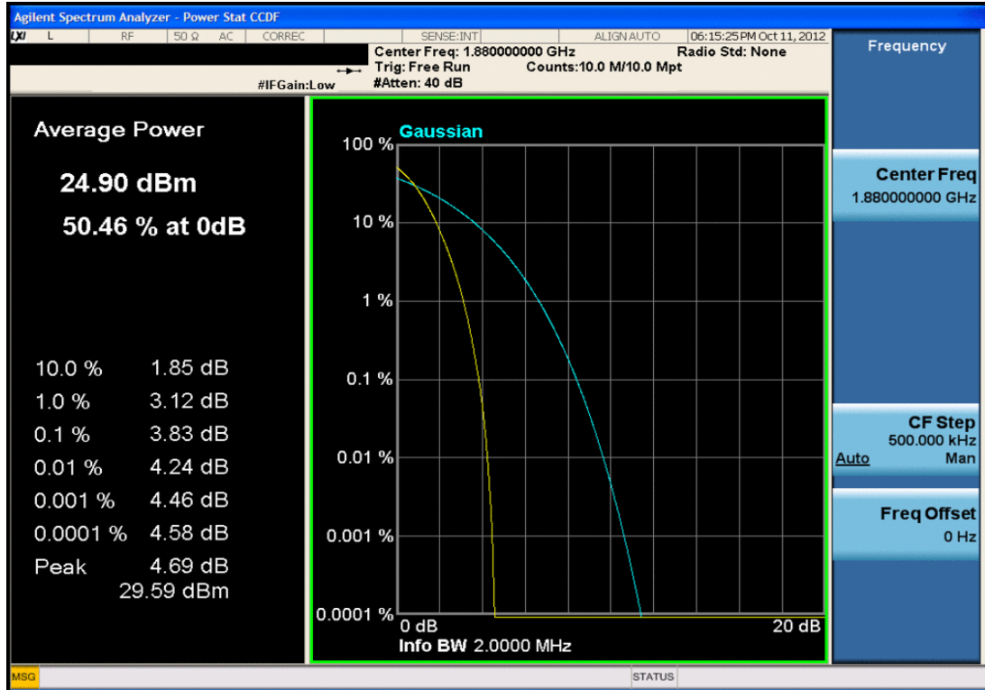
Plot 7-31. Peak-Average Ratio Plot (PCS CDMA Mode – Ch. 600)
