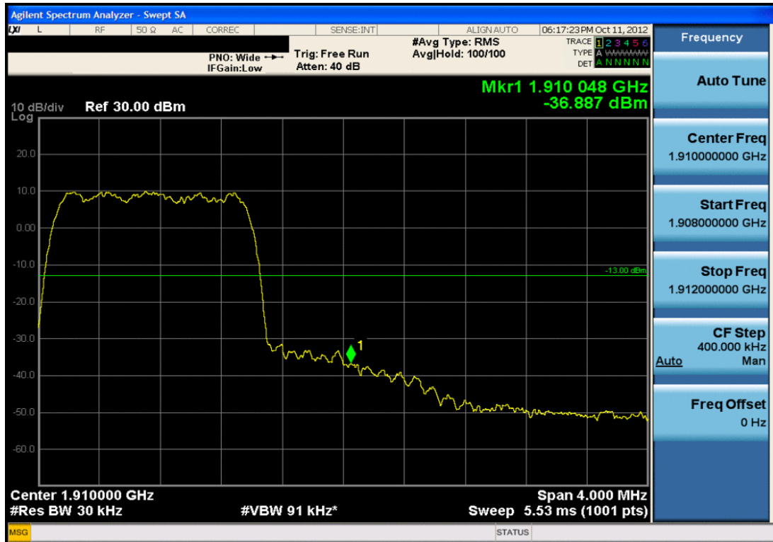
Plot 7-34. Band Edge Plot (PCS CDMA Mode – Ch. 1175)
