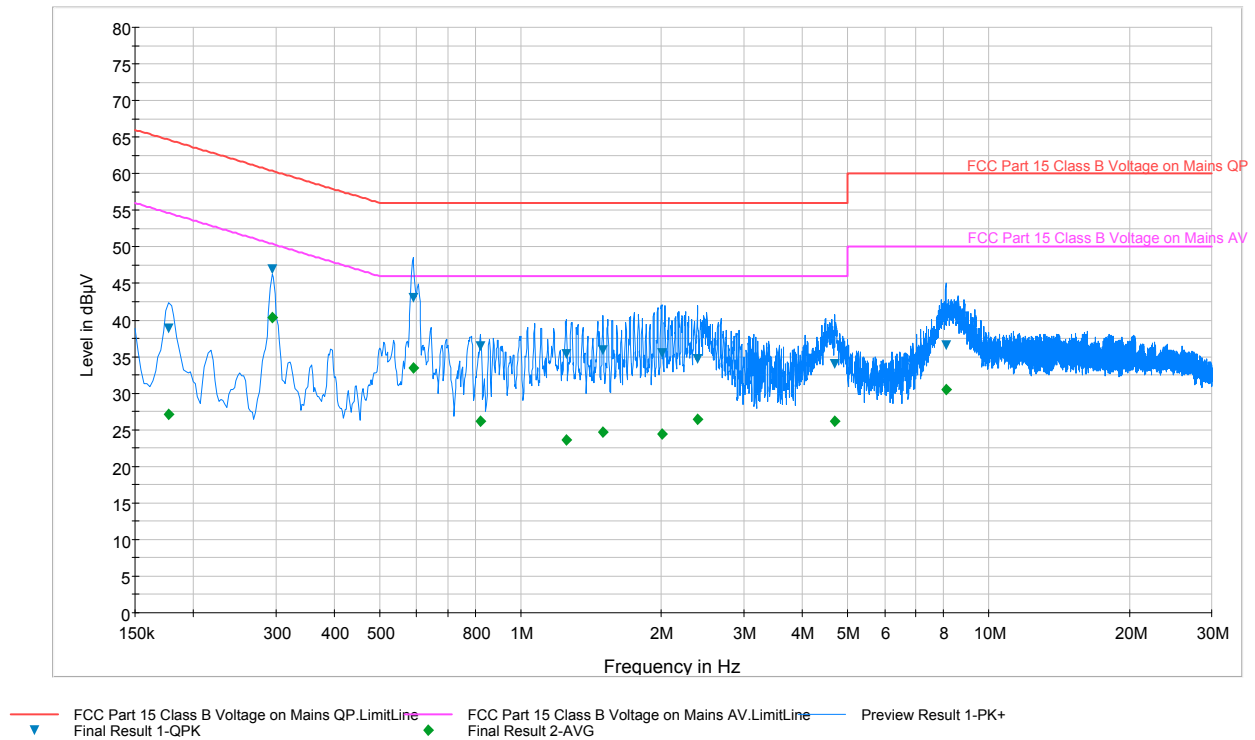
Plot 6-33. Line-Conducted Test Plot (L1)
