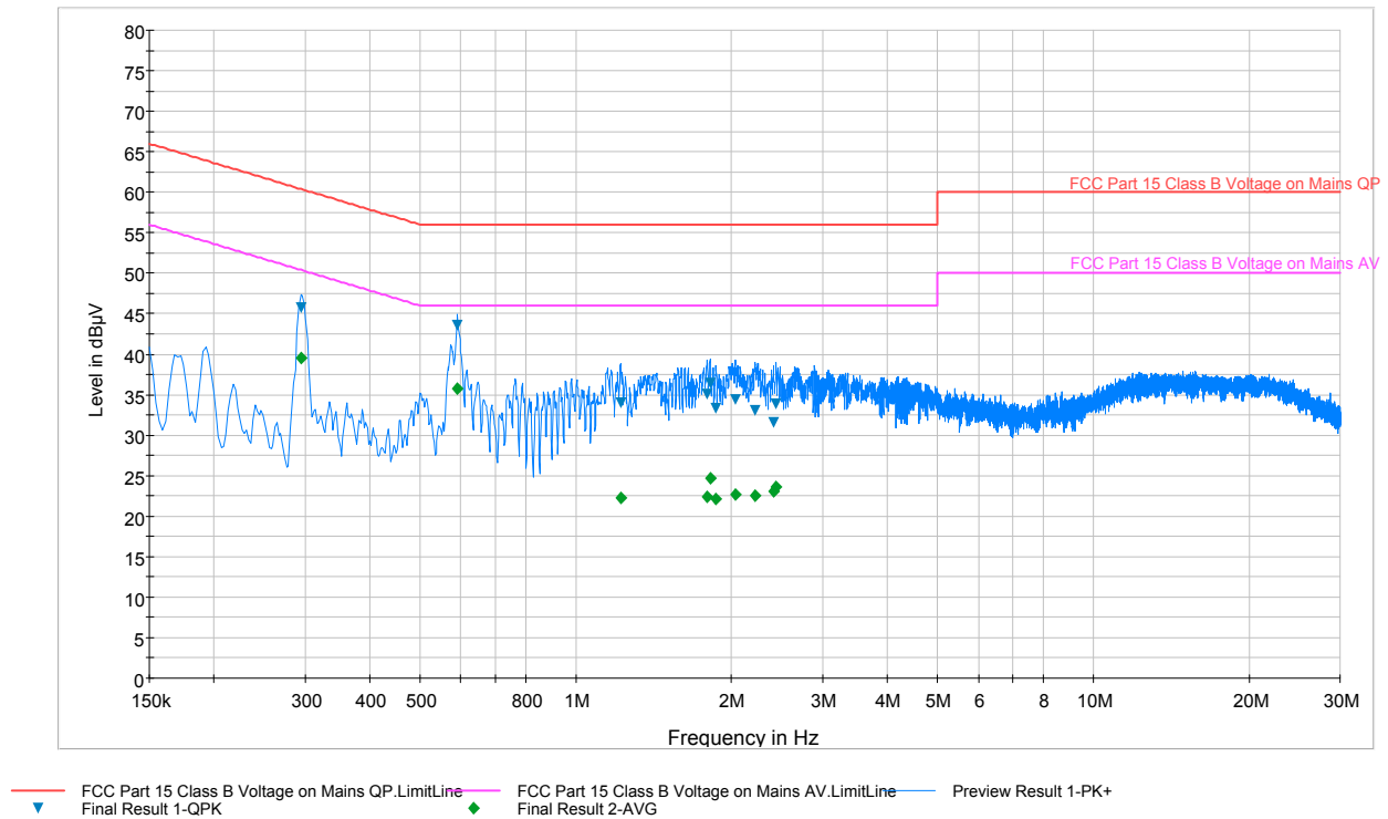
Plot 6-34. Line-Conducted Test Plot (N)
