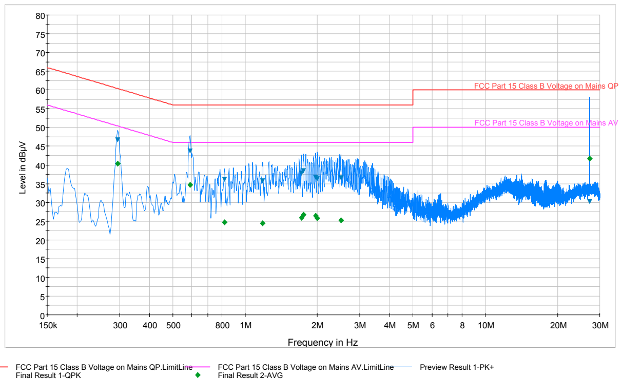
Plot 6-59. Line Conducted Plot with 802.11b (L1)
