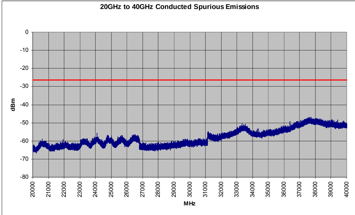
Plot 6-54. Conducted Spurious Plot (802.11a – Ch. 149)
