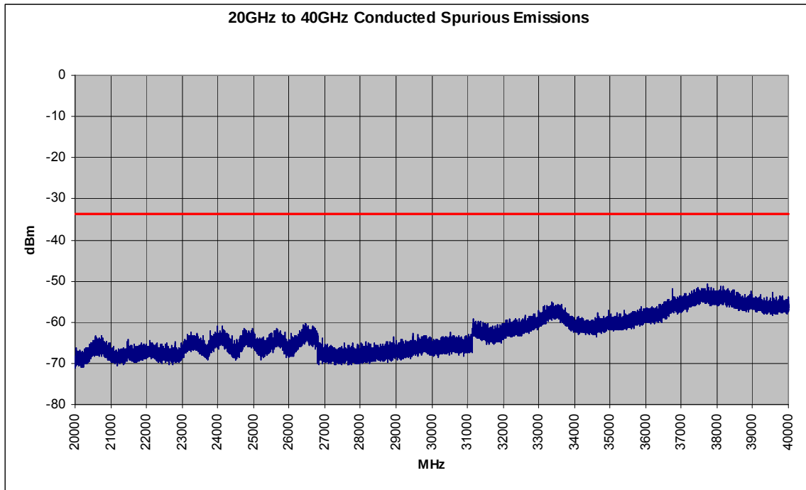
Plot 6-56. Conducted Spurious Plot (802.11a – Ch. 157)
