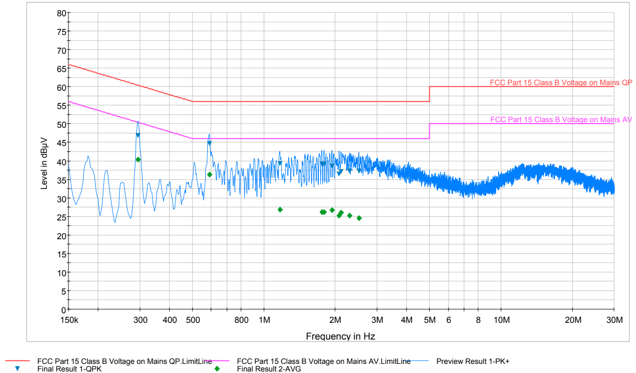
Plot 6-60. Line Conducted Plot with 802.11b (N)
