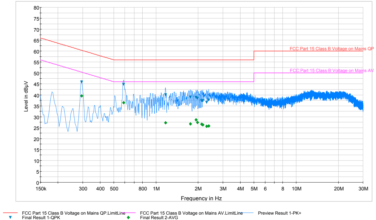
Plot 6-62. Line Conducted Plot with 802.11a (N)
