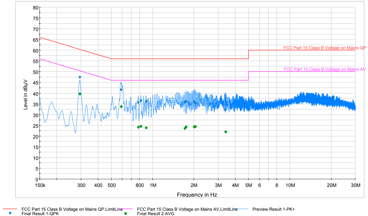
Plot 6-61. Line Conducted Plot with 802.11a (L1)
