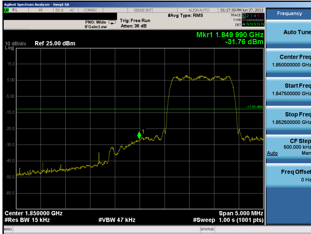
Plot 6-29. Band Edge Plot (PCS CDMA Mode – Ch. 25)
