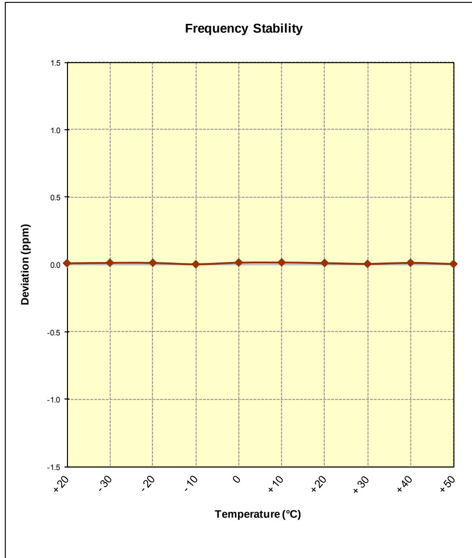
Figure 6-8. Frequency Stability Graph (PCS GSM Mode – Ch. 661)
