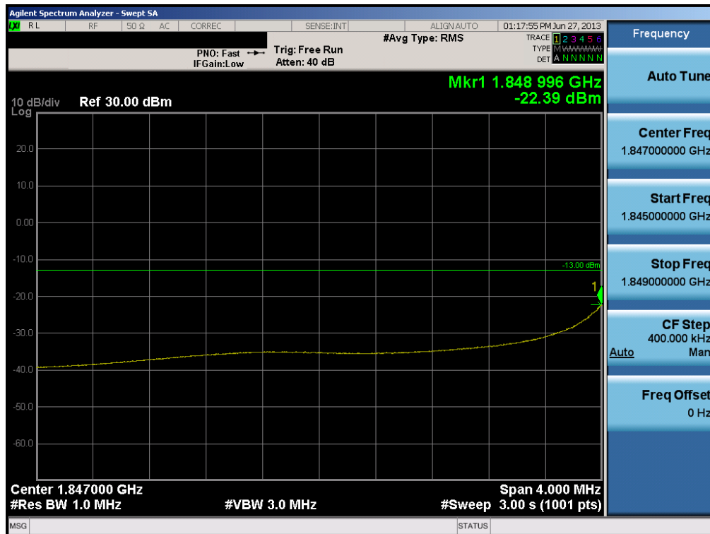
Plot 6-30. 4MHz Span Plot (PCS CDMA Mode – Ch. 25)
