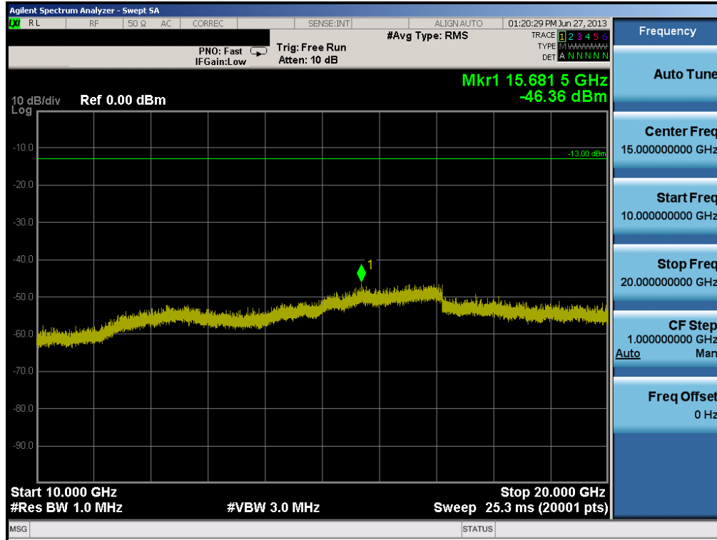
Plot 6-24. Conducted Spurious Plot (PCS CDMA Mode – Ch. 1175)
