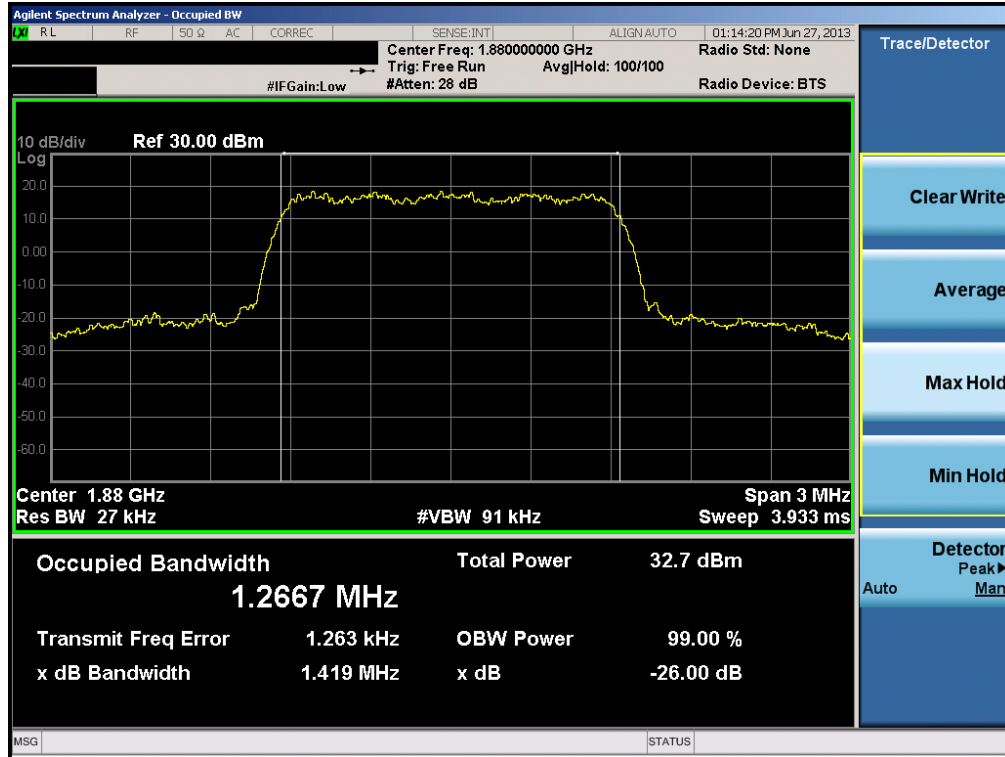
Plot 6-3. Occupied Bandwidth Plot (PCS CDMA Mode – Ch. 600)
