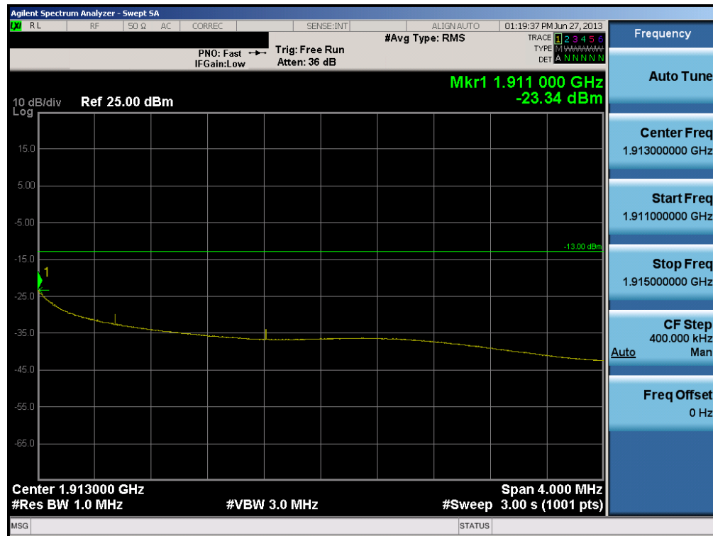
Plot 6-32. 4MHz Span Plot (PCS CDMA Mode – Ch. 1175)
