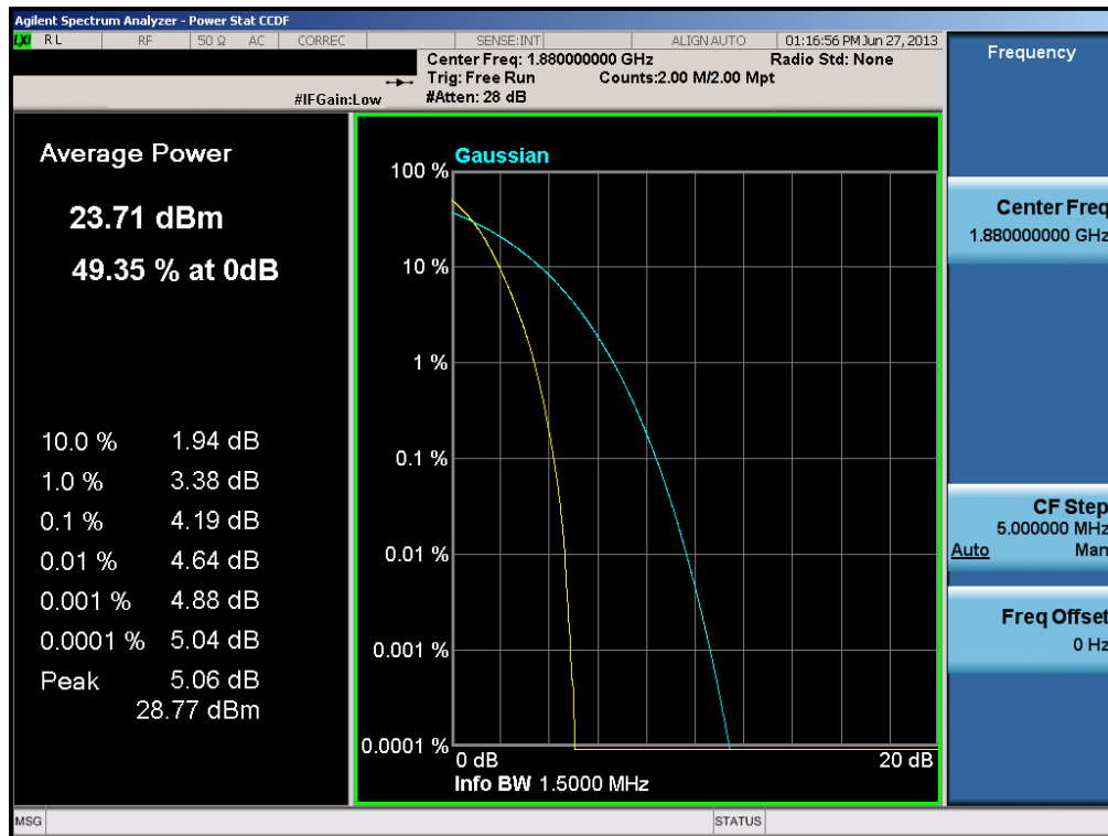
Plot 6-34. Peak-Average Ratio Plot (PCS CDMA Mode – Ch. 600)
