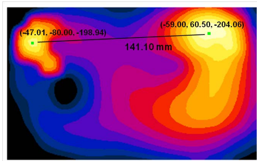
Figure 11-12 Peak SAR Location Plot of GSM1900 and 5 GHz WLAN
