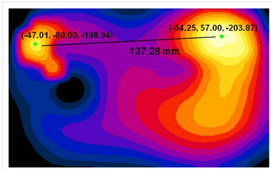
Figure 11-10 Peak SAR Location Plot of GPRS1900 and 5 GHz WLAN
