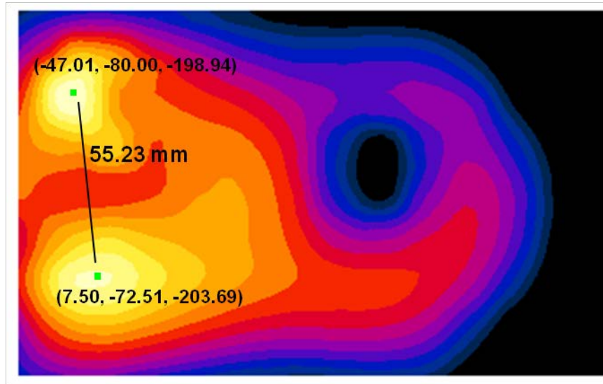
Figure 11-9 Peak SAR Location Plot of PCS CDMA and 5 GHz WLAN
