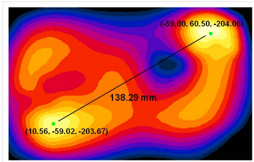
Figure 11-4 Peak SAR Location Plot of PCS EVDO and GSM1900
