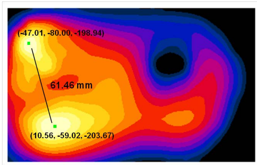
Figure 11-11 Peak SAR Location Plot of PCS EVDO and 5 GHz WLAN
