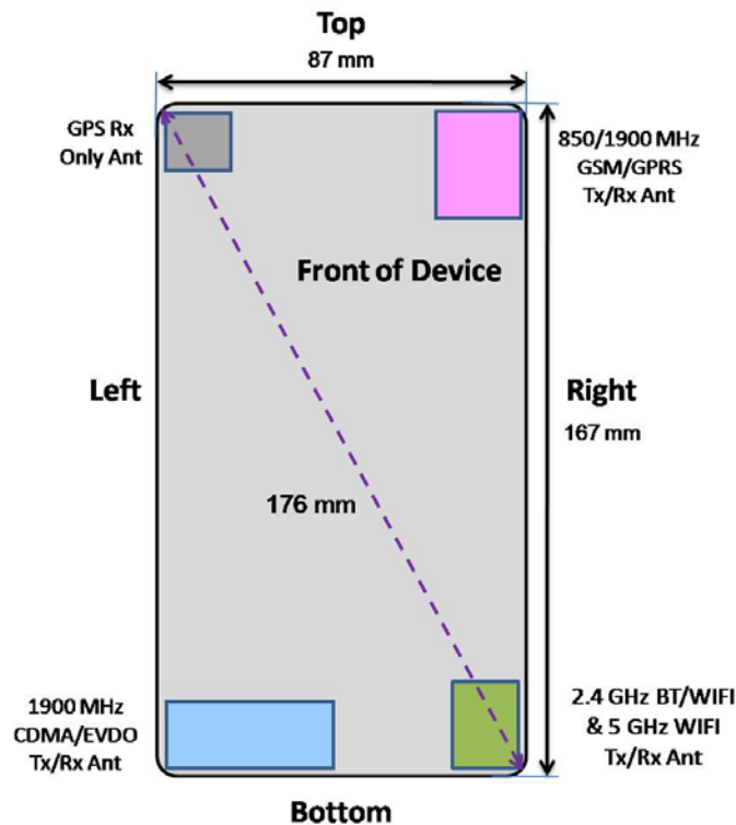
Figure 1-1 DUT Antenna Locations
