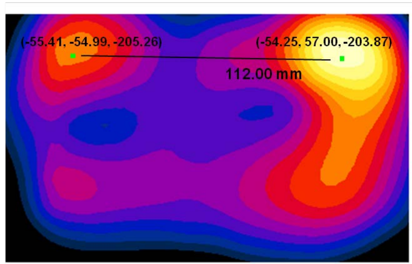
Figure 11-3 Peak SAR Location Plot of GPRS1900 and 2.4 GHz WLAN
