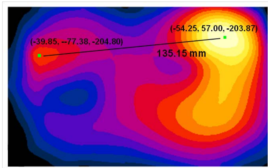
Figure 11-8 Peak SAR Location Plot of GPRS1900 and 2.4 GHz Bluetooth
