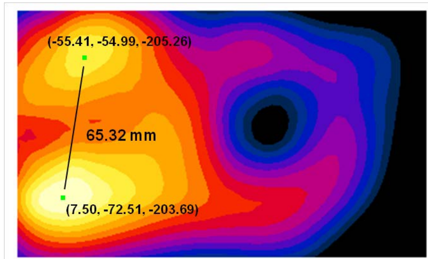
Figure 11-2 Peak SAR Location Plot of PCS CDMA and 2.4 GHz WLAN
