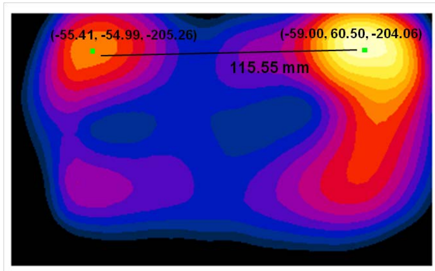
Figure 11-6 Peak SAR Location Plot of GSM1900 and 2.4 GHz WLAN
