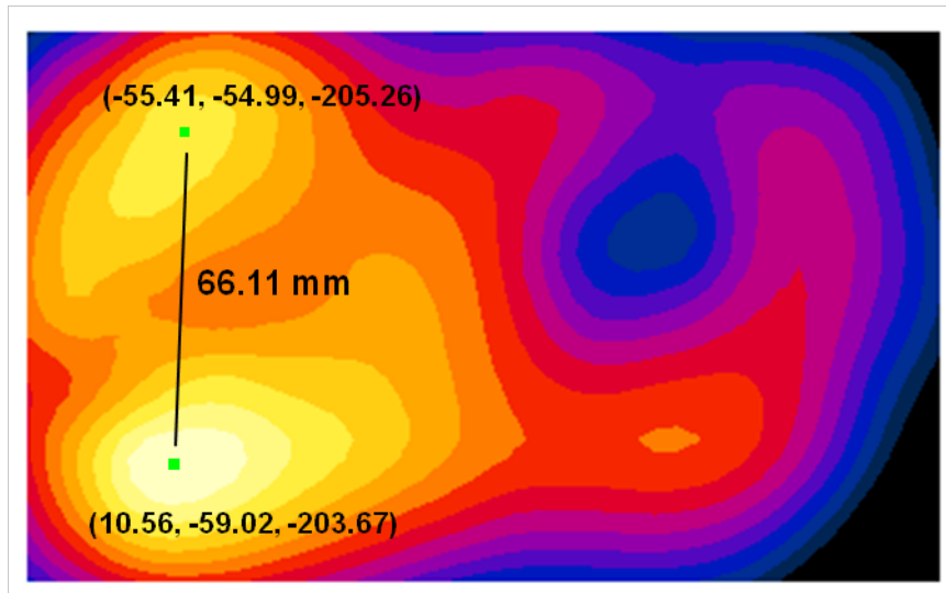
Figure 11-5 Peak SAR Location Plot of PCS EVDO and 2.4 GHz WLAN
