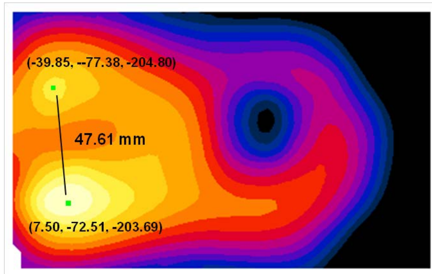
Figure 11-7 Peak SAR Location Plot of PCS CDMA and 2.4 GHz Bluetooth
