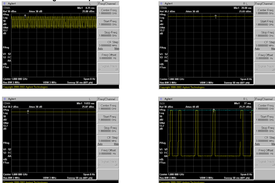
Figure 8-4 Zero-Span Plots
