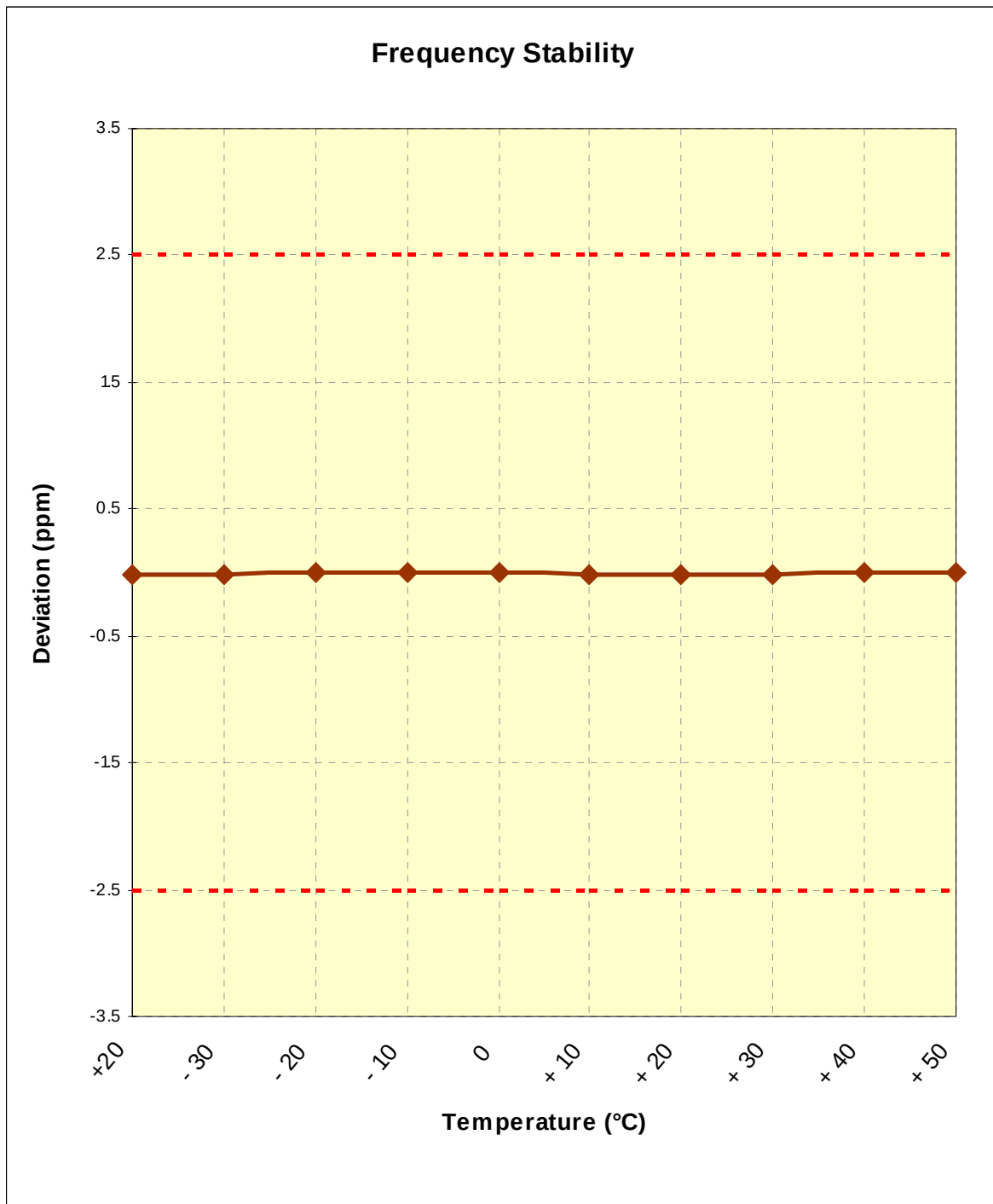
Figure 6-2. Frequency Stability Graph (AWS CDMA Mode – Ch. 450)
