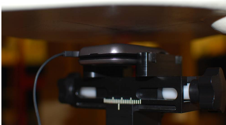
Figure 19-6 SAR Test Setup Photo 6 – Body Back
