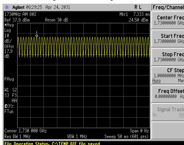
Figure 8.5 AM 80% Signal
