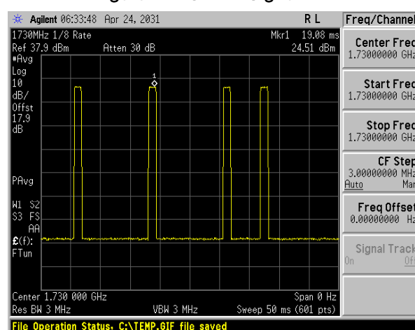
Figure 8.6 1/8 rate Signal
