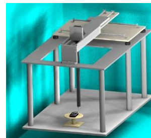
Figure 4-3 RF Near-Field Scanner
