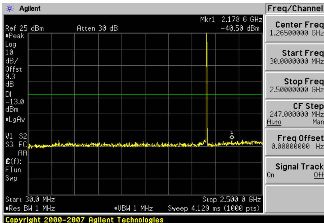
Plot 7-20. Conducted Spurious Plot (PCS CDMA Mode – Ch. 1275)
