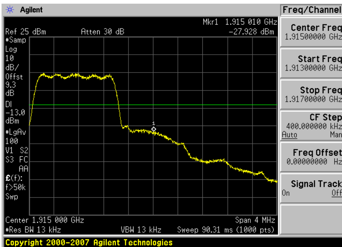
Plot 7-22. Band Edge Plot (PCS CDMA Mode – Ch. 1275)
