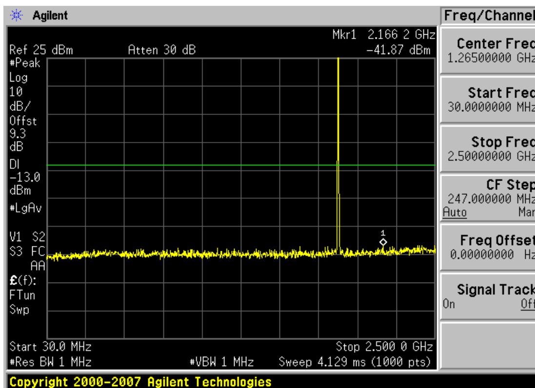
Plot 7-16. Conducted Spurious Plot (PCS CDMA Mode – Ch. 650)
