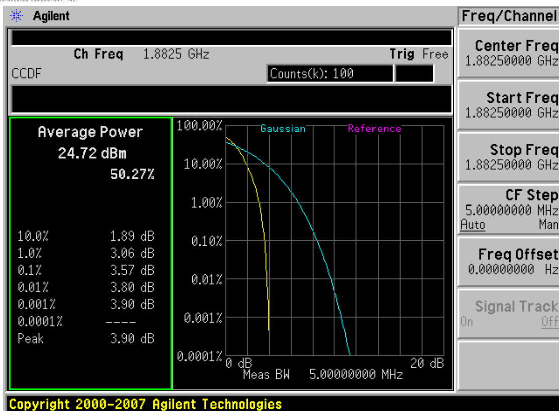
Plot 7-19. Peak-Average Ratio Plot (PCS CDMA Mode – Ch. 650)
