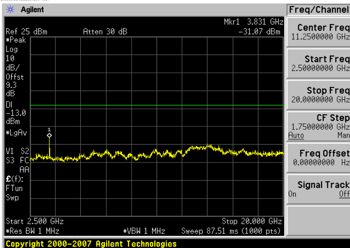
Plot 7-21. Conducted Spurious Plot (PCS CDMA Mode – Ch. 1275)
