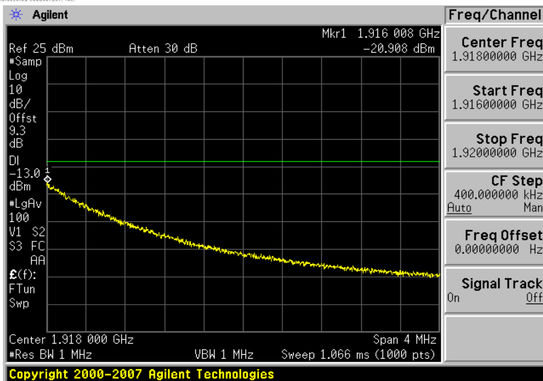
Plot 7-23. 4MHz Span Plot (PCS CDMA Mode – Ch. 1275)
