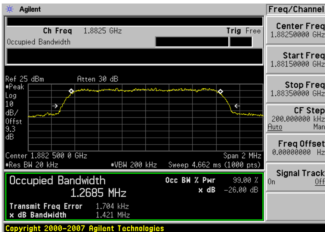
Plot 7-18. Occupied Bandwidth Plot (PCS CDMA Mode – Ch. 650)
