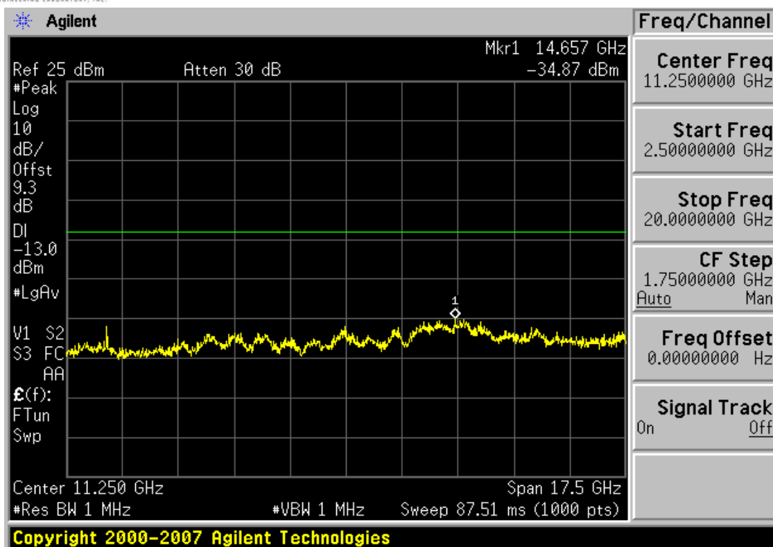
Plot 7-17. Conducted Spurious Plot (PCS CDMA Mode – Ch. 650)
