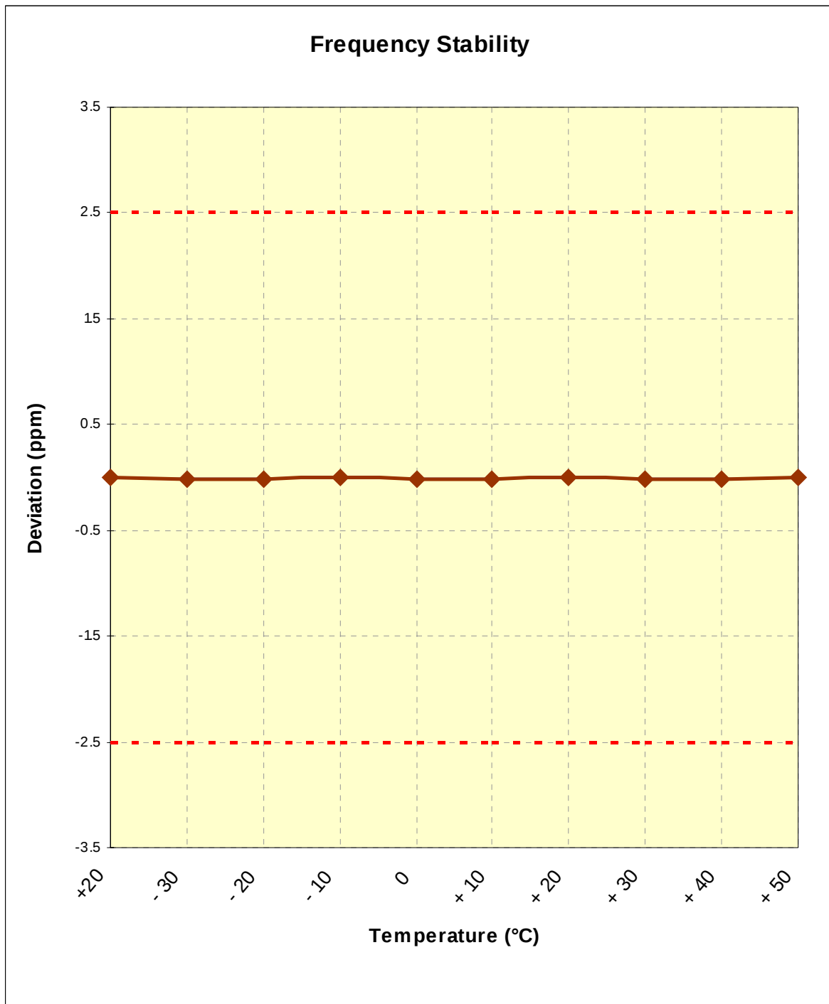
Figure 6-2. Frequency Stability Graph (PCS CDMA Mode – Ch. 650)
