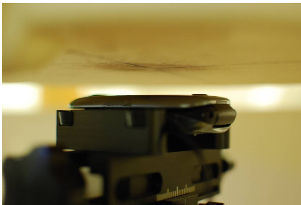
Figure 19-6 SAR Test Setup Photo 6
