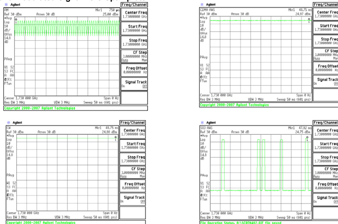
Figure 8-4 Zero-Span Plots
