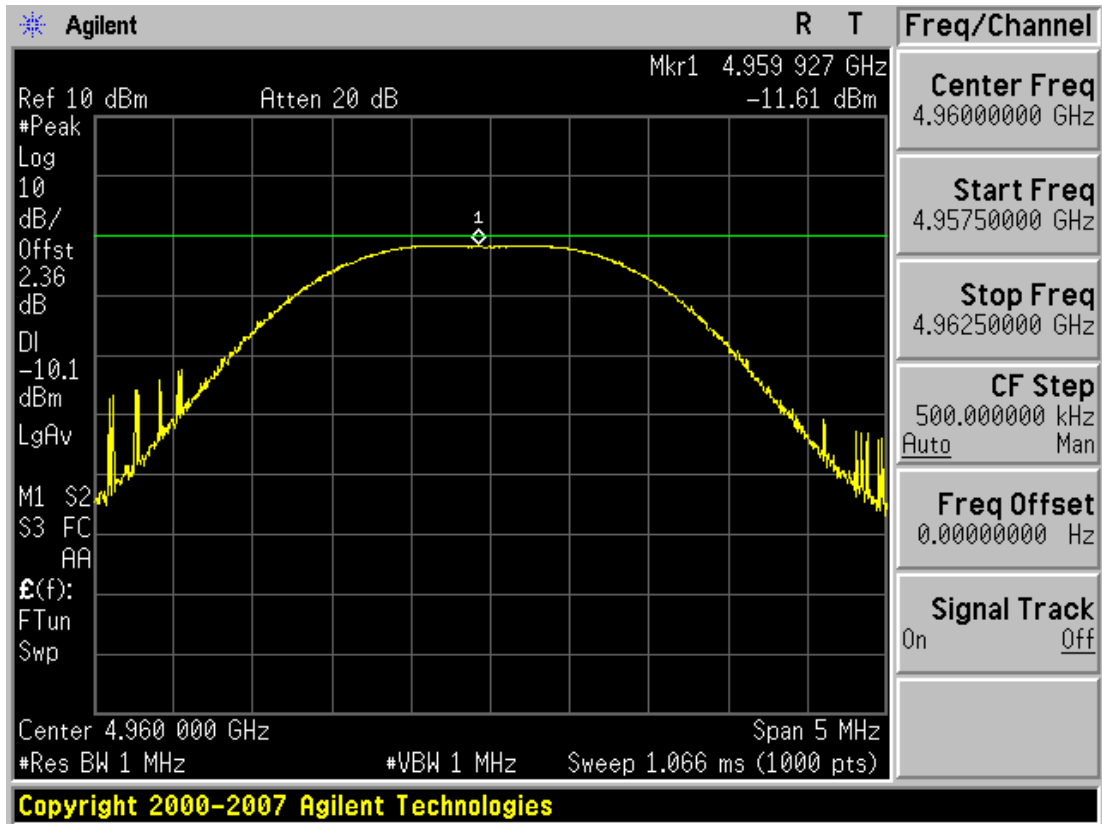
Plot 6-20. Supplemental Conducted Spurious Plot (Bluetooth – Ch. 78)
