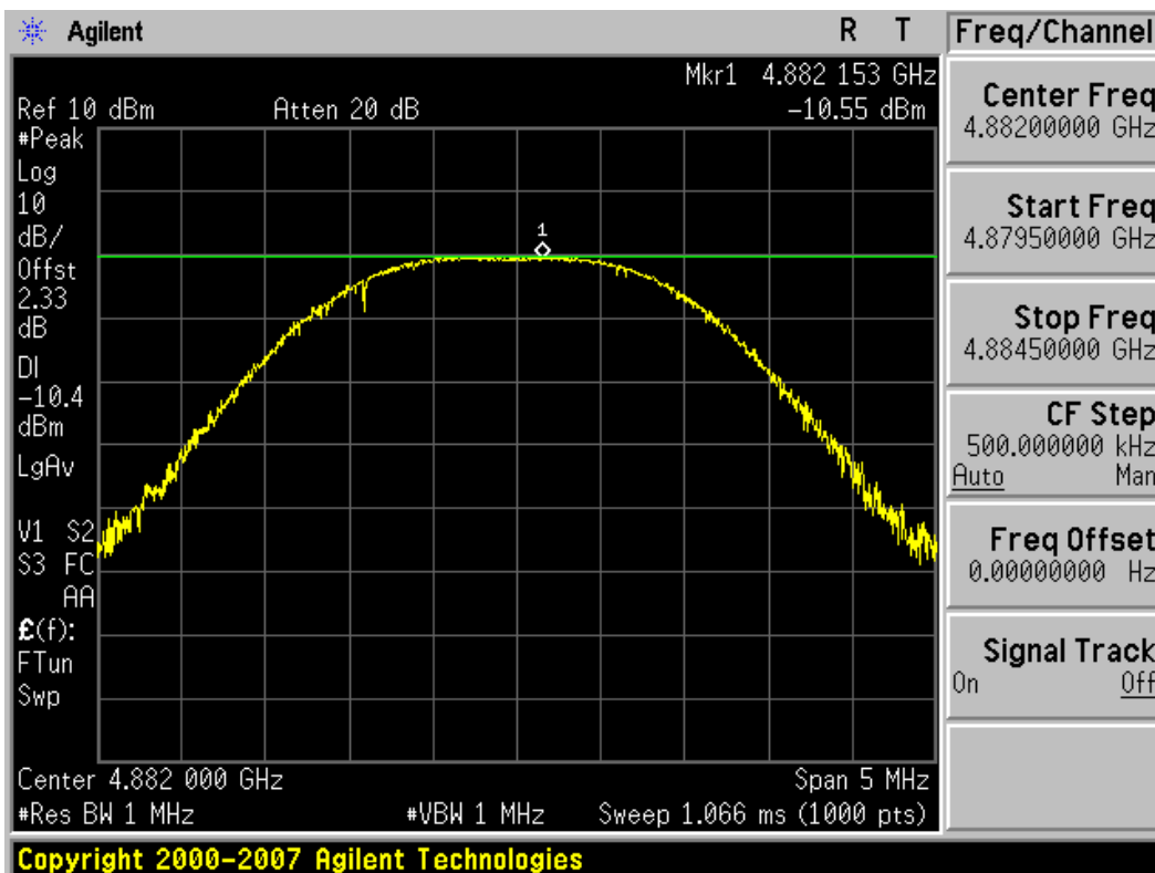
Plot 6-19. Supplemental Conducted Spurious Plot (Bluetooth – Ch. 39)
