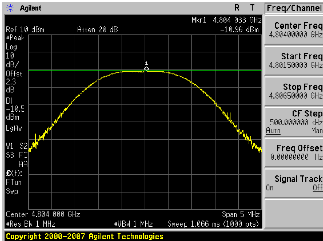
Plot 6-18. Supplemental Conducted Spurious Plot (Bluetooth – Ch. 0)
