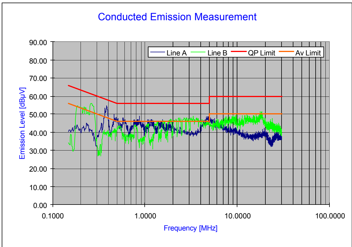
Plot 6-21. Line Conducted Plot with Bluetooth
