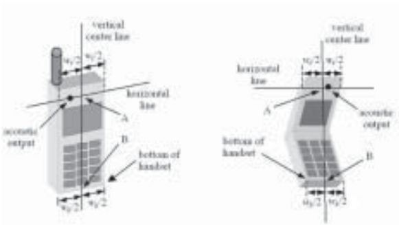
Figure 5.4 Handset vertical and horizontal reference lines
