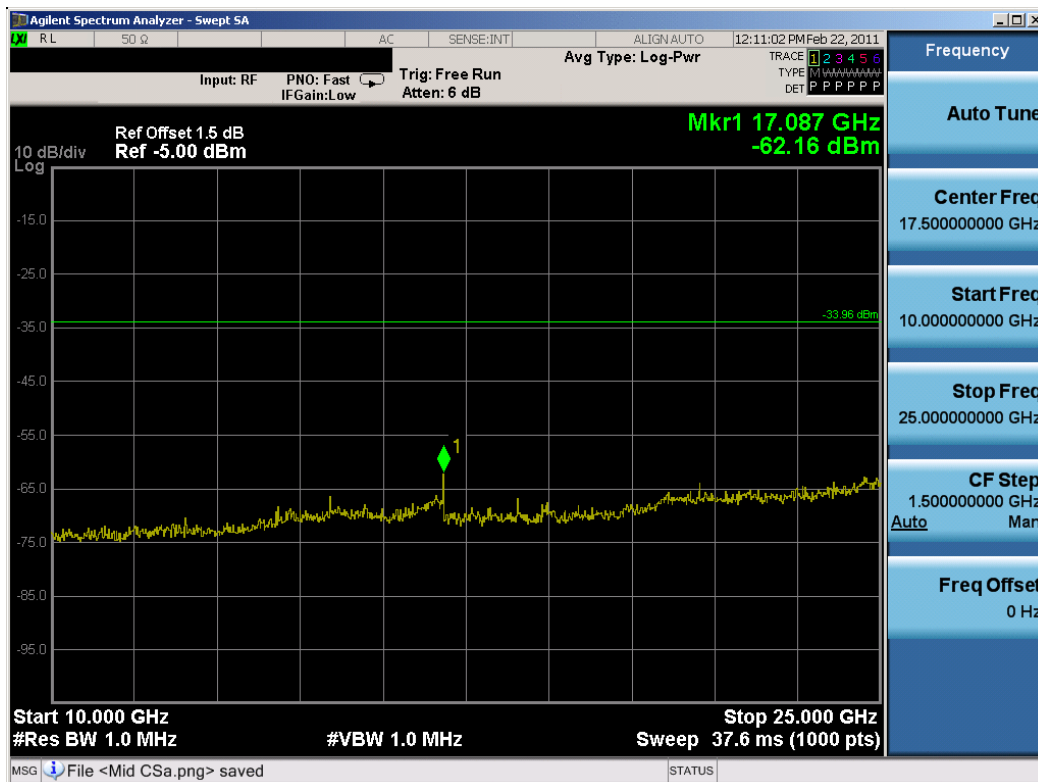
Plot 6-21. Conducted Spurious Plot (Bluetooth, 1Mbps – Ch. 39)
