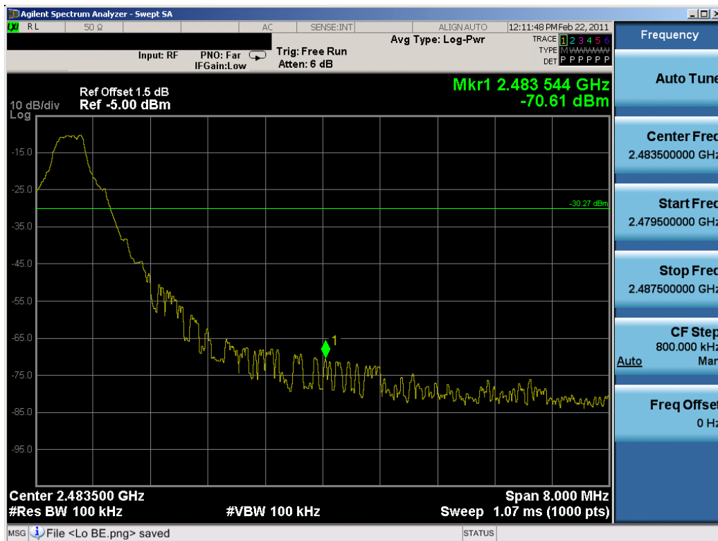
Plot 6-11. Band Edge Plot (Bluetooth, 1Mbps – Ch. 78)
