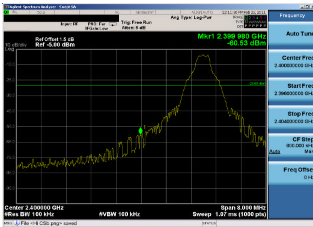
Plot 6-10. Band Edge Plot (Bluetooth, 1Mbps – Ch. 0)
