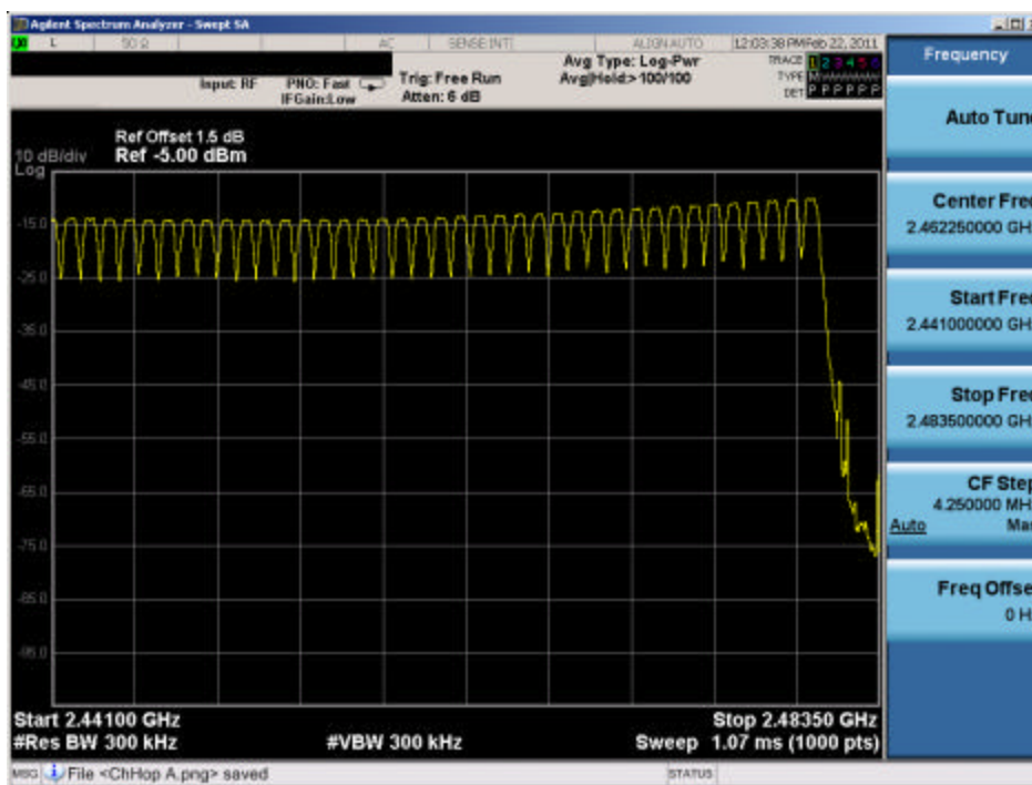
Plot 6-17. High End Spectrum Channel Hopping Plot (Bluetooth)
