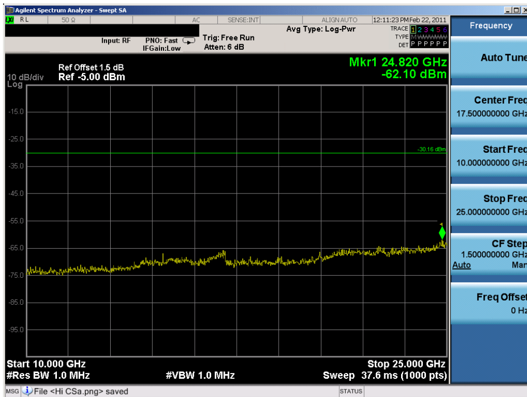
Plot 6-23. Conducted Spurious Plot (Bluetooth, 1Mbps – Ch. 78)
