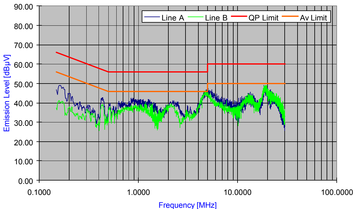
Plot 6-24. Line Conducted Plot with Bluetooth
