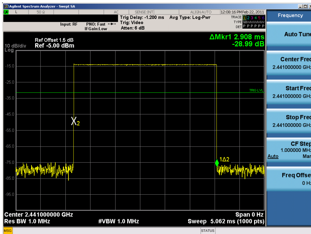
Plot 6-15. Time of Occupancy Plot (Bluetooth)
