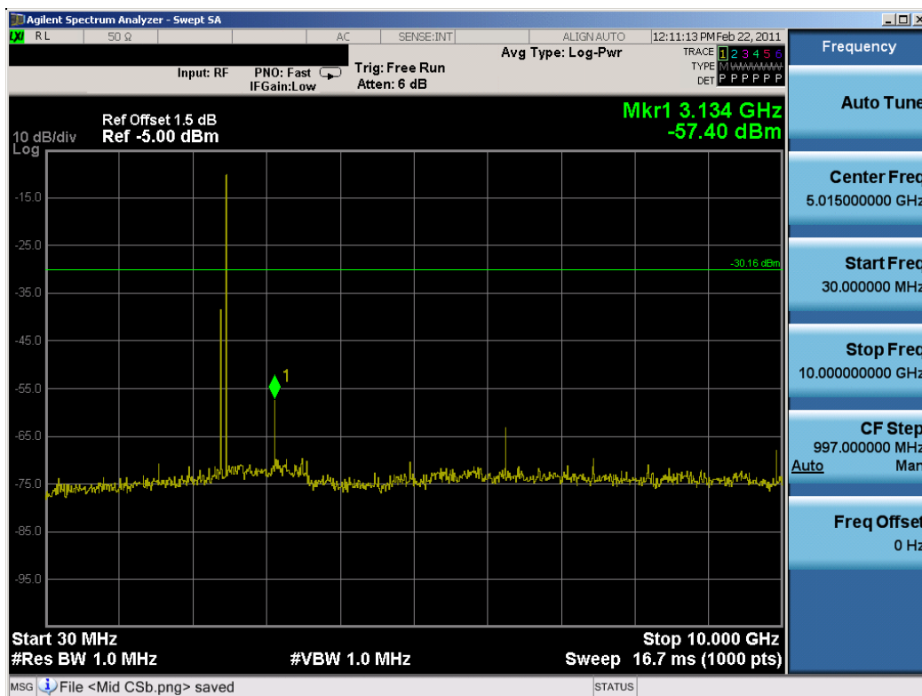
Plot 6-22. Conducted Spurious Plot (Bluetooth, 1Mbps – Ch. 78)
