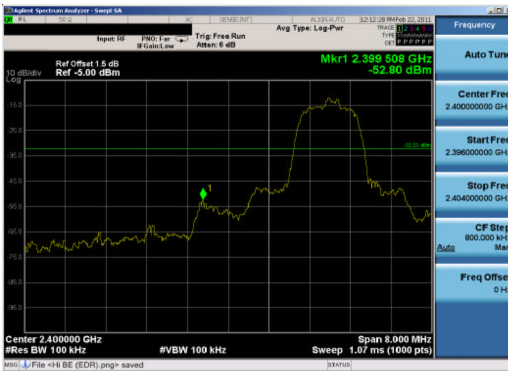
Plot 6-12. Band Edge Plot (Bluetooth, 3Mbps – Ch. 0)
