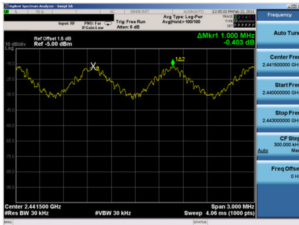
Plot 6-14. Channel Spacing Plot (Bluetooth)
