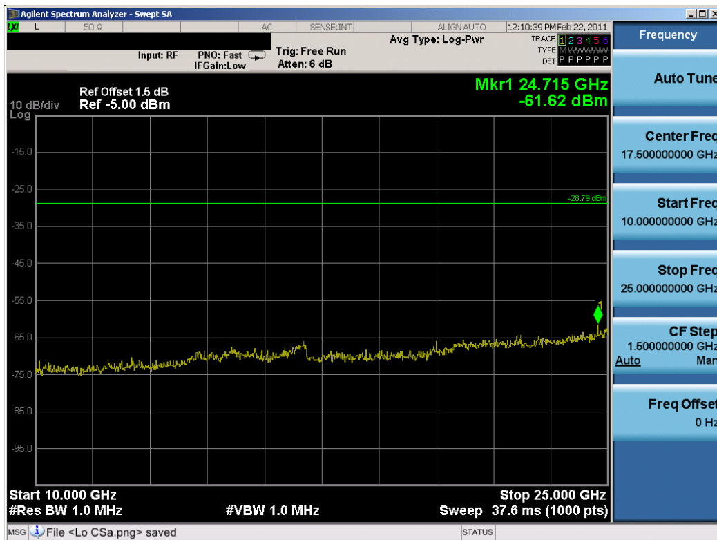
Plot 6-19. Conducted Spurious Plot (Bluetooth, 1Mbps – Ch. 0)
