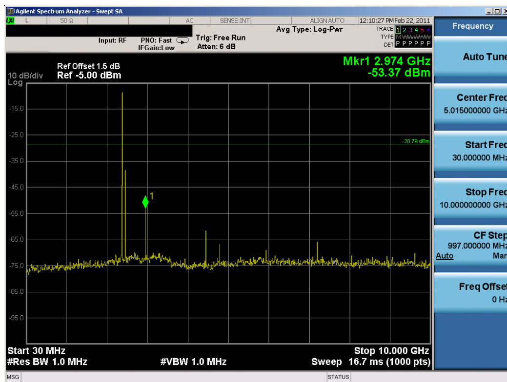
Plot 6-18. Conducted Spurious Plot (Bluetooth, 1Mbps – Ch. 0)
