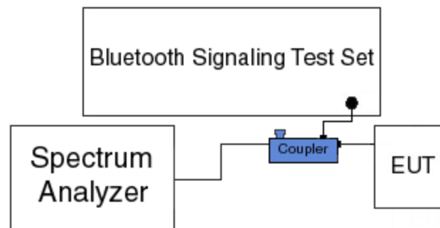
Figure 6-2. Test Instrument & Measurement Setup
