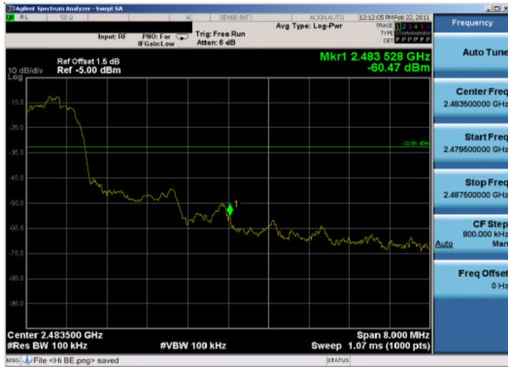
Plot 6-13. Band Edge Plot (Bluetooth, 3Mbps – Ch. 78)
