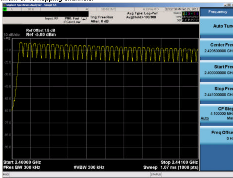
Plot 6-16. Low End Spectrum Channel Hopping Plot (Bluetooth)
