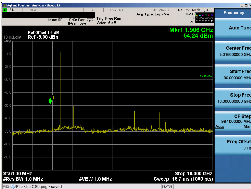
Plot 6-20. Conducted Spurious Plot (Bluetooth, 1Mbps – Ch. 39)
