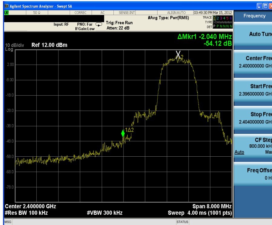
Plot 6-10. Band Edge Plot (Bluetooth with Hopping Disabled, 2Mbps – Ch. 0)
