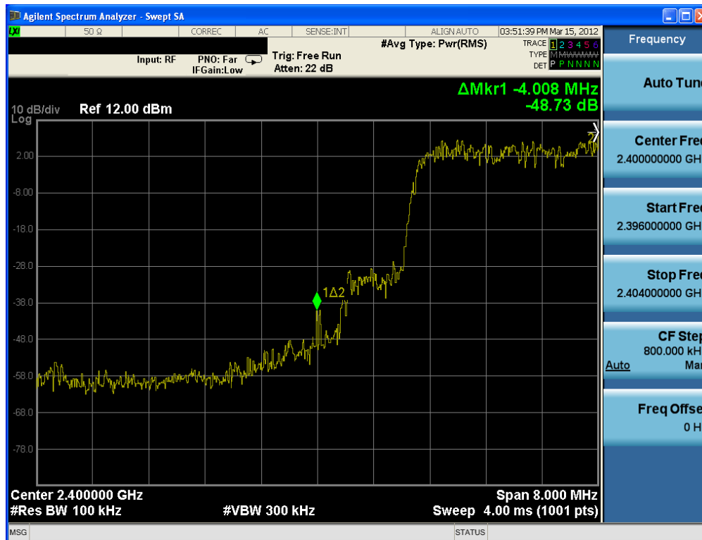
Plot 6-12. Band Edge Plot (Bluetooth with Hopping Enabled, 2Mbps – Ch. 0)
