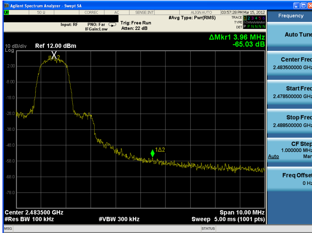
Plot 6-11. Band Edge Plot (Bluetooth with Hopping Disabled, 2Mbps – Ch. 78)
