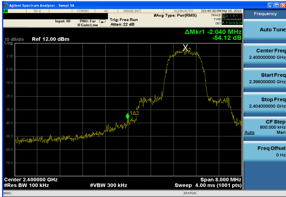
Plot 6-10. Band Edge Plot (Bluetooth with Hopping Disabled, 2Mbps – Ch. 0)
