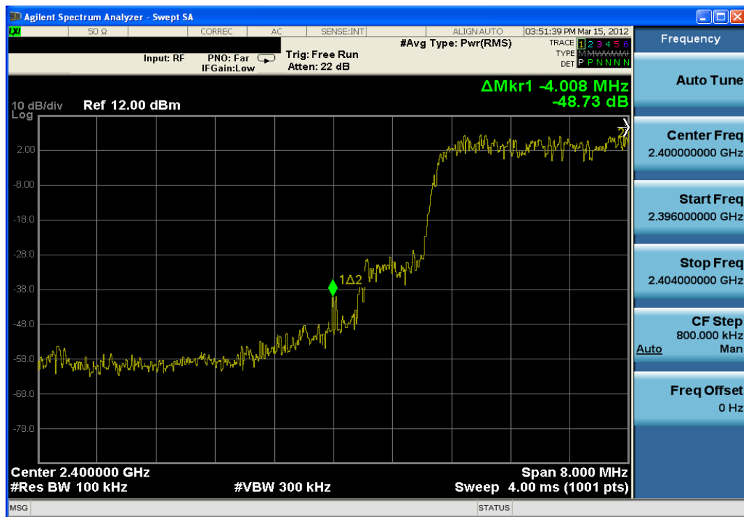
Plot 6-12. Band Edge Plot (Bluetooth with Hopping Enabled, 2Mbps – Ch. 0)
