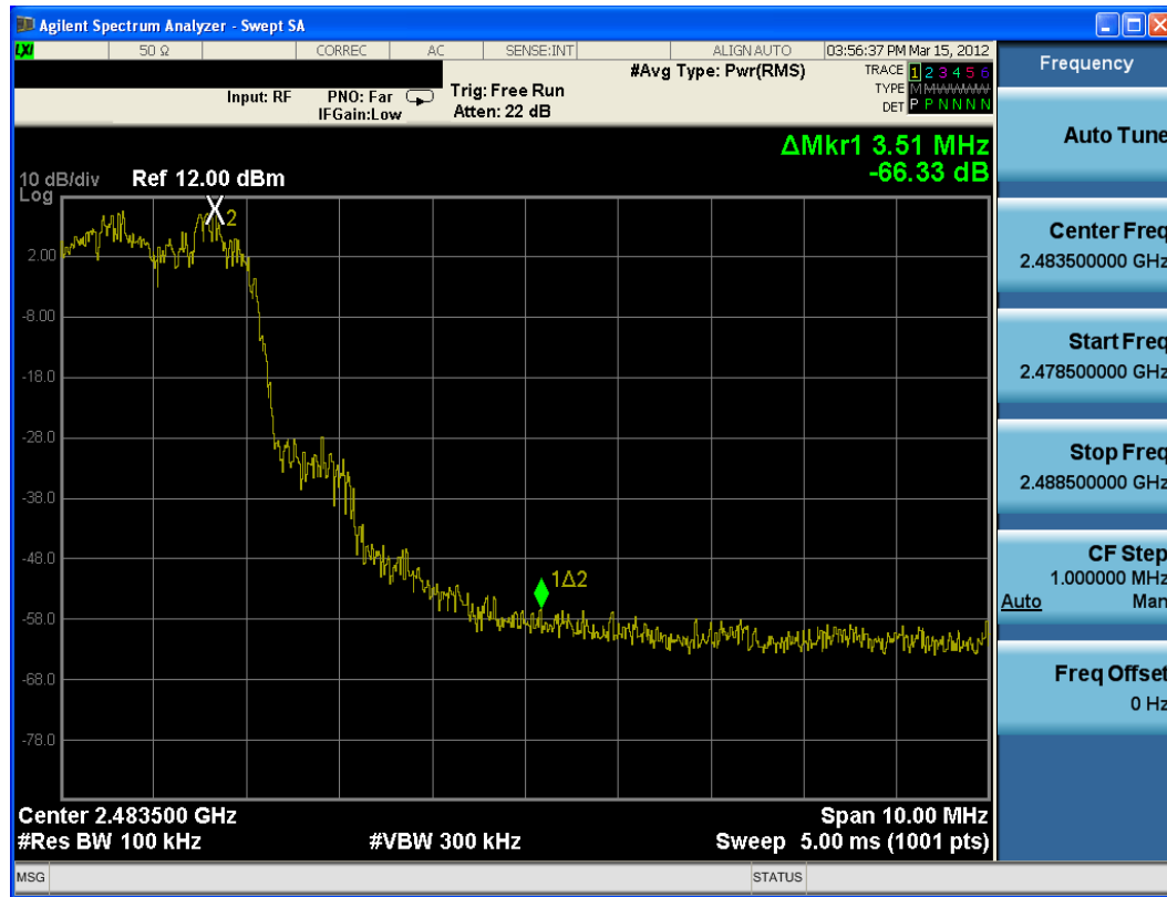
Plot 6-13. Band Edge Plot (Bluetooth with Hopping Enabled, 2Mbps – Ch. 78)
