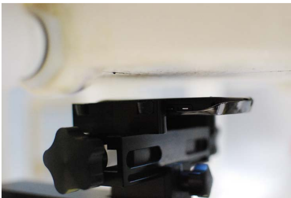
SAR Test Setup Photo 6 – Body-Worn Back Side at 1.5 cm
