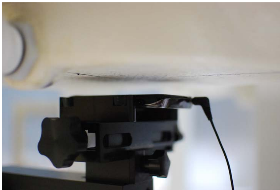
SAR Test Setup Photo 5 – Body-Worn Back Side at 1.5 cm
