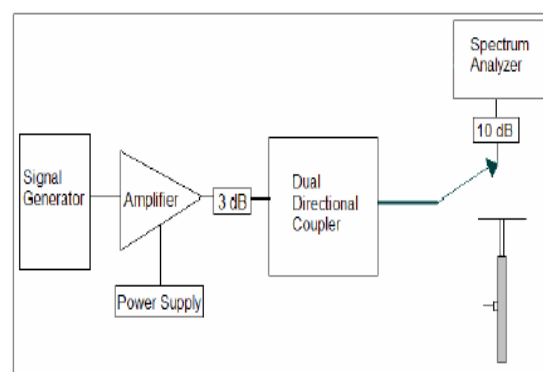
Figure 8.2 Setup to Peak Power using Spectrum Analyzer
